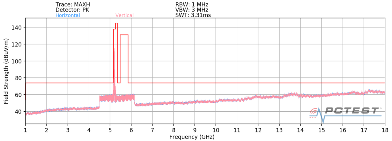
Plot 7-133. Radiated Spurious Plot above 1GHz (802.11a – U1 Ch. 40)
