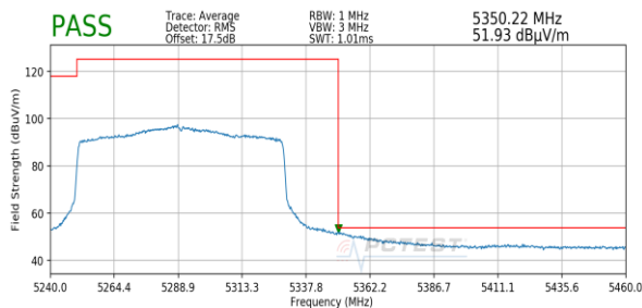
Plot 7-155. Radiated Upper Band Edge Plot (Average – UNII Band 2A)
