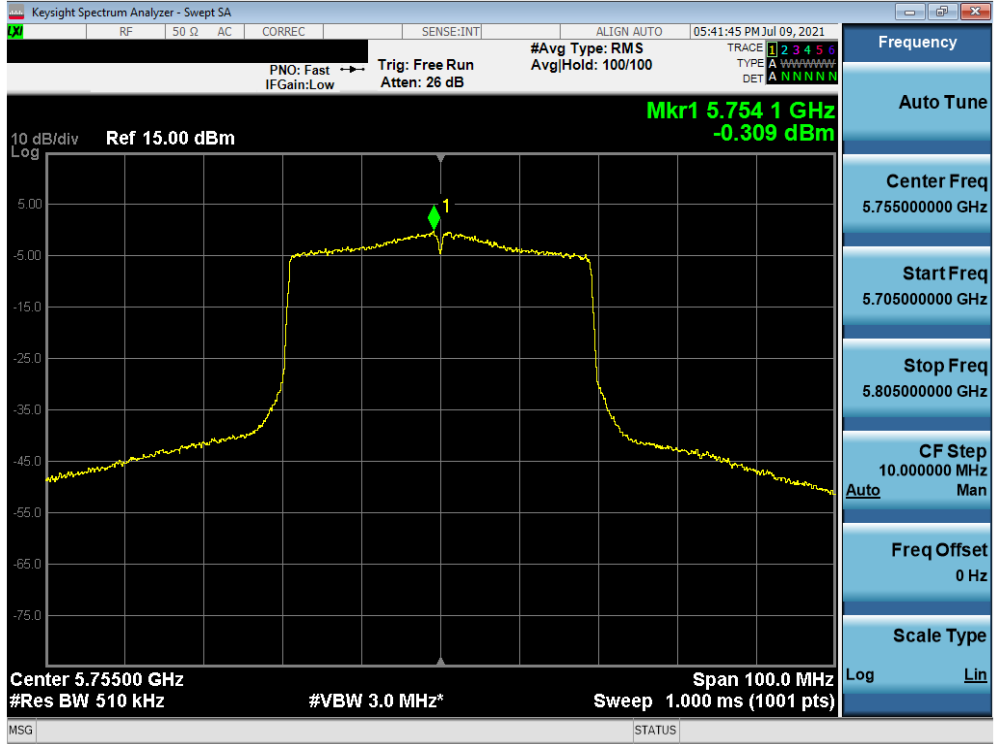
Plot 7-129. Power Spectral Density Plot (40MHz BW 802.11ax (UNII Band 3) – Ch. 151)
