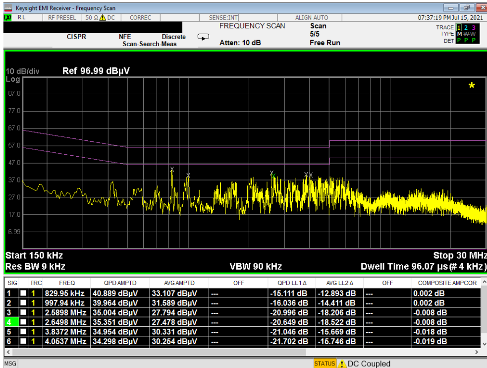
Plot 7-166. Line Conducted Plot with 802.11a UNII Band 2C (N)
