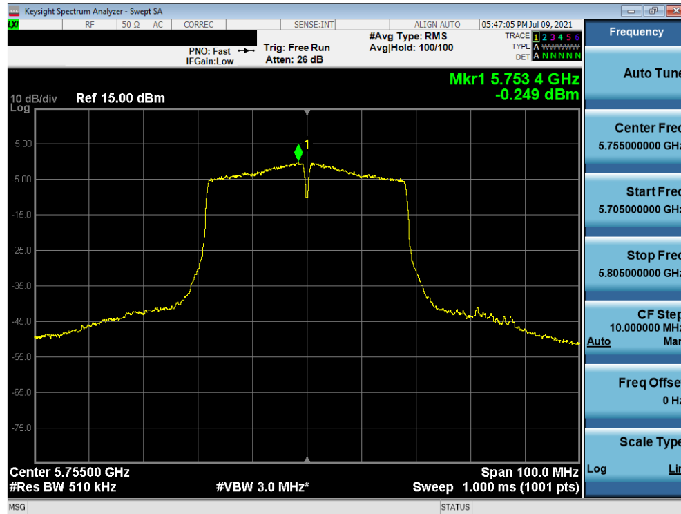
Plot 7-127. Power Spectral Density Plot (40MHz BW 802.11n (UNII Band 3) – Ch. 151)
