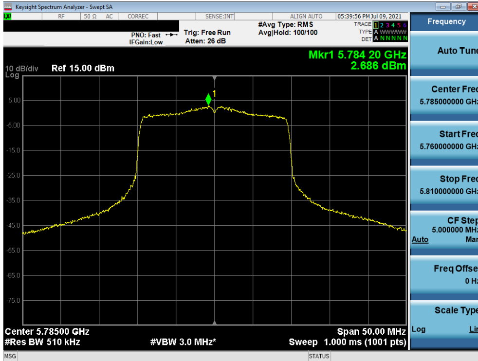
Plot 7-125. Power Spectral Density Plot (20MHz BW 802.11ax (UNII Band 3) – Ch. 157)
