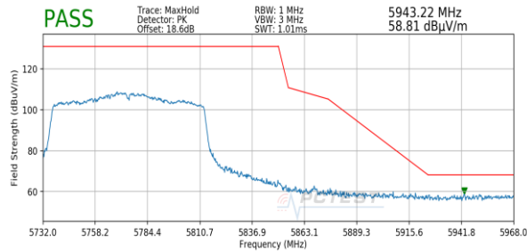
Plot 7-159. Radiated Upper Band Edge Plot (Peak – UNII Band 3)
