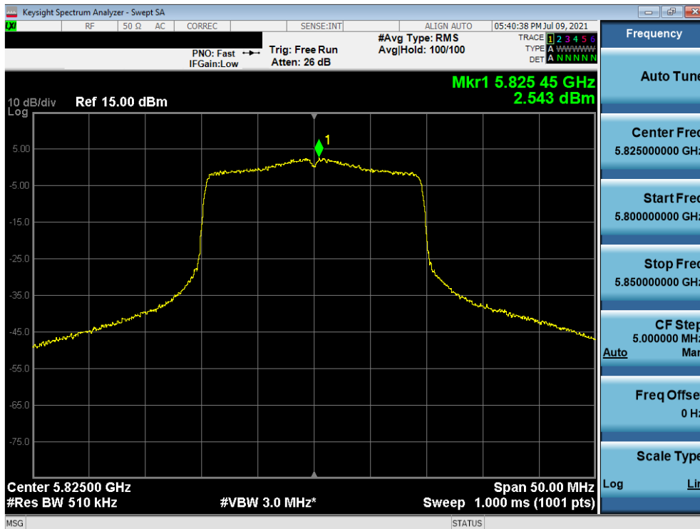
Plot 7-126. Power Spectral Density Plot (20MHz BW 802.11ax (UNII Band 3) – Ch. 165)
