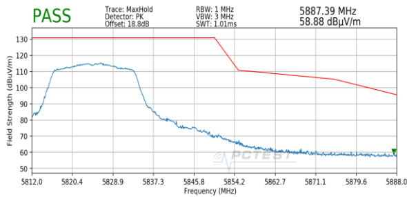
Plot 7-145. Radiated Upper Band Edge Plot (Peak – UNII Band 3)
