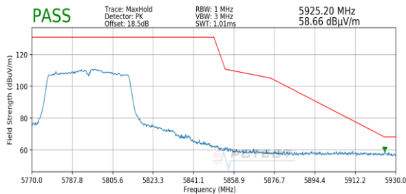
Plot 7-152. Radiated Upper Band Edge Plot (Peak – UNII Band 3)
