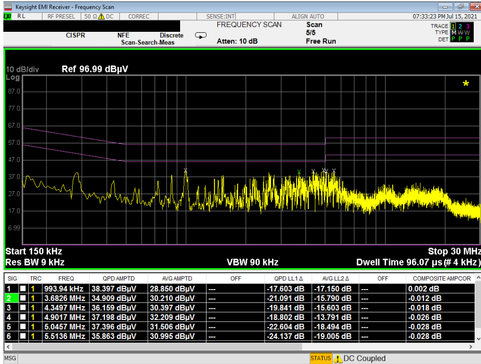
Plot 7-161. Line Conducted Plot with 802.11a UNII Band 1 (L1)
