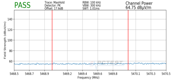
Plot 7-151. Radiated Lower Band Edge Plot (Peak – UNII Band 2C)
