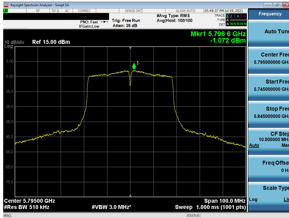
Plot 7-128. Power Spectral Density Plot (40MHz BW 802.11n (UNII Band 3) – Ch. 159)
