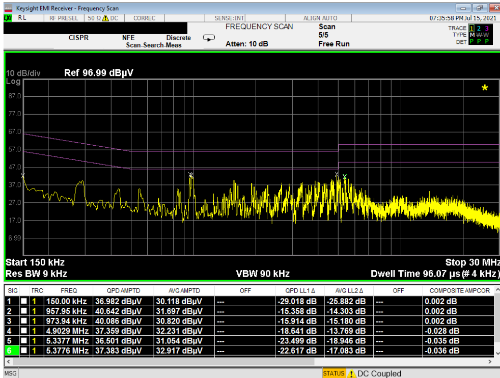
Plot 7-164. Line Conducted Plot with 802.11a UNII Band 2A (N)
