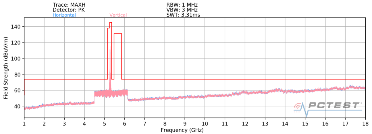
Plot 7-134. Radiated Spurious Plot above 1GHz (802.11a – U2A Ch. 56)
