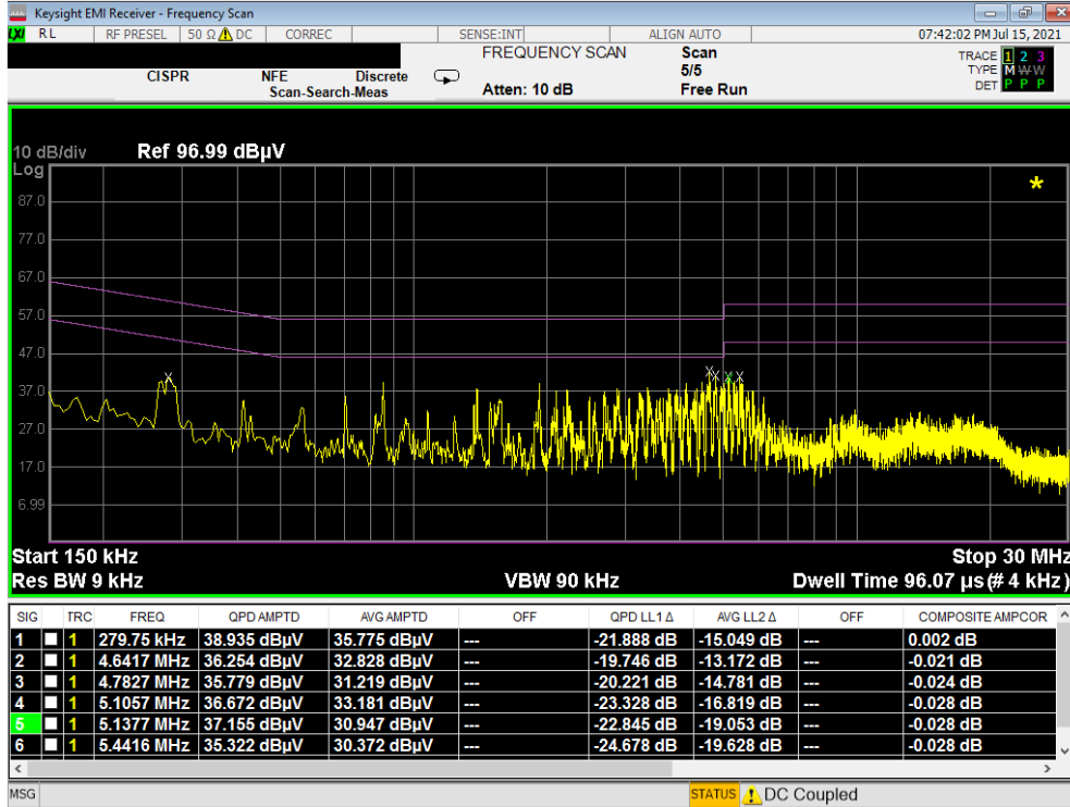
Plot 7-167. Line Conducted Plot with 802.11a UNII Band 3 (L1)
