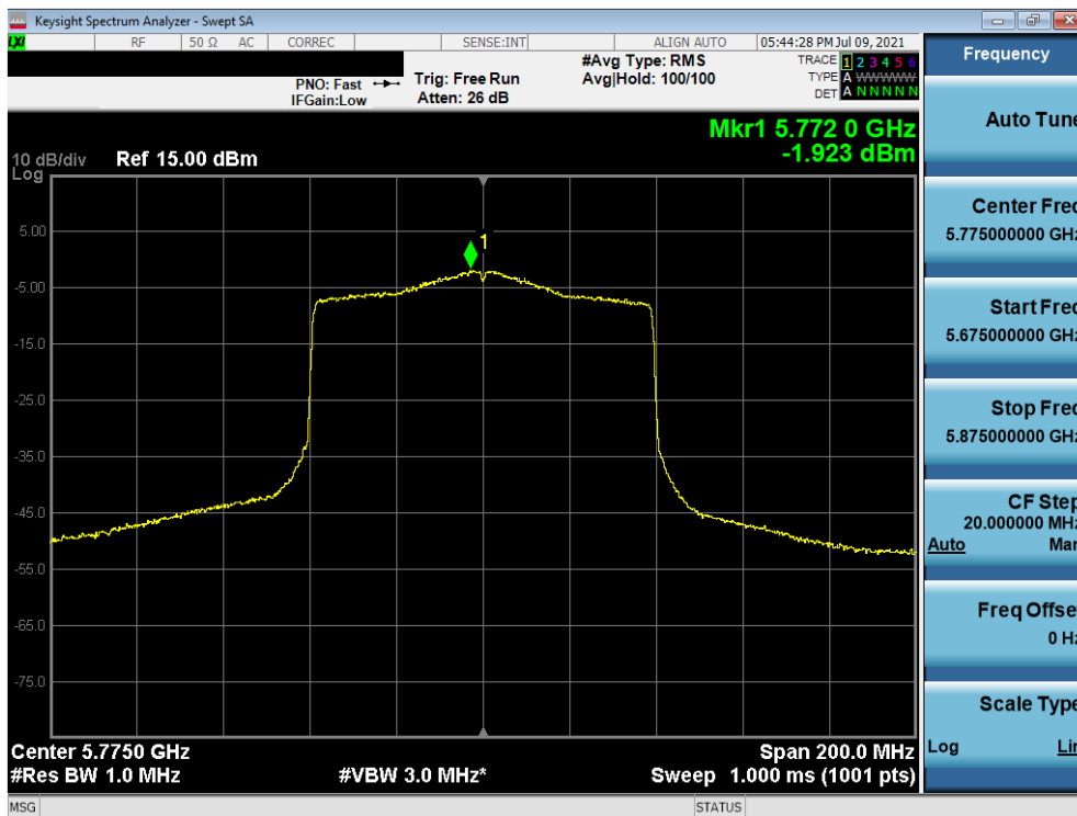
Plot 7-132. Power Spectral Density Plot (80MHz BW 802.11ax (UNII Band 3) – Ch. 155)
