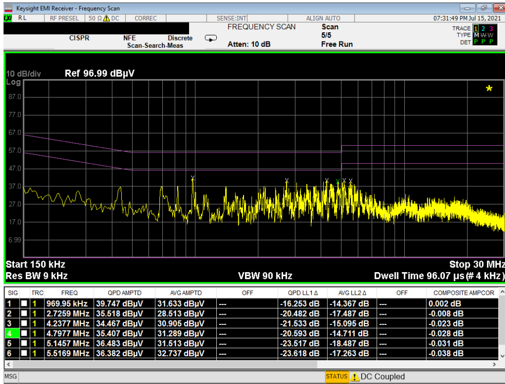
Plot 7-162. Line Conducted Plot with 802.11a UNII Band 1 (N)
