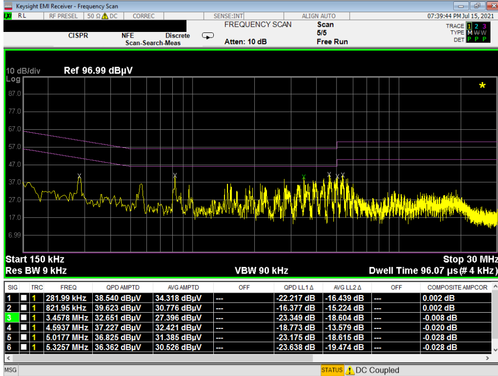
Plot 7-165. Line Conducted Plot with 802.11a UNII Band 2C (L1)
