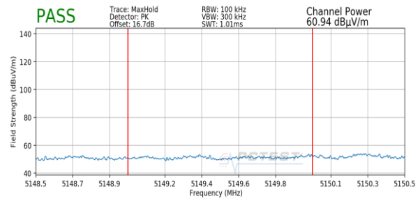
Plot 7-147. Radiated Lower Band Edge Plot (Peak – UNII Band 1)
