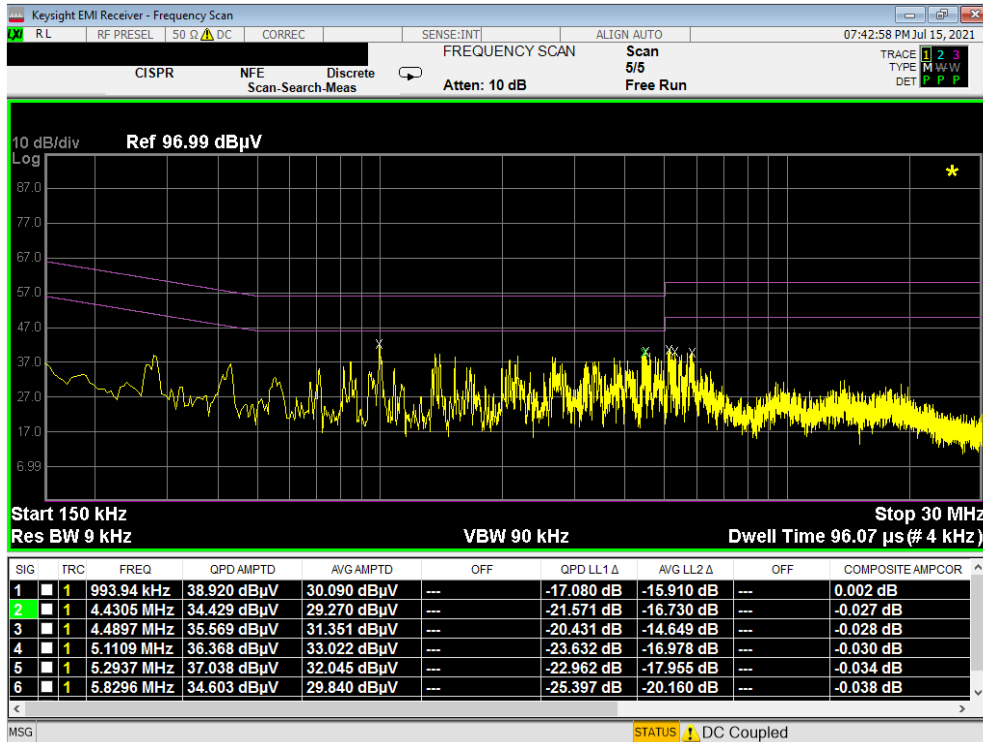
Plot 7-168. Line Conducted Plot with 802.11a UNII Band 3 (N)
