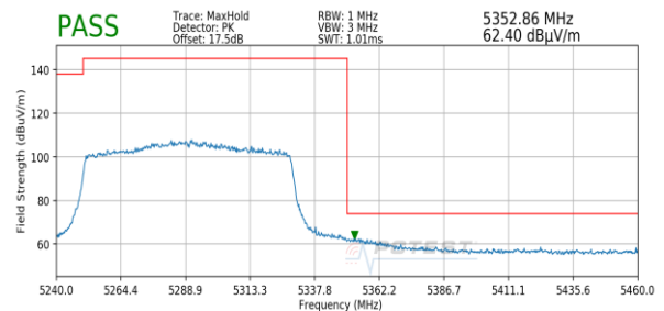
Plot 7-156. Radiated Upper Band Edge Plot (Peak – UNII Band 2A)
