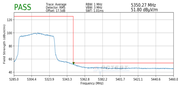
Plot 7-148. Radiated Upper Band Edge Plot (Average – UNII Band 2A)
