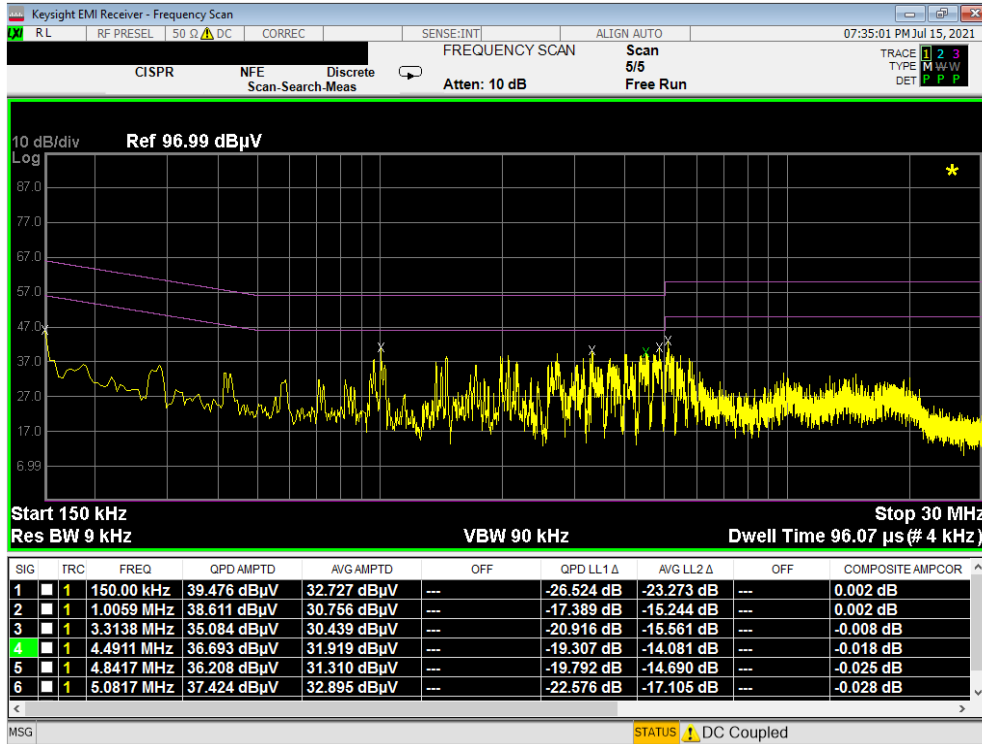
Plot 7-163. Line Conducted Plot with 802.11a UNII Band 2A (L1)
