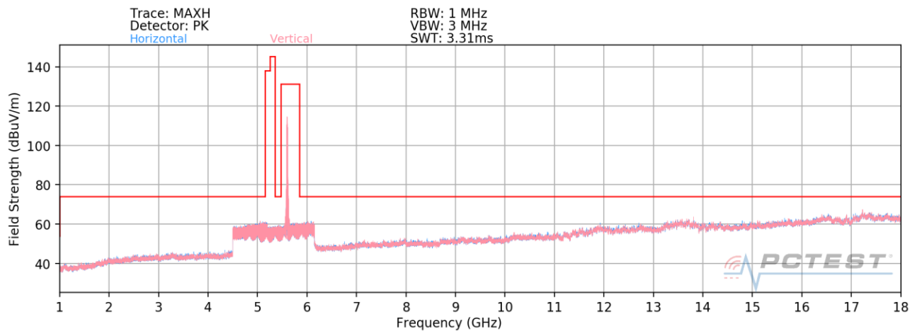
Plot 7-135. Radiated Spurious Plot above 1GHz (802.11a – U2C Ch. 120)
