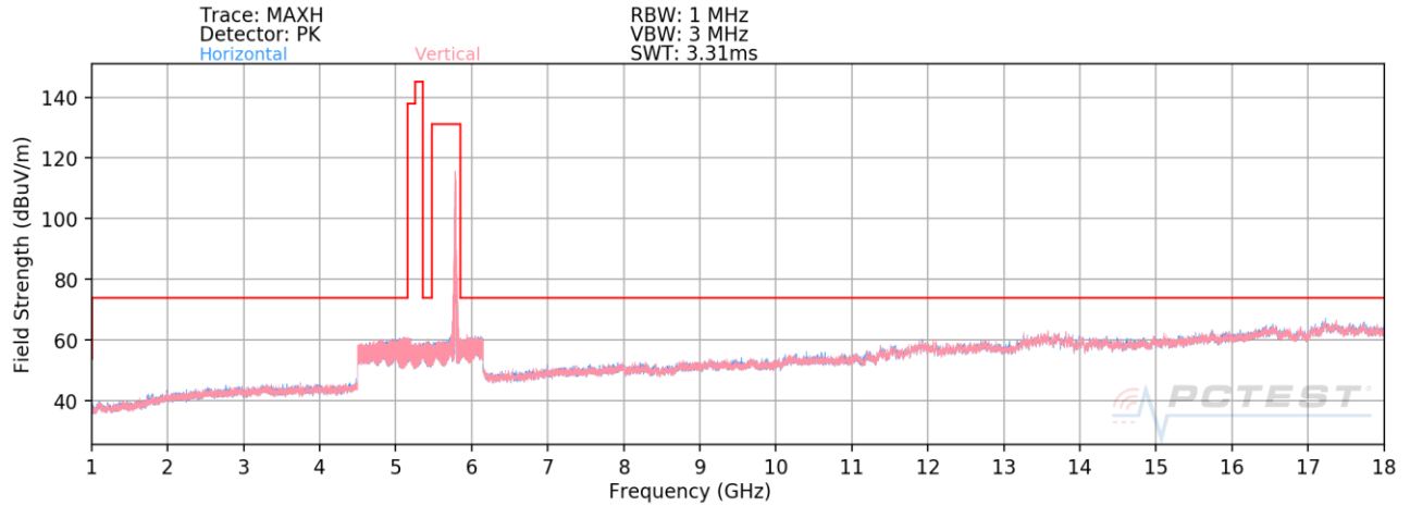
Plot 7-136. Radiated Spurious Plot above 1GHz (802.11a – U3 Ch. 157)
