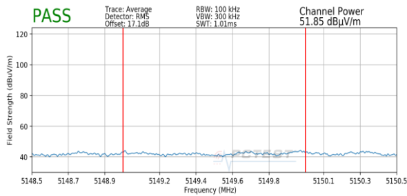
Plot 7-139. Radiated Lower Band Edge Plot (Average – UNII Band 1)
