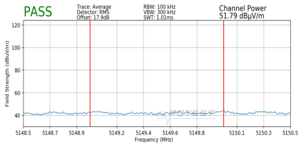
Plot 7-153. Radiated Lower Band Edge Plot (Average – UNII Band 1)
