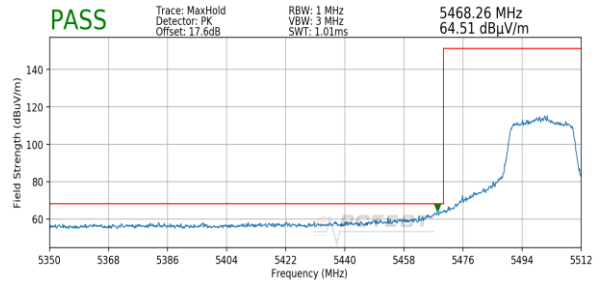
Plot 7-144. Radiated Lower Band Edge Plot (Peak – UNII Band 2C)
