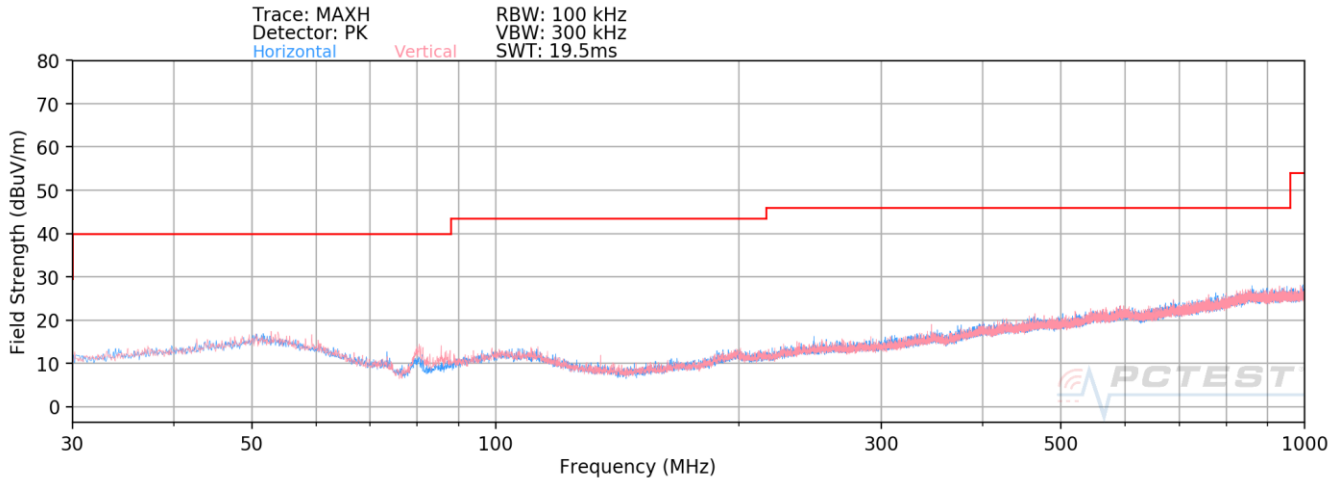
Plot 7-160. Radiated Spurious Plot below 1GHz (802.11a – U3 Ch. 157)
