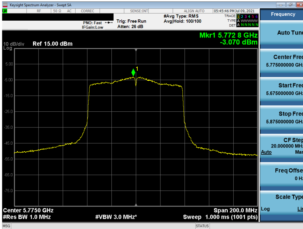
Plot 7-131. Power Spectral Density Plot (80MHz BW 802.11ac (UNII Band 3) – Ch. 155)
