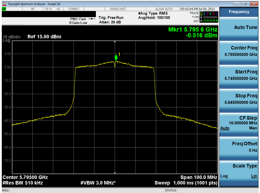
Plot 7-130. Power Spectral Density Plot (40MHz BW 802.11ax (UNII Band 3) – Ch. 159)
