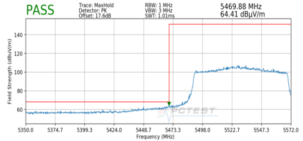
Plot 7-158. Radiated Lower Band Edge Plot (Peak – UNII Band 2C)
