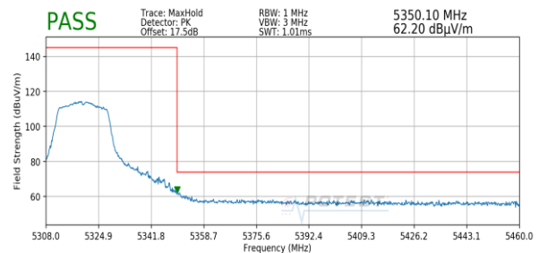
Plot 7-142. Radiated Upper Band Edge Plot (Peak – UNII Band 2A)
