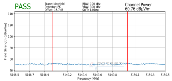
Plot 7-154. Radiated Lower Band Edge Plot (Peak – UNII Band 1)
