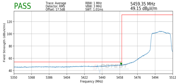
Plot 7-143. Radiated Lower Band Edge Plot (Average – UNII Band 2C)
