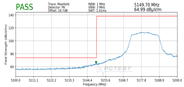
Plot 7-140. Radiated Lower Band Edge Plot (Peak – UNII Band 1)
