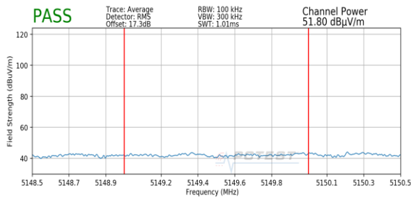
Plot 7-146. Radiated Lower Band Edge Plot (Average – UNII Band 1)
