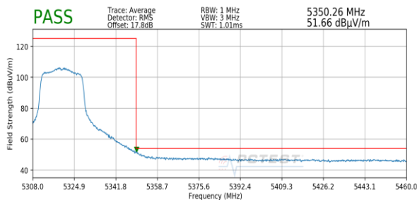
Plot 7-141. Radiated Upper Band Edge Plot (Average – UNII Band 2A)
