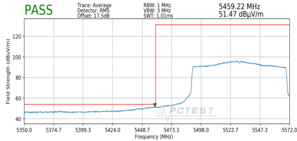
Plot 7-157. Radiated Lower Band Edge Plot (Average – UNII Band 2C)
