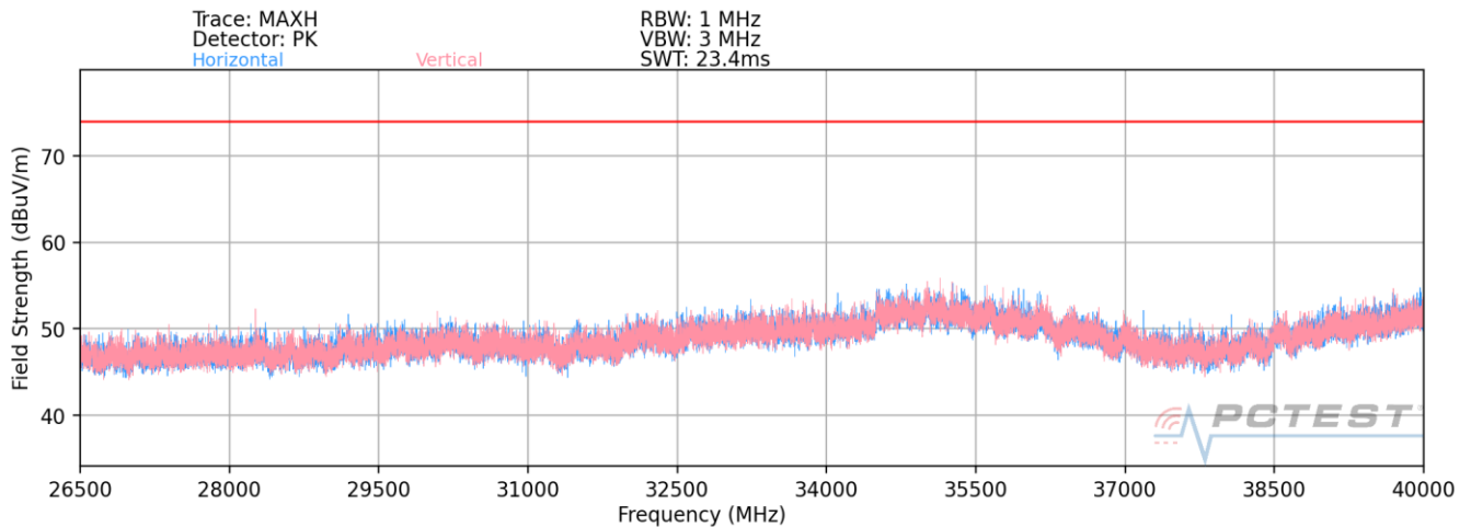
Plot 7-138. Radiated Spurious Plot 26.5GHz - 40GHz (802.11a)
