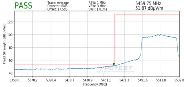
Plot 7-150. Radiated Lower Band Edge Plot (Average – UNII Band 2C)
