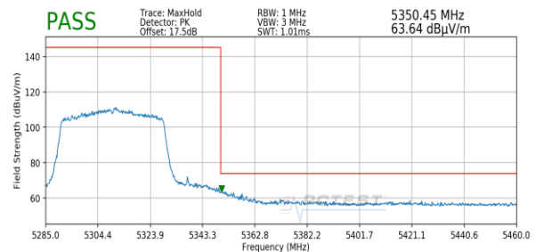
Plot 7-149. Radiated Upper Band Edge Plot (Peak – UNII Band 2A)
