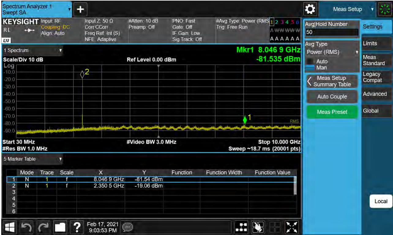
BAND 40. Conducted Spurious Plot 1 (5 MHz 2352.5MHz_QPSK_1RB)
