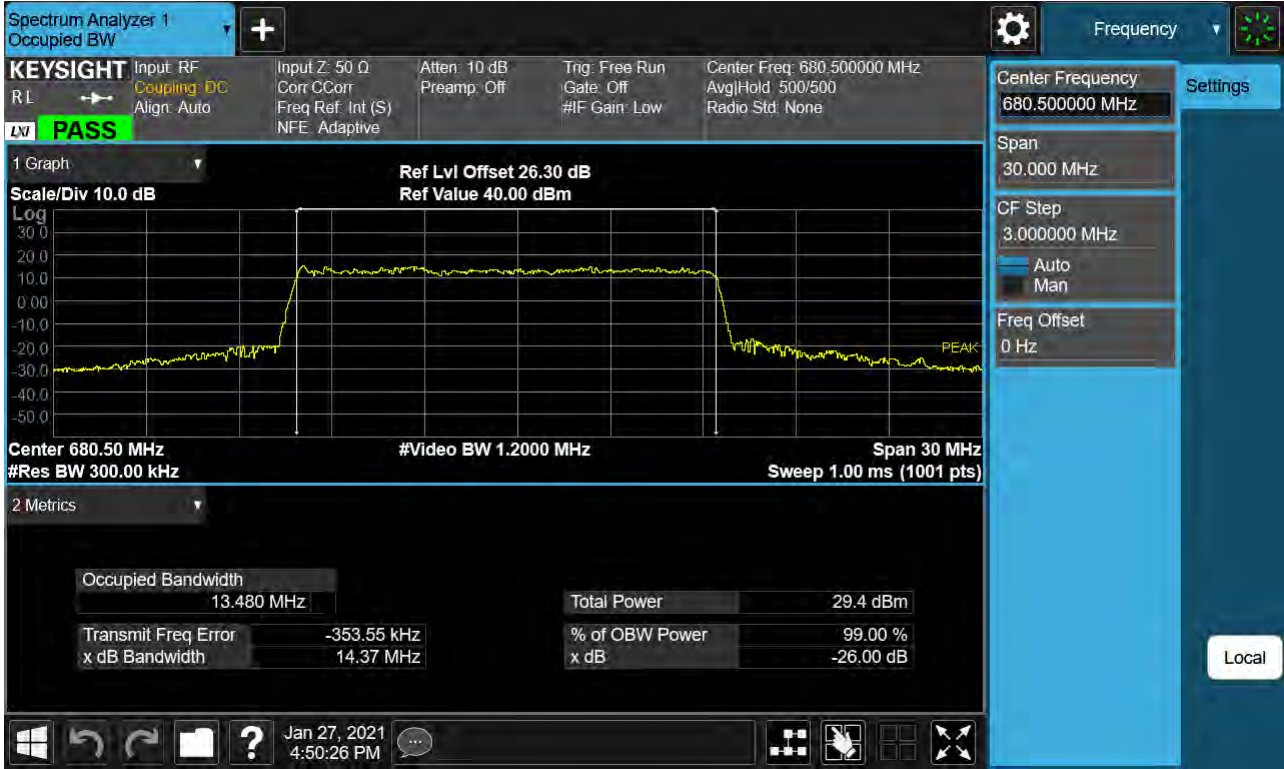
Sub6 n71. Occupied Bandwidth Plot (15M BW Ch.136100 64QAM_ RB79_0)
