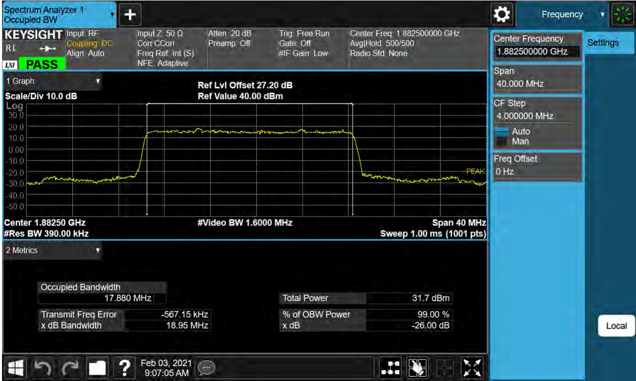
Sub6 n25. Occupied Bandwidth Plot (20M BW Ch.376500 BPSK)
