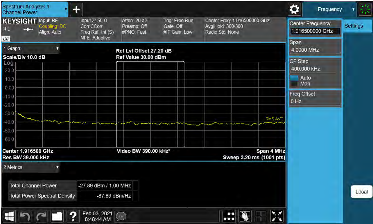
Sub6 n25. Upper Extended Band Edge Plot (10M BW Ch.382000 BPSK_ Full RB) -2
