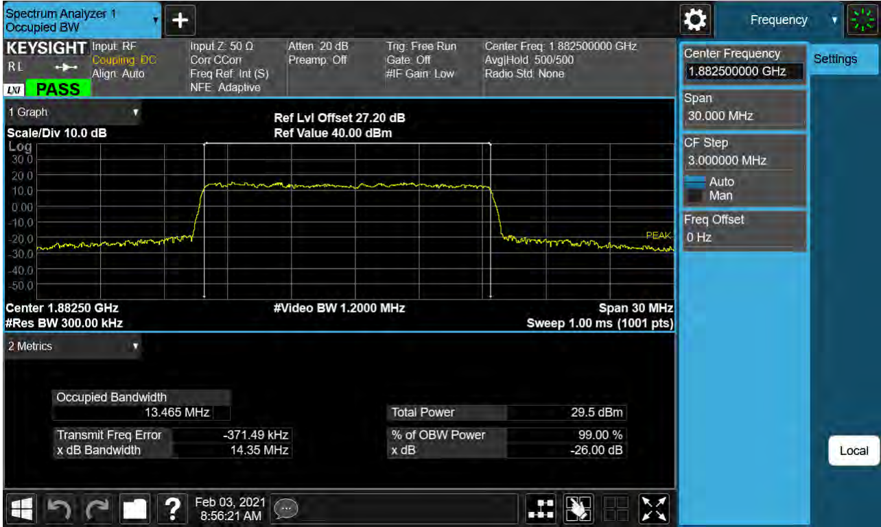
Sub6 n25. Occupied Bandwidth Plot (15M BW Ch.376500 64QAM)
