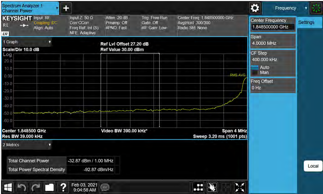
Sub6 n25. Lower Extended Band Edge Plot (20M BW Ch.372000 BPSK_ Full RB) -2
