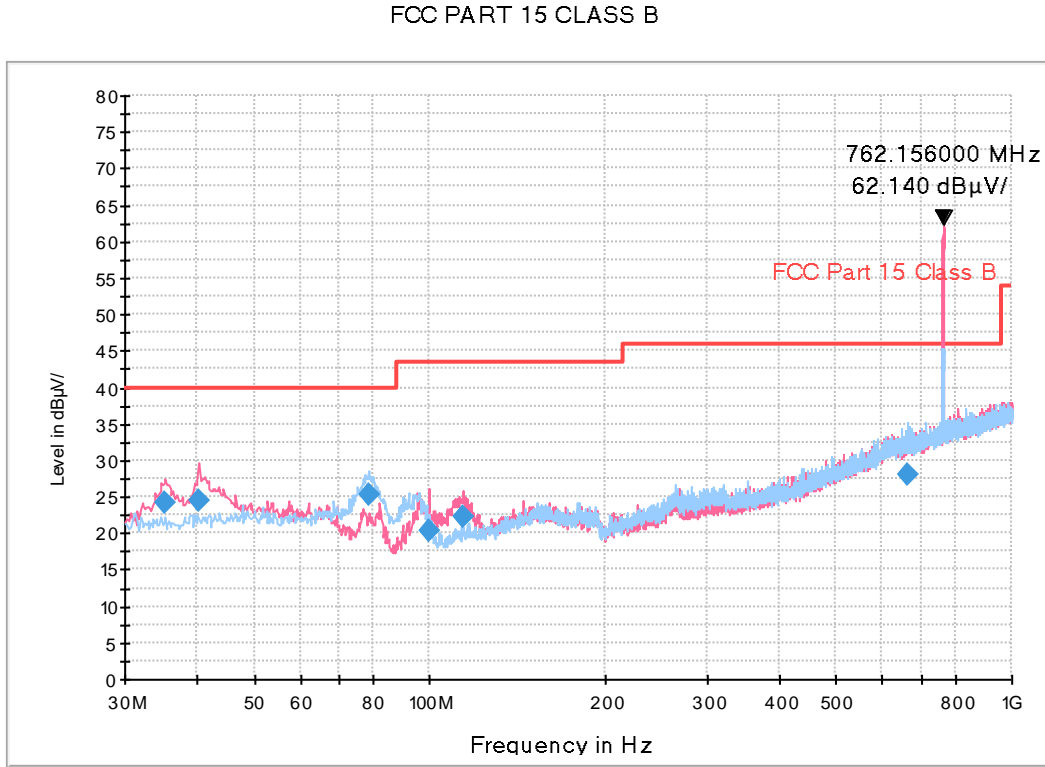
Figure 3: Radiated Emission (30 MHz to 1 GHz), LTE B14 Middle ch Idle
