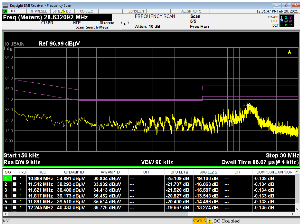
Plot 7-4. Line Conducted Plot with 802.11b (N)
