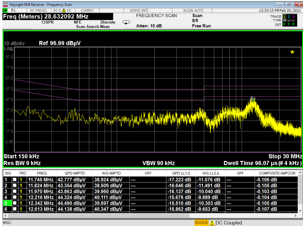
Plot 7-3. Line Conducted Plot with 802.11b (L1)
