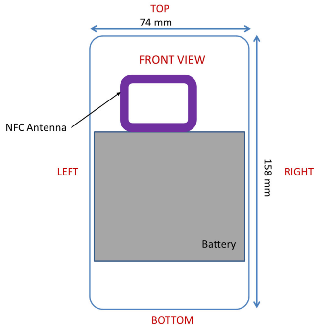
Figure E-2 NFC Antenna Location
