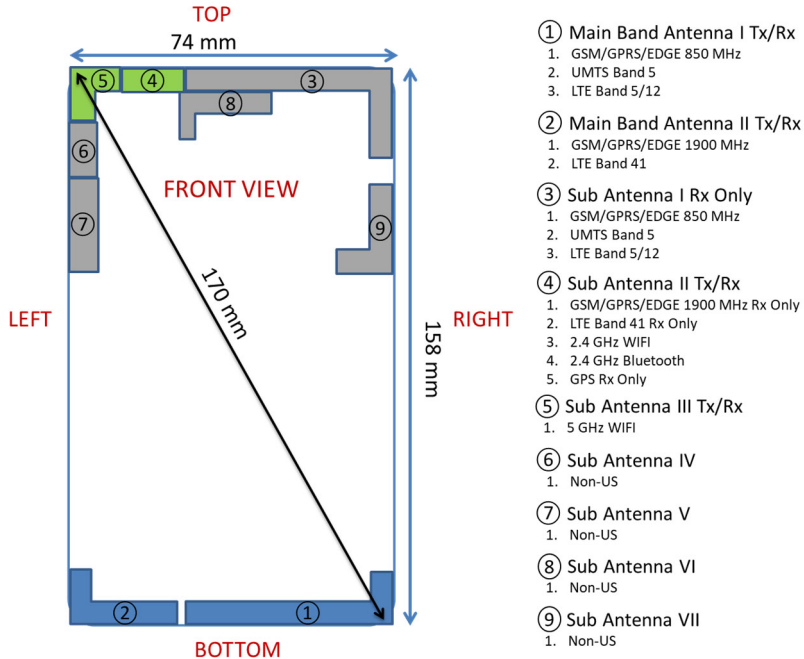
Figure E-1 DUT Antenna Locations
