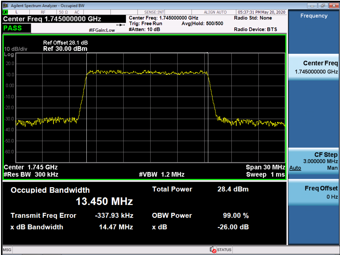
Sub6 n66. Occupied Bandwidth Plot (15M BW Ch.349000 256QAM RB 75)
