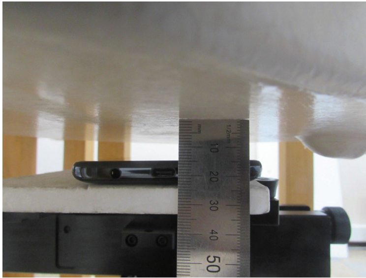
Distance of 15 mm from the EUT (DUT Holder Perturbation)
