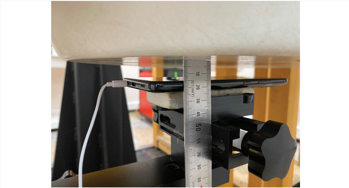
Distance of 15 mm from the EUT with Earphone
