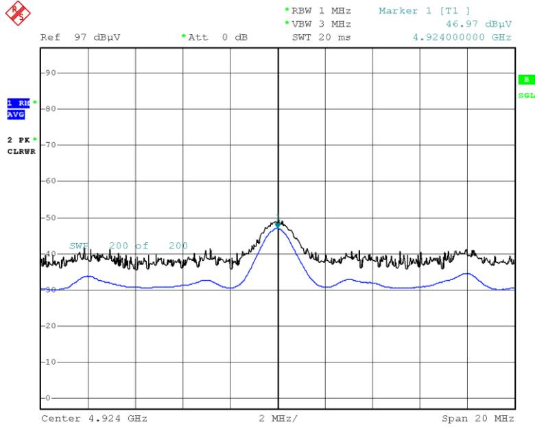
Radiated Spurious Emissions plot – Average Reading (802.11b_1 Mbps, Ch.11 2nd Harmonic)
