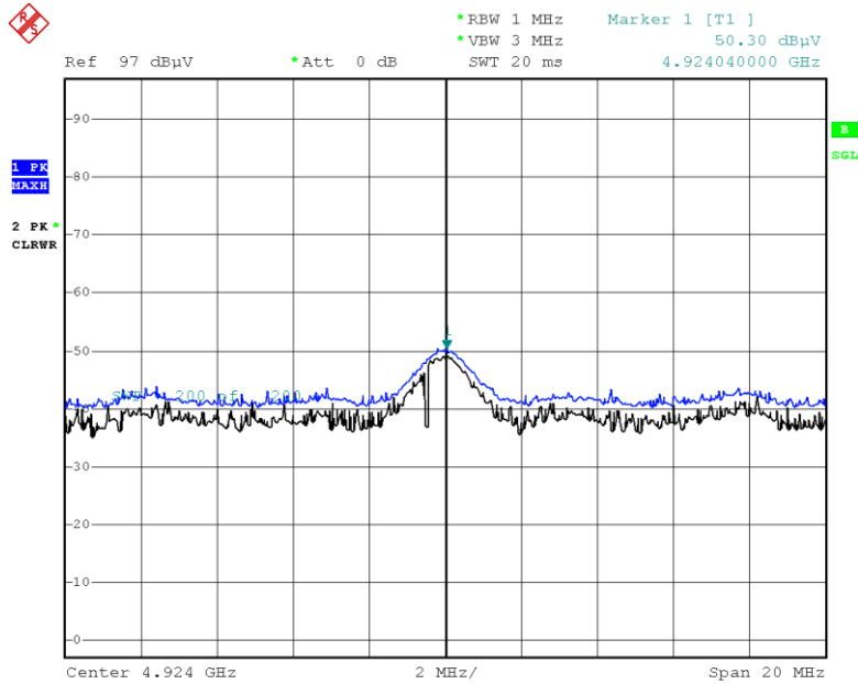
Radiated Spurious Emissions plot – Peak Reading (802.11b_1 Mbps, Ch.11 2nd Harmonic)
