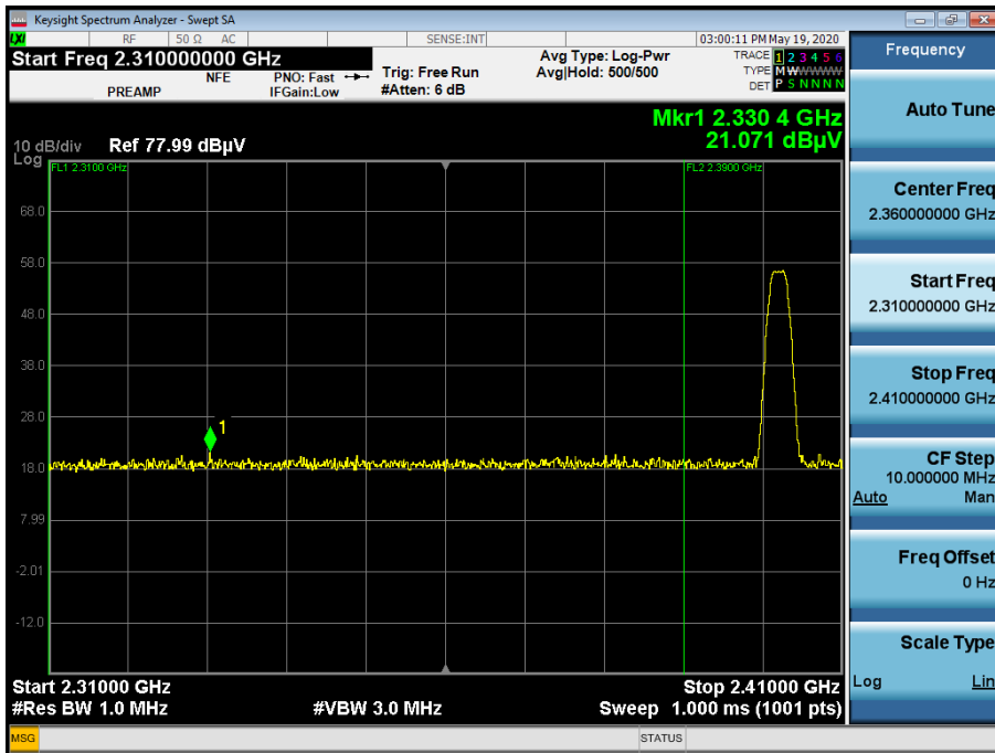
Radiated Restricted Band Edges plot – Peak Reading (Ch.0, Z-H)
