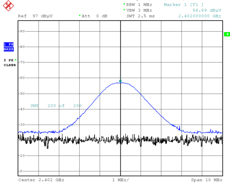
Fundamental Field Strength plot (Ch.0)
