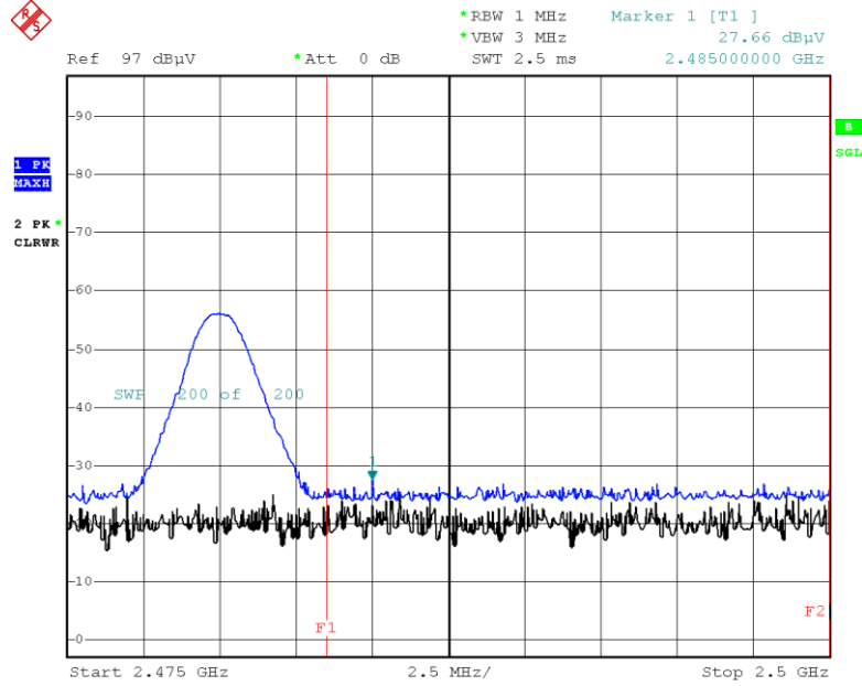
Radiated Band Edges plot – Ch.78
