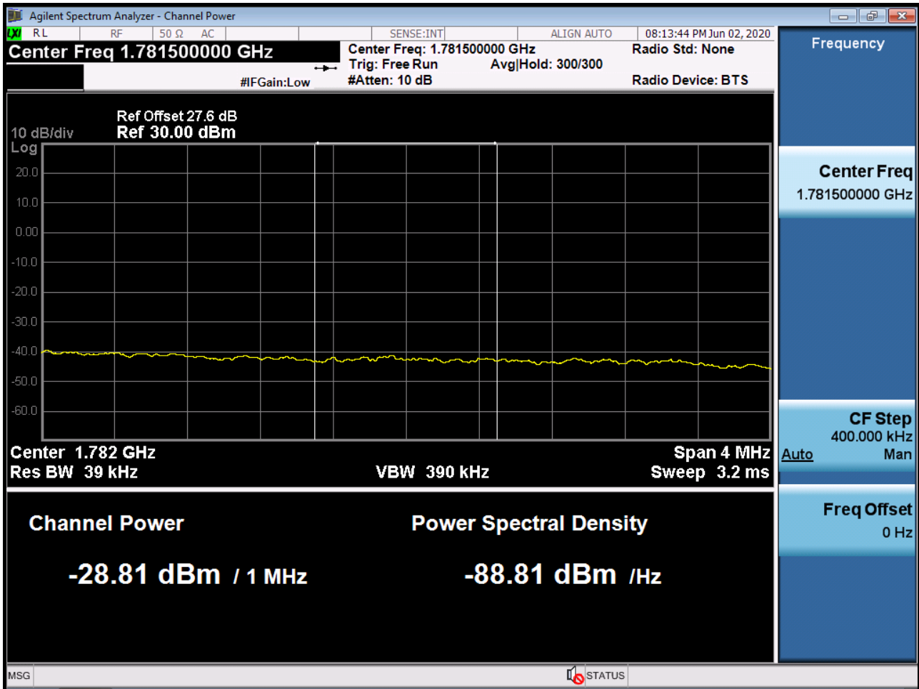
Sub6 n66. Upper Extended Band Edge Plot (20M BW Ch.354000 BPSK_RB100) -3
