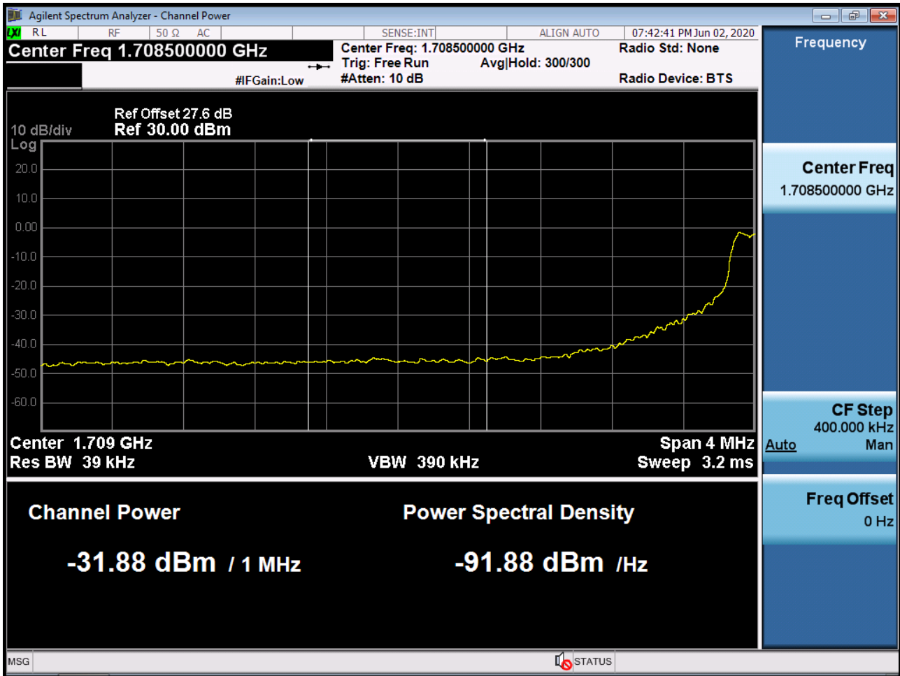
Sub6 n66. Lower Extended Band Edge Plot (15M BW Ch.343500 BPSK_RB75_0) -3
