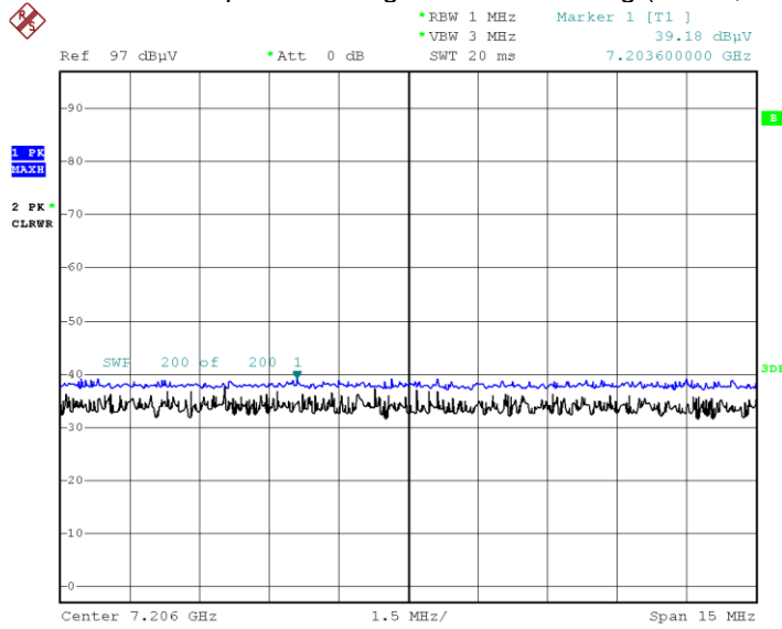
Radiated Spurious Emissions plot – Average & Peak Reading (GFSK, Ch.0 3rd Harmonic, Z-H)
