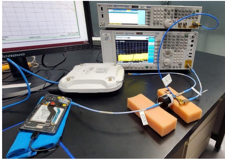
DFS TEST PHOTO
