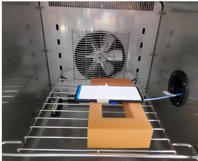
NFC STABILITY TEST PHOTO
