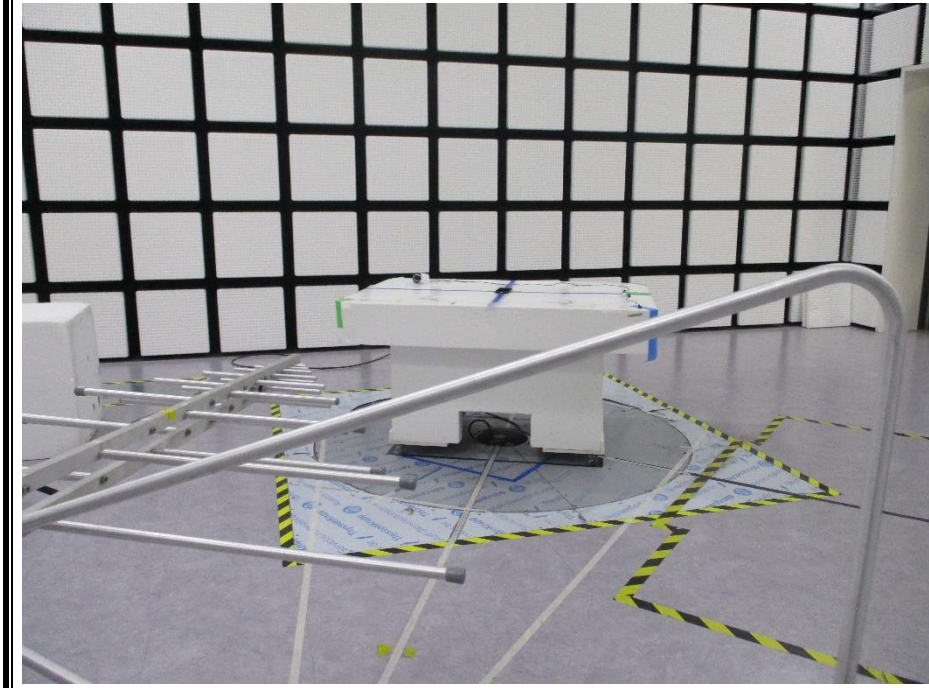
BELOW 1 GHz FRONT TEST PHOTO
