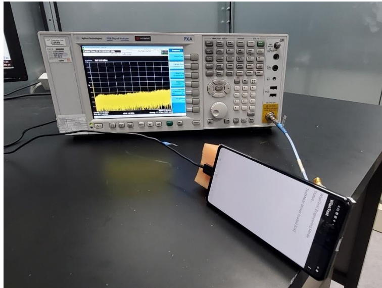
CONDUCTED TEST PHOTO
