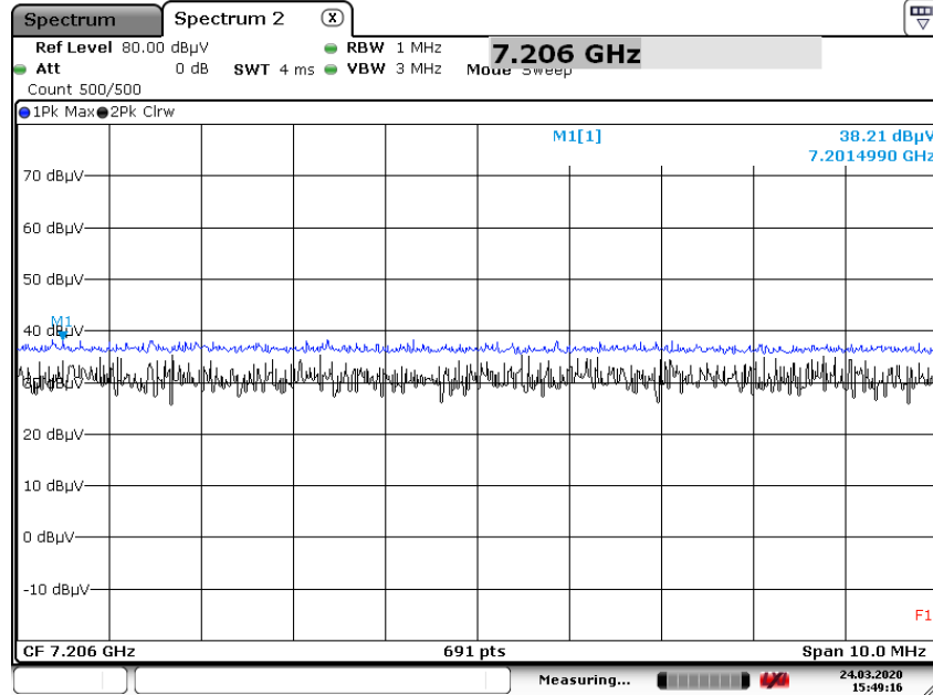
Radiated Spurious Emissions plot – Ch.0 3rd Harmonic
