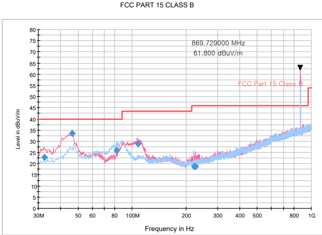
Figure 1: Radiated Emission (30 MHz to 1 GHz), Receiver mode (LTE B5 Low Idle)
