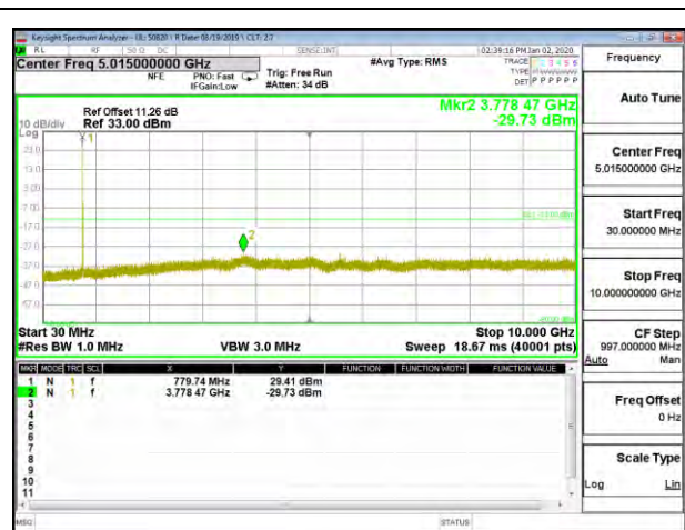
LTE B13 5MHz QPSK Mid Channel RB1-0
