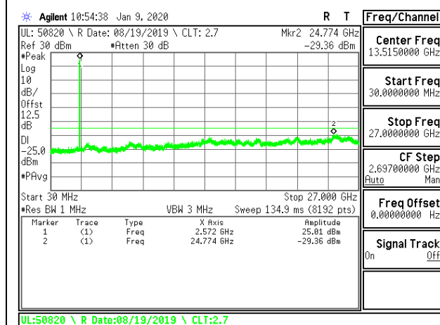
LTE B38 15MHz QPSK Low Channel RB1-0
