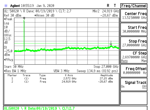
LTE B38 15MHz 16QAM Low Channel RB1-0
