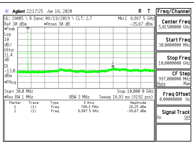
LTE B14 5MHz QPSK Mid Channel RB1-0
