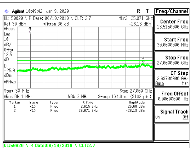
LTE B38 5MHz 16QAM High Channel RB1-0
