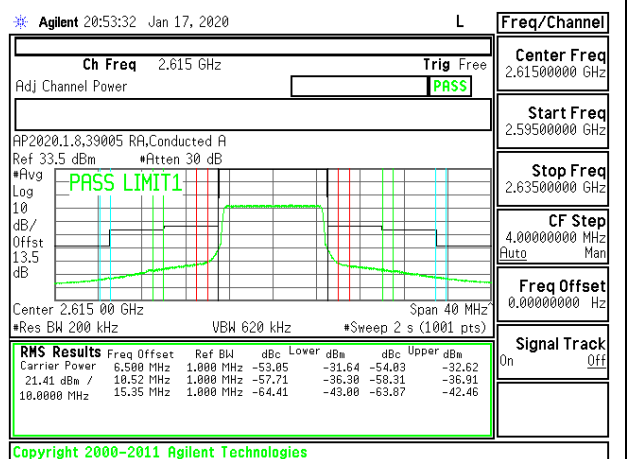
LTE B38 10MHz 16QAM High Channel RB50-0
