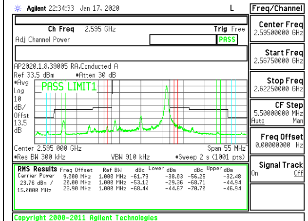
LTE B38 15MHz QPSK Middle Channel RB1-74
