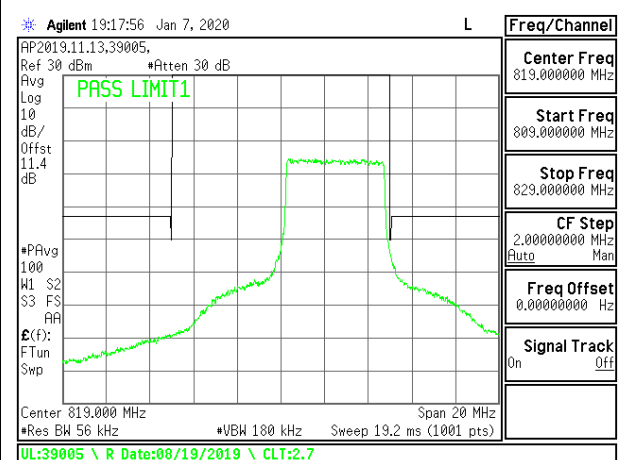
LTE B26 5MHz QPSK High Channel RB25-0
