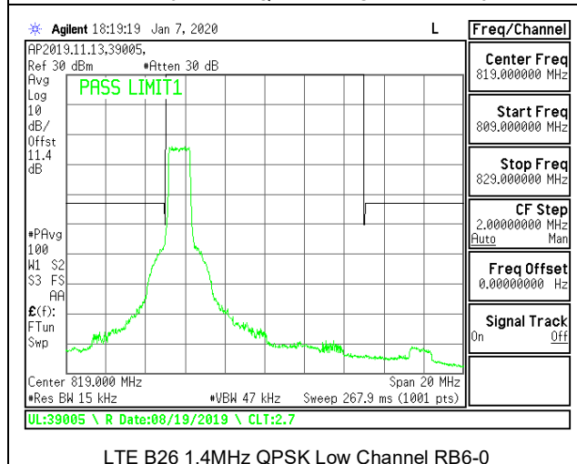
LTE B26 1.4MHz QPSK Low Channel RB6-0
