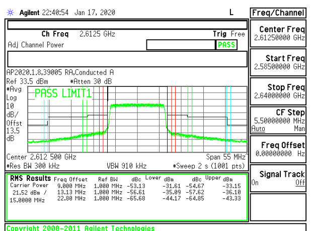
LTE B38 15MHz 16QAM High Channel RB75-0
