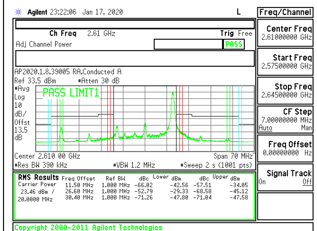
LTE B38 20MHz QPSK High Channel RB1-99
