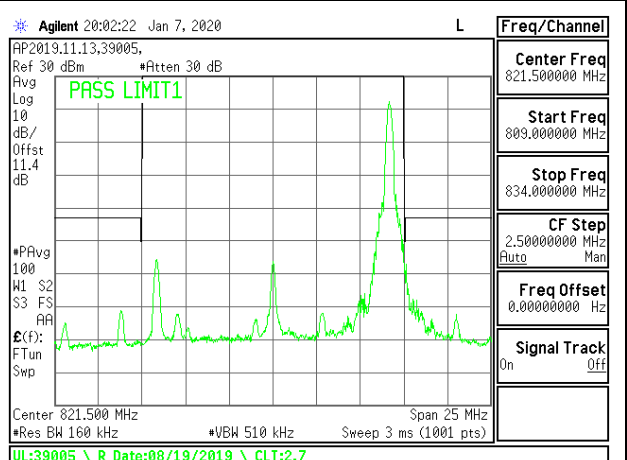
LTE B26 15MHz 16QAM Low Channel RB1-74
