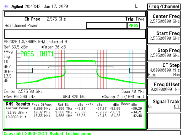
LTE B38 10MHz 16QAM Low Channel RB50-0
