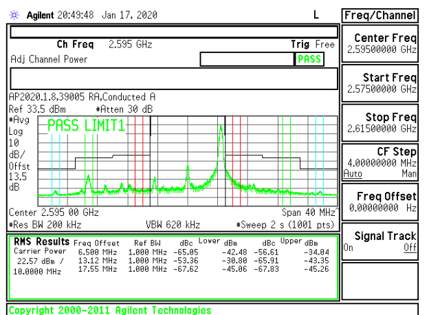
LTE B38 10MHz 16QAM Middle Channel RB1-49
