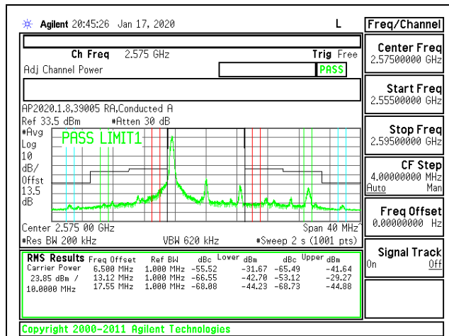
LTE B38 10MHz QPSK Low Channel RB1-0
