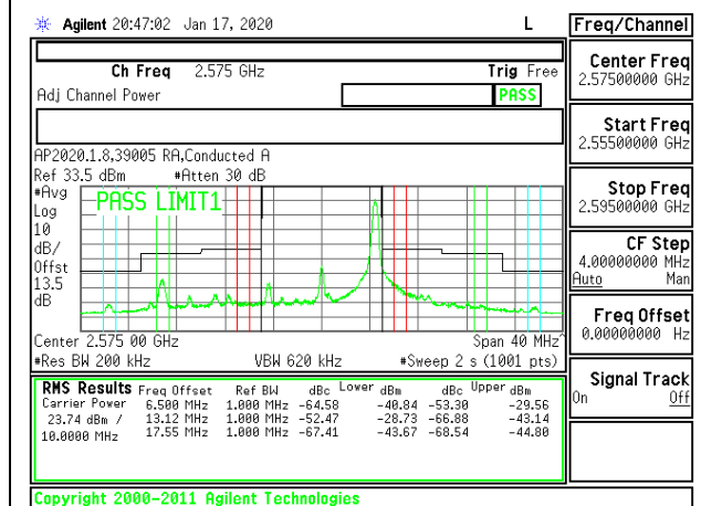
LTE B38 10MHz QPSK Low Channel RB1-49
