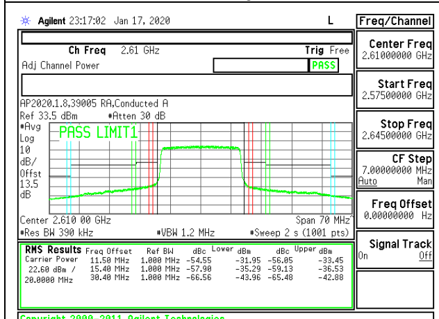
LTE B38 20MHz QPSK High Channel RB100-0
