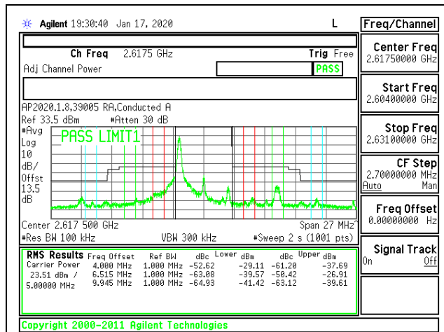
LTE B38 5MHz QPSK High Channel RB1-0
