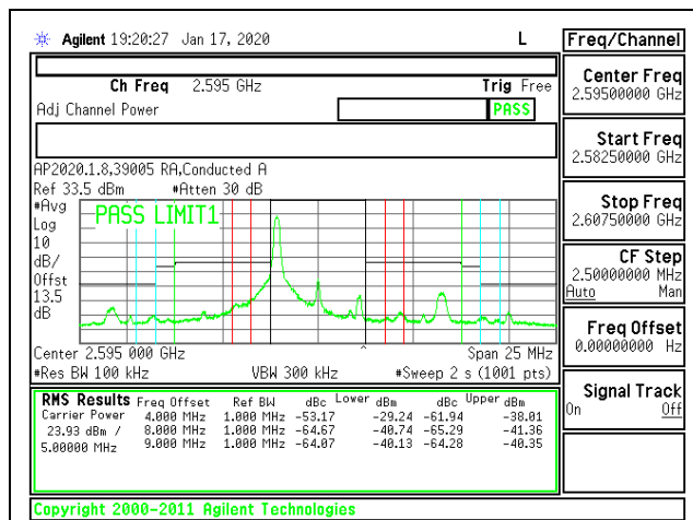
LTE B38 5MHz QPSK Middle Channel RB1-0
