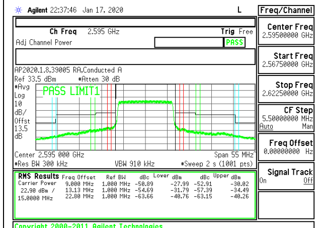
LTE B38 15MHz QPSK Middle Channel RB75-0
