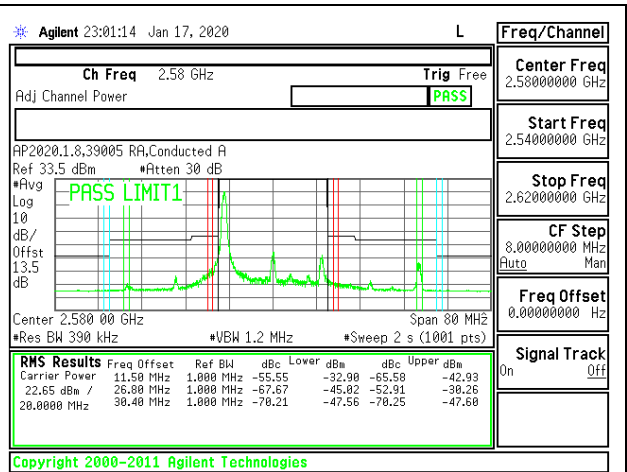
LTE B38 20MHz 16QAM Low Channel RB1-0
