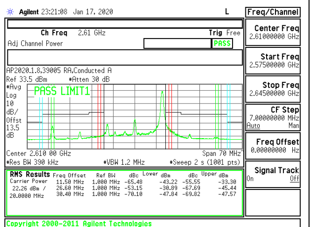
LTE B38 20MHz 16QAM High Channel RB1-99
