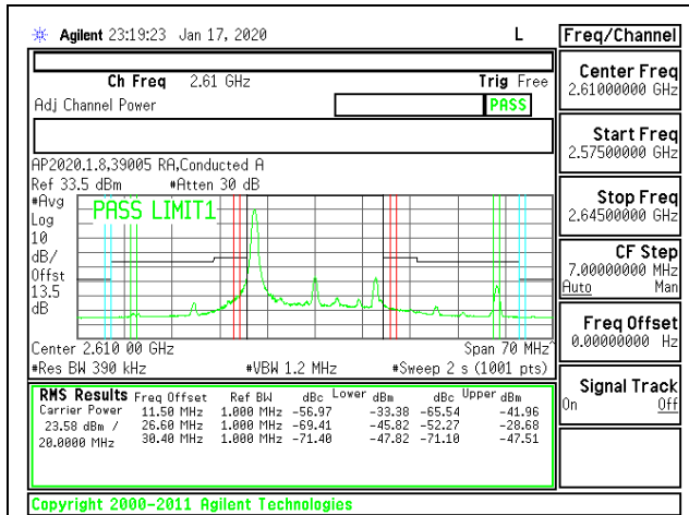
LTE B38 20MHz QPSK High Channel RB1-0
