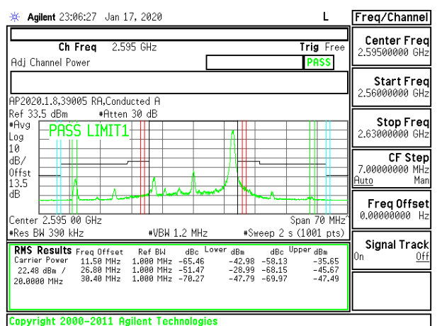
LTE B38 20MHz 16QAM Middle Channel RB1-99
