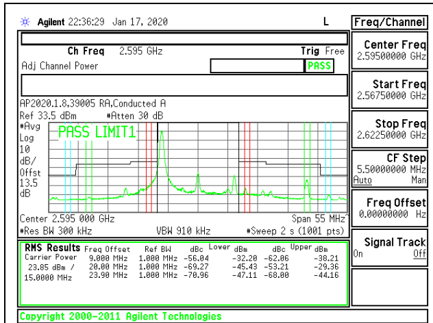
LTE B38 15MHz QPSK Middle Channel RB1-0
