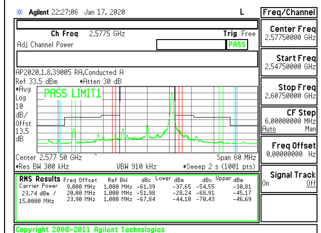
LTE B38 15MHz QPSK Low Channel RB1-74
