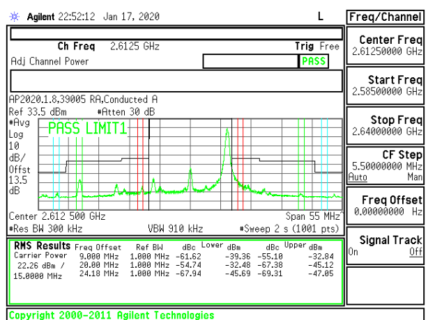
LTE B38 15MHz 16QAM High Channel RB1-74
