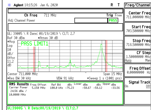
LTE B12 10MHz QPSK High Channel RB1-49
