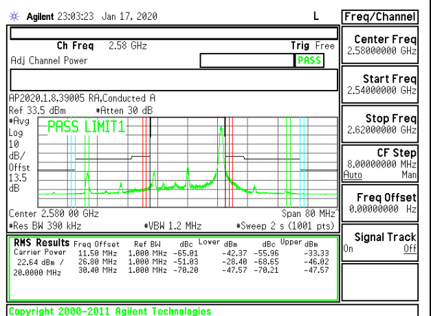
LTE B38 20MHz 16QAM Low Channel RB1-99
