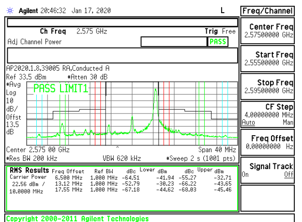
LTE B38 10MHz 16QAM Low Channel RB1-49
