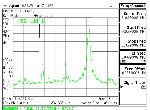
LTE B26 10MHz 16QAM Middle Channel RB1-49
