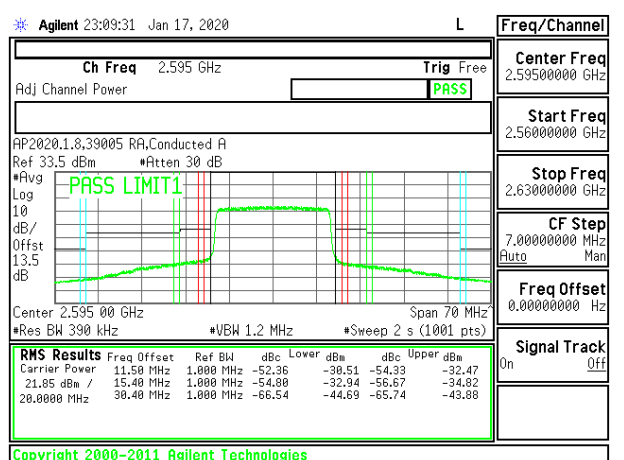
LTE B38 20MHz 16QAM Middle Channel RB100-0
