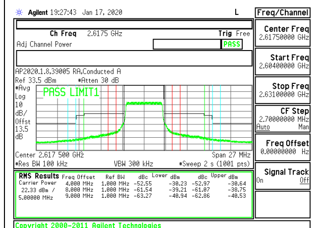
LTE B38 5MHz QPSK High Channel RB25-0
