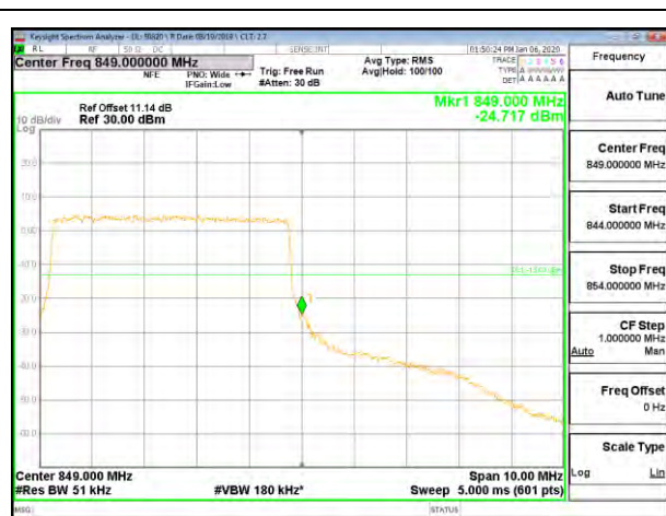
LTE B26 5MHz 16QAM High Channel RB25-0
