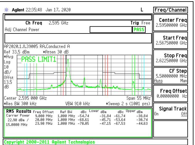
LTE B38 15MHz 16QAM Middle Channel RB1-0
