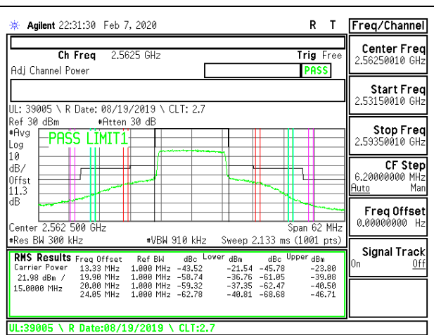
LTE B7 15MHz 16QAM High Channel RB75-0
