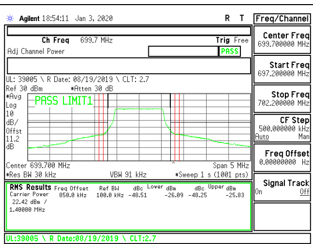
LTE B12 1.4MHz 16QAM Low Channel RB6-0
