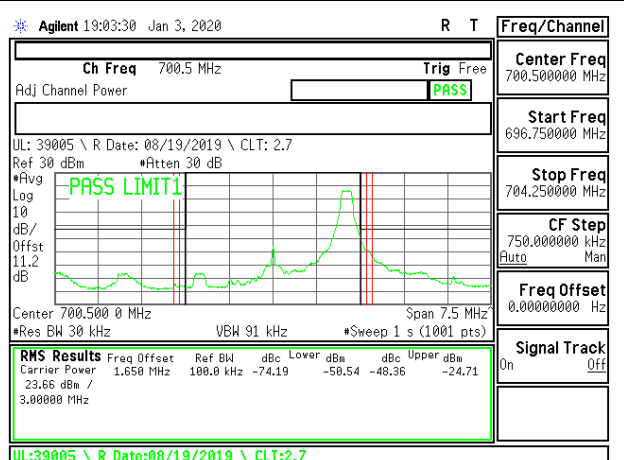
LTE B12 3MHz 16QAM Low Channel RB1-14
