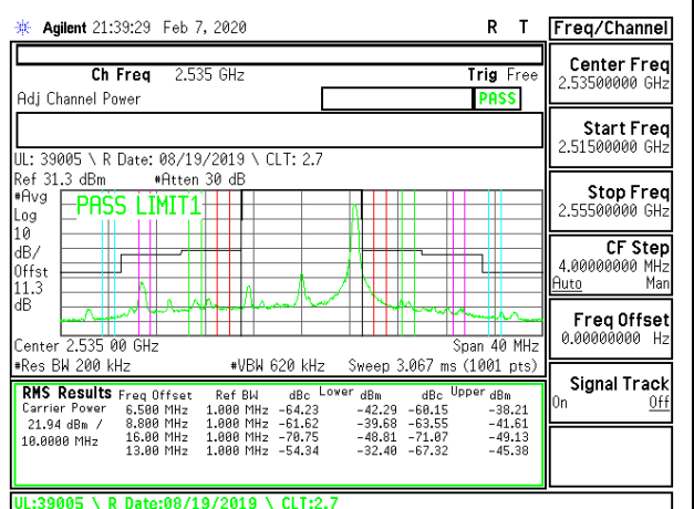
LTE B7 10MHz 16QAM Middle Channel RB1-49
