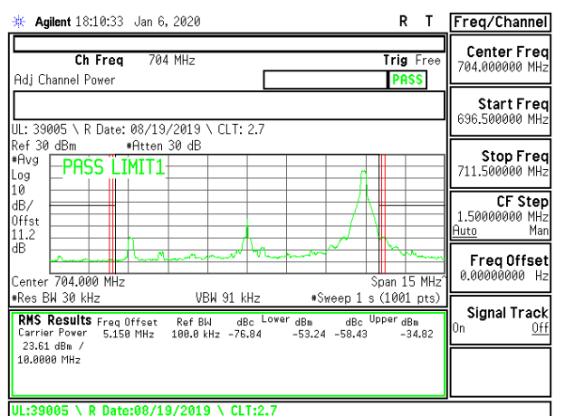
LTE B12 10MHz 16QAM Low Channel RB1-49
