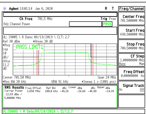
LTE B12 5MHz 16QAM Low Channel RB25-0
