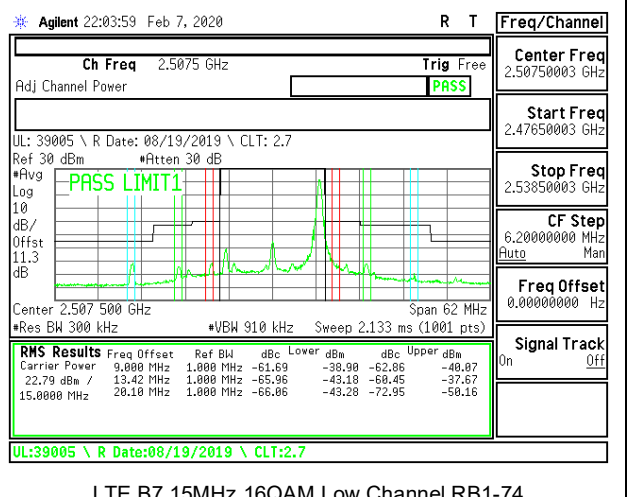
LTE B7 15MHz 16QAM Low Channel RB1-74
