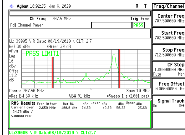
LTE B12 5MHz QPSK Middle Channel RB1-24
