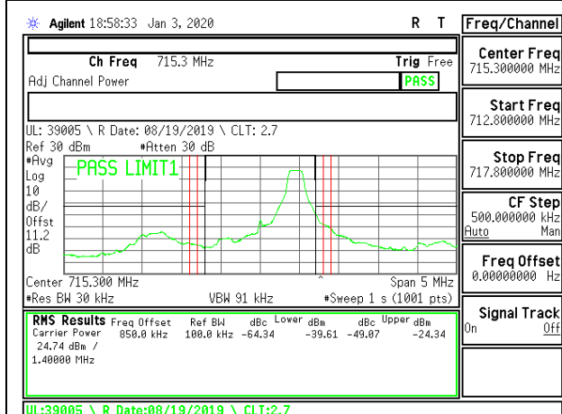
LTE B12 1.4MHz QPSK High Channel RB1-5
