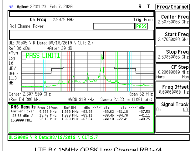
LTE B7 15MHz QPSK Low Channel RB1-74
