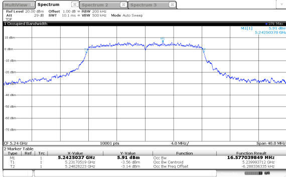
UNII-1 / 802.11n HT20 / 5 240 MHz
