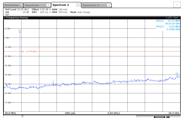
Conducted spurious / High ch.
