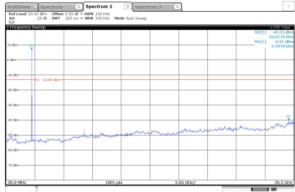
Conducted spurious / Mid ch.
