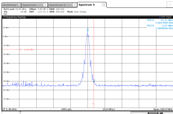
Conducted band-edge / High ch.
