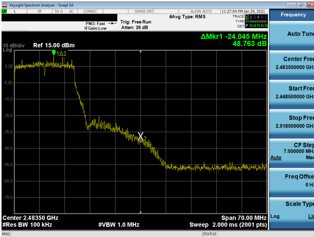
Plot 7-24. Band Edge Plot (802.11g – Ch. 10)
