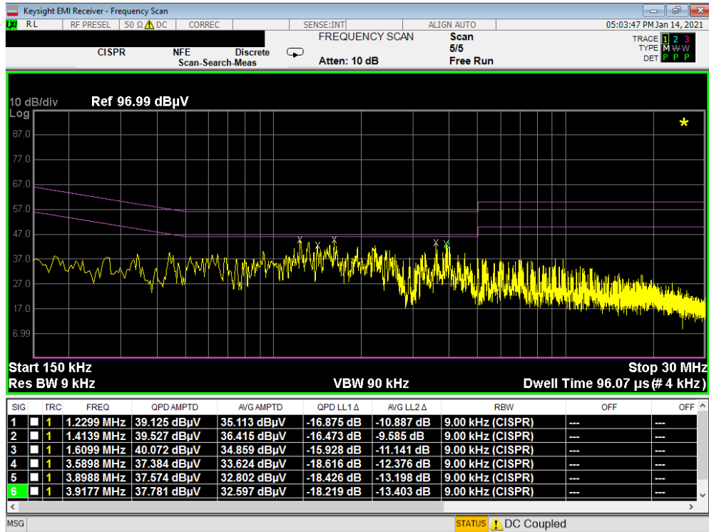
Plot 7-59. Line Conducted Plot with 802.11b (L1)
