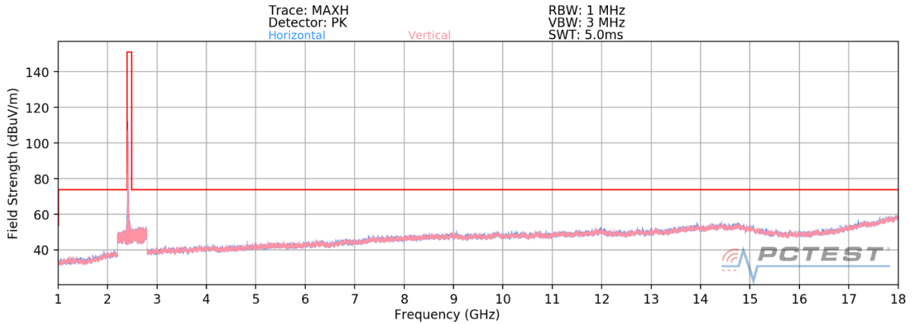
Plot 7-40. Radiated Spurious Plot above 1GHz (802.11b – Ch. 1)
