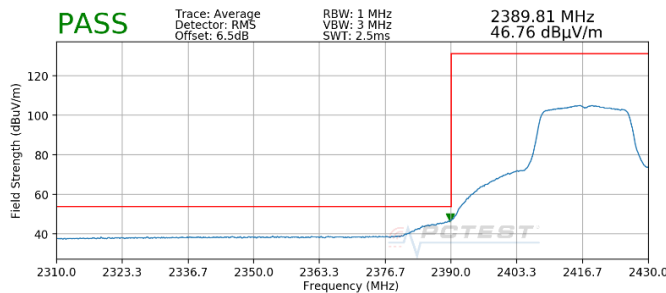
Plot 7-46. Radiated Restricted Lower Band Edge Measurement (Average)
