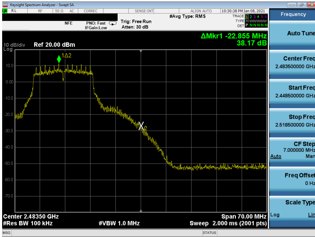
Plot 7-25. Band Edge Plot (802.11g – Ch. 11)
