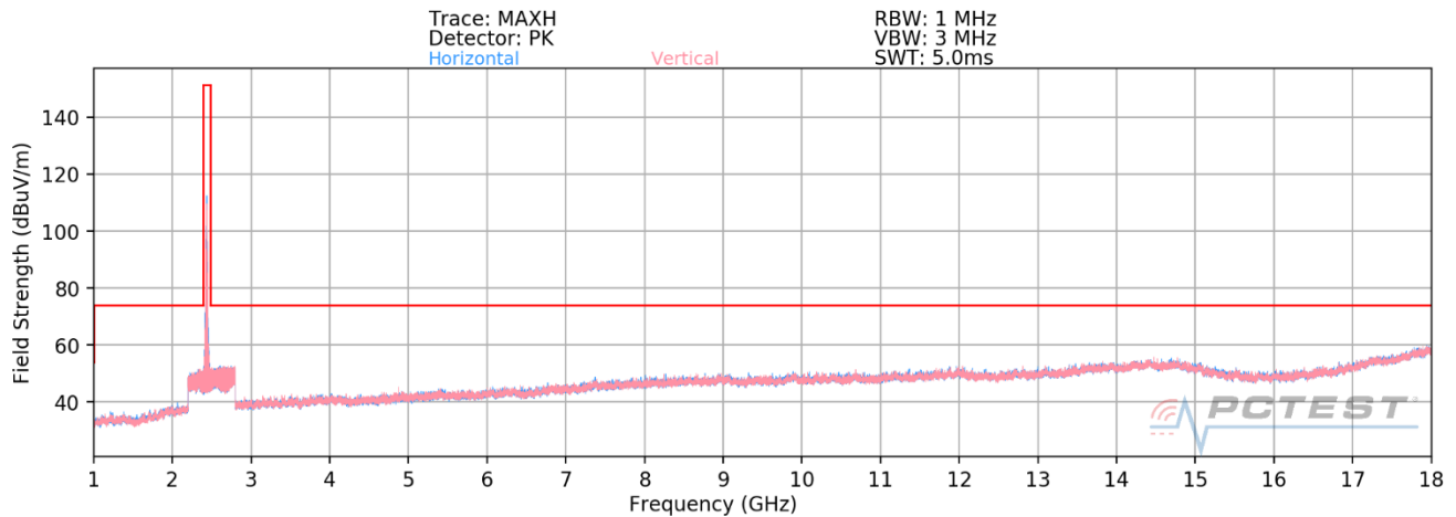
Plot 7-41. Radiated Spurious Plot above 1GHz (802.11b – Ch. 6)
