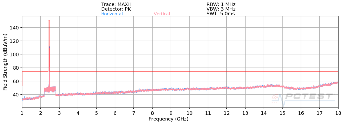
Plot 7-42. Radiated Spurious Plot above 1GHz (802.11b – Ch. 11)
