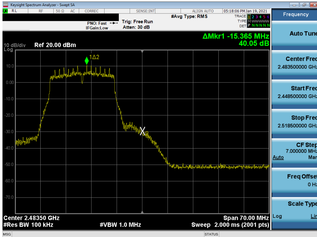
Plot 7-32. Band Edge Plot (802.11n (2.4GHz) – Ch. 12)
