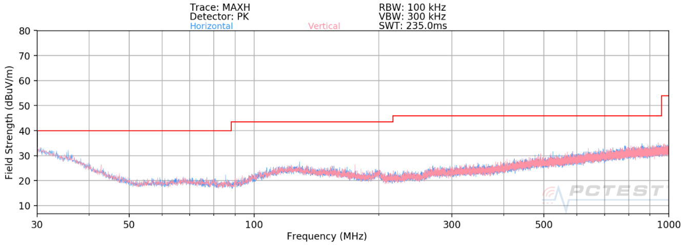
Plot 7-58. Radiated Spurious Plot below 1GHz
