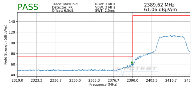
Plot 7-47. Radiated Restricted Lower Band Edge Measurement (Peak)
