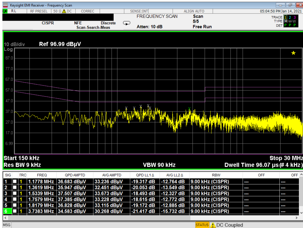
Plot 7-60. Line Conducted Plot with 802.11b (N)
