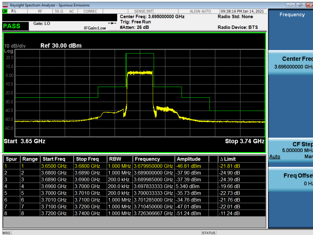
Plot 7-30. Upper Band Edge Plot (LTE Band 48 - 10MHz QPSK – Full RB Configuration)
