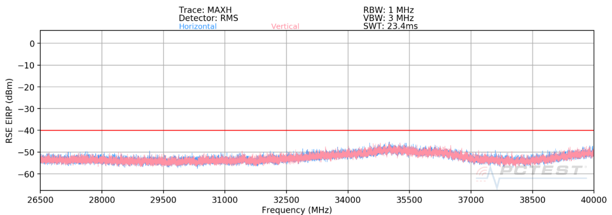
Plot 7-35. Radiated Spurious Plot 26.5 - 40GHz (Band 48)
