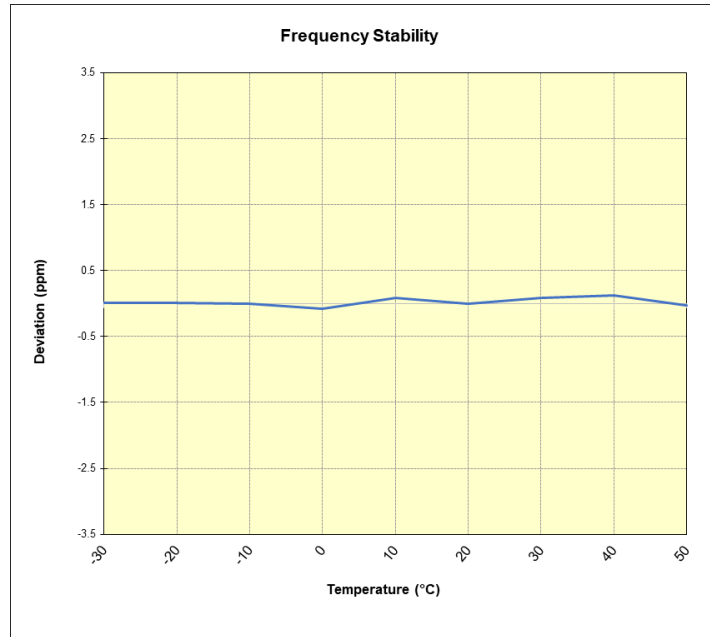
Figure 7-6. Frequency Stability Graph (LTE Band 48)
