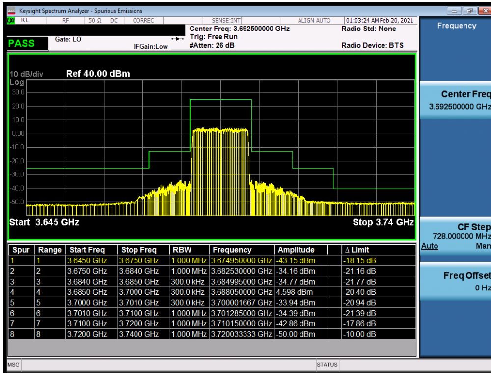
Plot 7-28. Upper Band Edge Plot (LTE Band 48 - 15MHz QPSK – Full RB Configuration)
