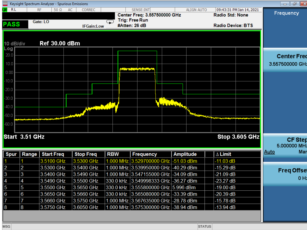
Plot 7-27. Lower Band Edge Plot (LTE Band 48 - 15MHz QPSK – Full RB Configuration)
