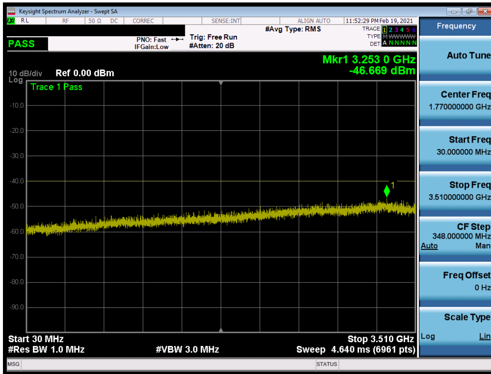
Plot 7-13. Conducted Spurious Plot (LTE Band 48 - 20MHz QPSK - RB Size 1, RB Offset 0 - Low Channel)
