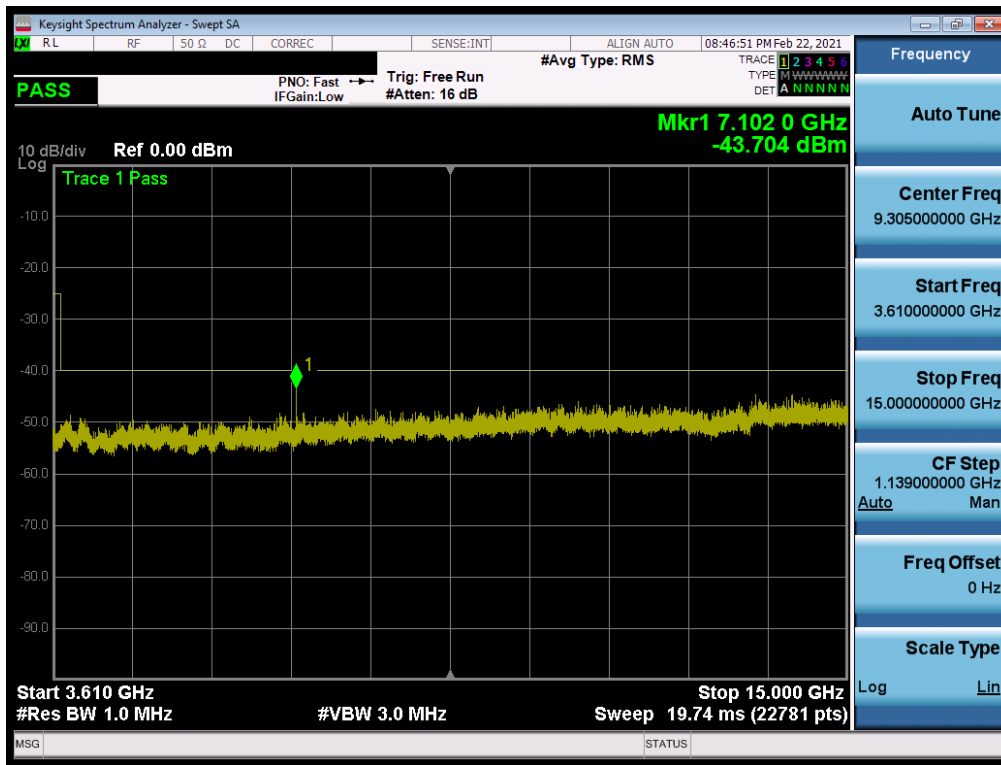
Plot 7-14. Conducted Spurious Plot (LTE Band 48 - 20MHz QPSK - RB Size 1, RB Offset 0 - Low Channel)
