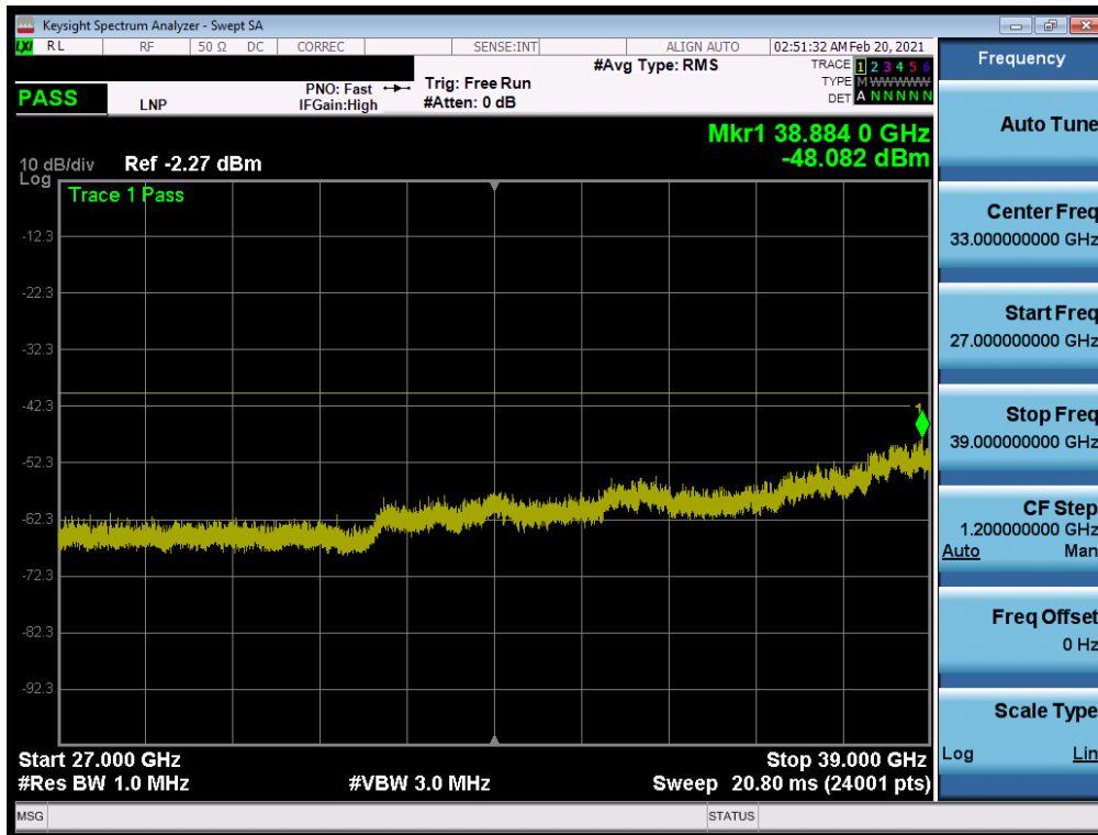
Plot 7-20. Conducted Spurious Plot (LTE Band 48 - 20MHz QPSK - RB Size 1, RB Offset 0 - Mid Channel)
