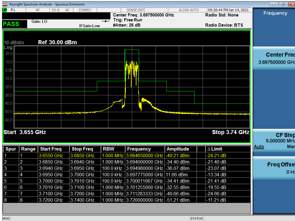
Plot 7-32. Upper Band Edge Plot (LTE Band 48 - 5MHz QPSK – Full RB Configuration)
