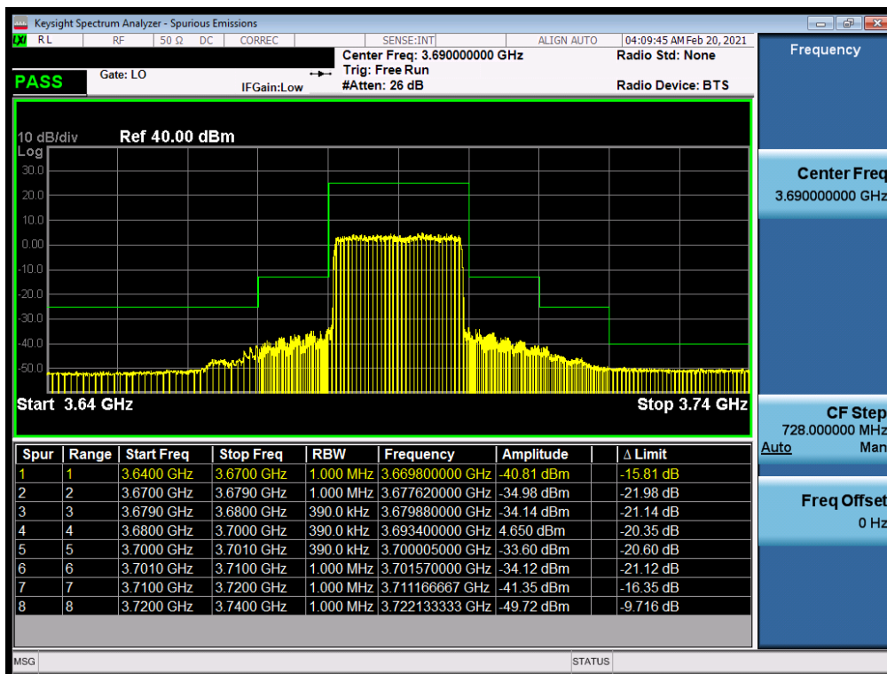
Plot 7-26. Upper Band Edge Plot (LTE Band 48 - 20MHz QPSK – Full RB Configuration)
