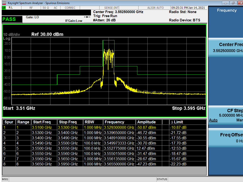
Plot 7-31. Lower Band Edge Plot (LTE Band 48 - 5MHz QPSK – Full RB Configuration)
