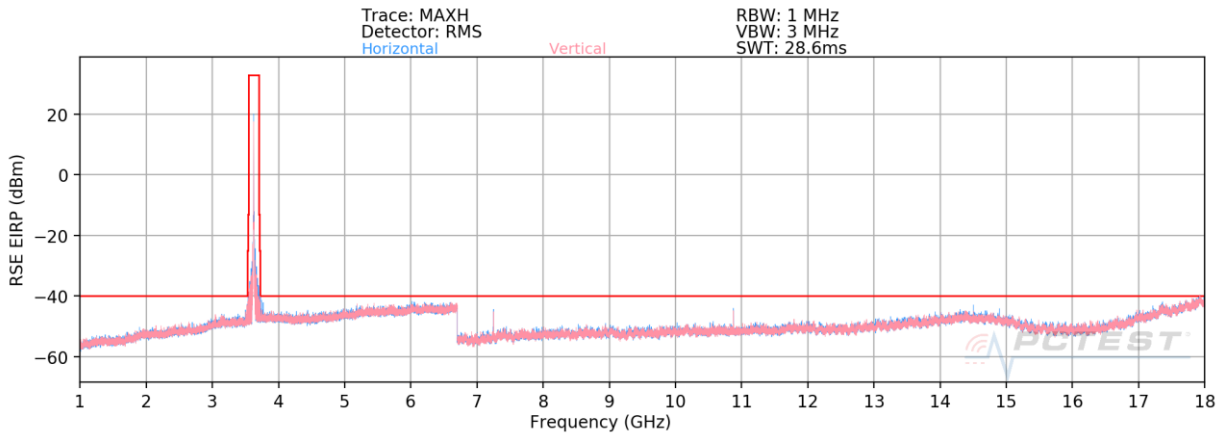
Plot 7-33. Radiated Spurious Plot 1 - 18GHz (Band 48)
