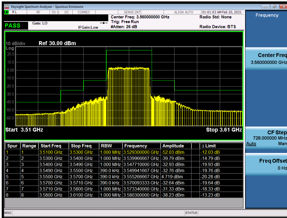
Plot 7-25. Lower Band Edge Plot (LTE Band 48 - 20MHz QPSK – Full RB Configuration)
