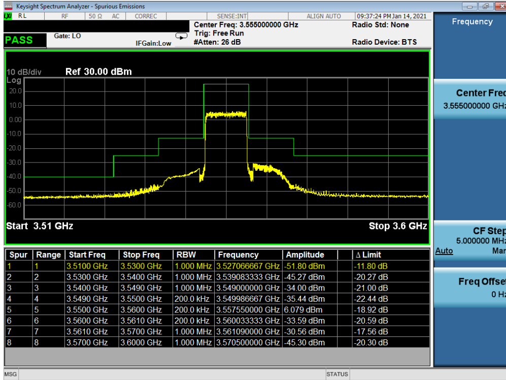
Plot 7-29. Lower Band Edge Plot (LTE Band 48 - 10MHz QPSK – Full RB Configuration)
