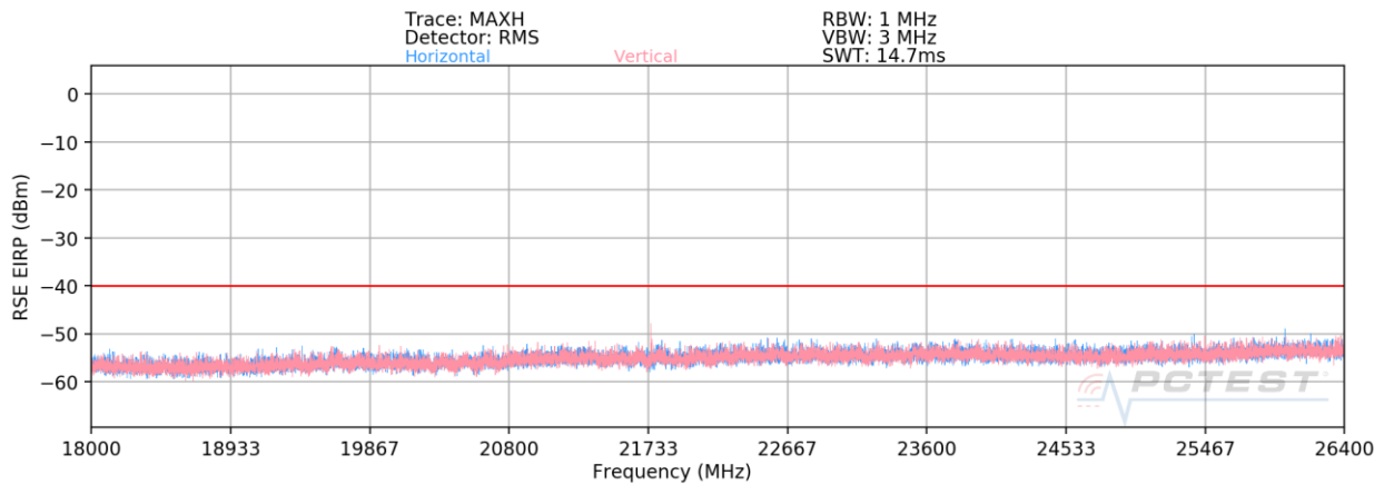
Plot 7-34. Radiated Spurious Plot 18 - 26.5GHz (Band 48)
