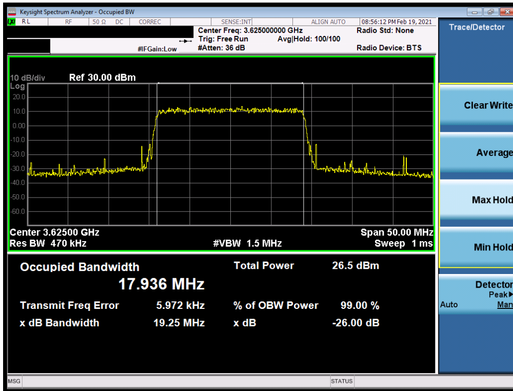
Plot 7-2. Occupied Bandwidth Plot (LTE Band 48 - 20MHz 16-QAM - Full RB Configuration)
