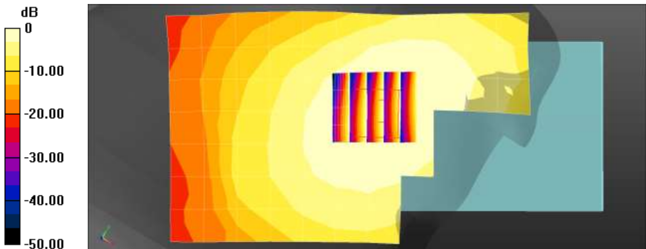
0 dB = 0.256 W/kg = -5.92 dBW/kg
