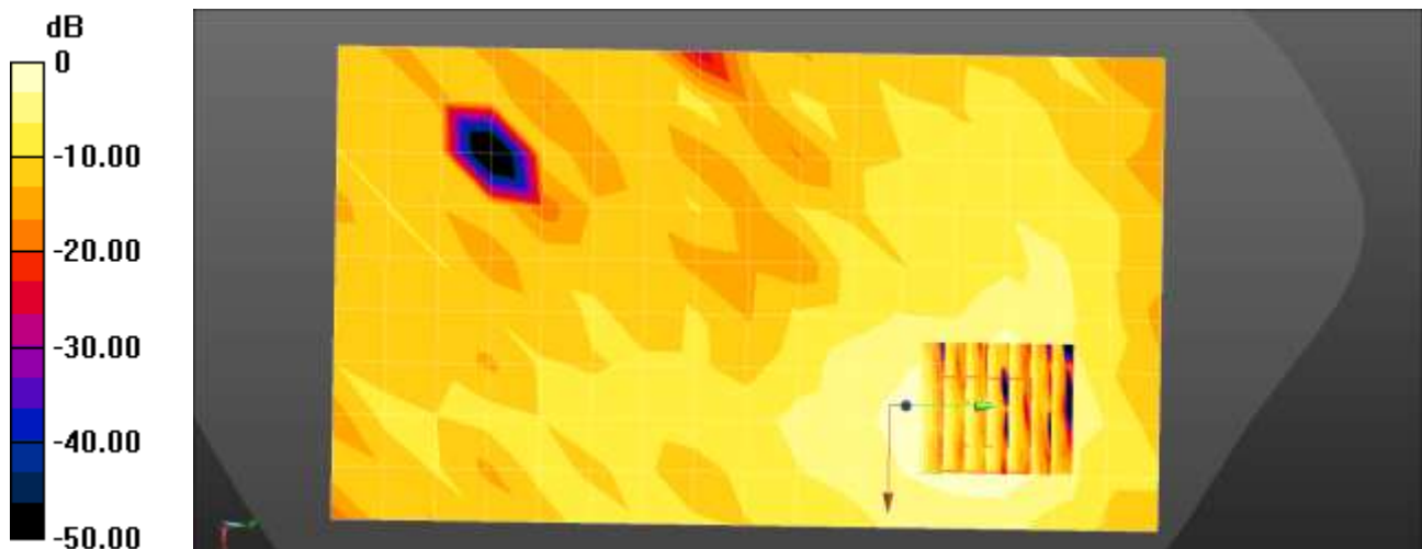
0 dB = 0.0228 W/kg = -16.42 dBW/kg
