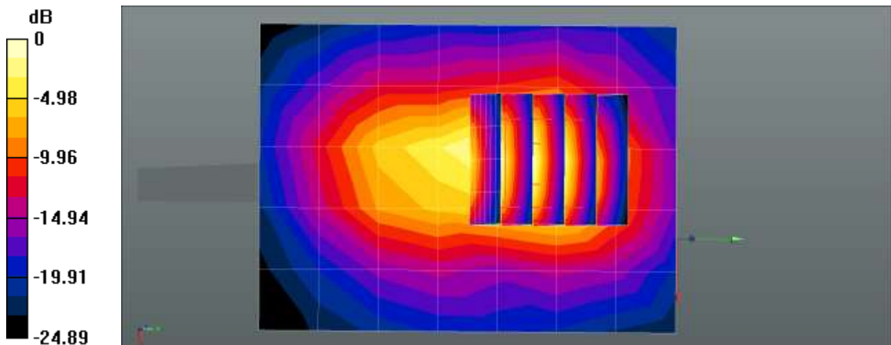
0 dB = 3.78 W/kg = 5.77 dBW/kg
