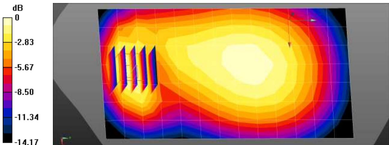
0 dB = 0.259 W/kg = -5.87 dBW/kg
