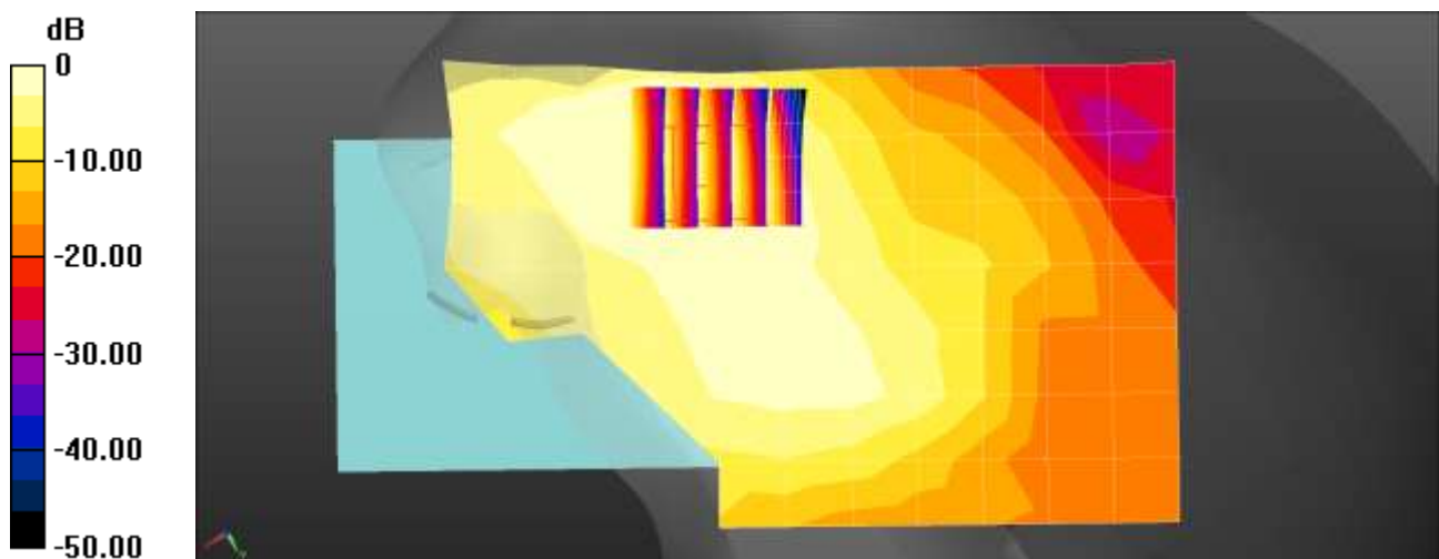
0 dB = 0.125 W/kg = -9.02 dBW/kg
