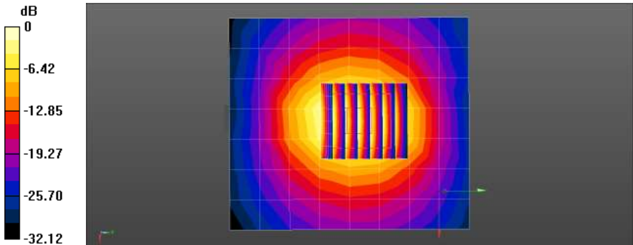
0 dB = 3.78 W/kg = 5.78 dBW/kg
