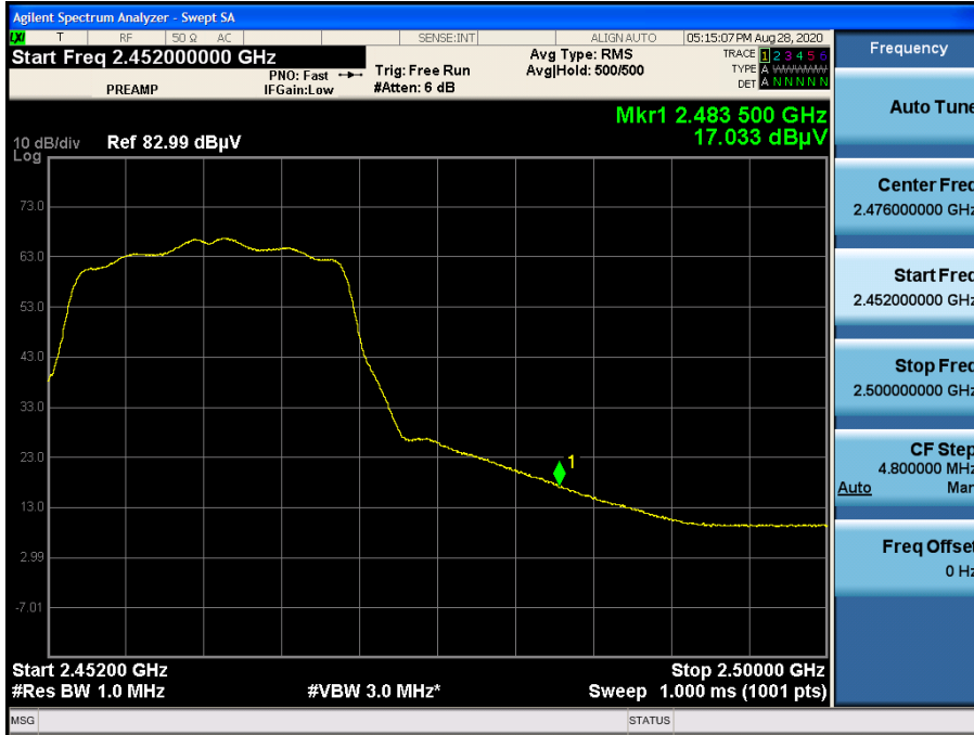
Radiated Restricted Band Edges plot – Average Reading (802.11g_6 Mbps Ch.11)
