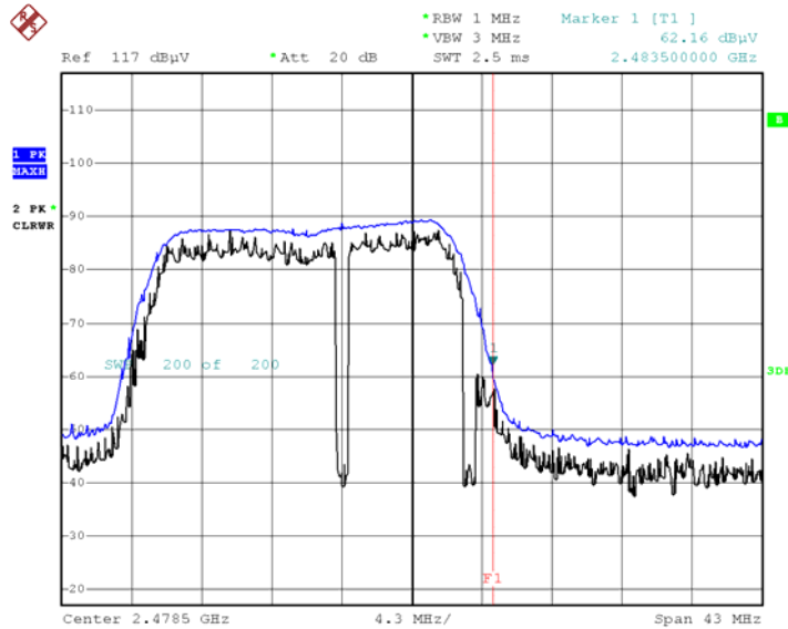
Radiated Restricted Band Edges plot – Peak Reading (802.11n (HT20)_ Ch.13)
