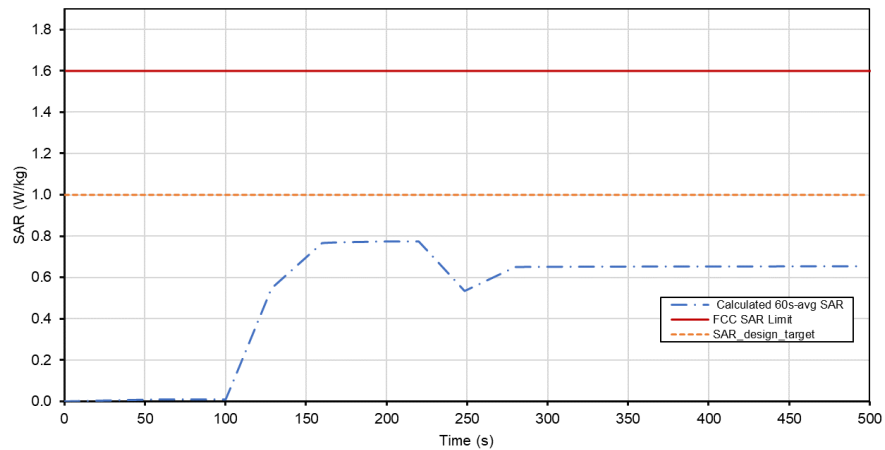
Total Time-Averaged SAR Test Sequence A Tech: LTE, Band 48, Ant G
