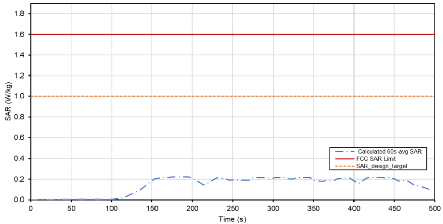
Total Time-Averaged SAR Test Sequence B Tech: LTE, Band 66, Ant B
