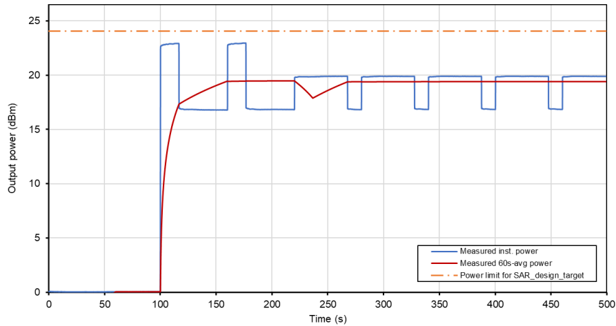
Time-Averaged Conducted Power Test Sequence A Tech: WCDMA, Band 2
