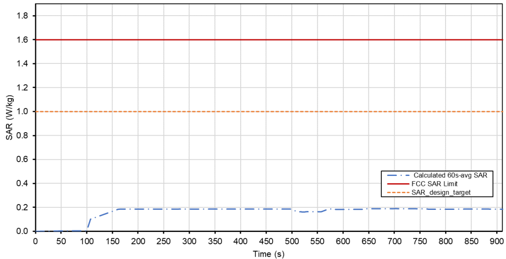
Total Time-Averaged SAR Change in Call Tech: 5G NR SUB6, n41, Ant B
