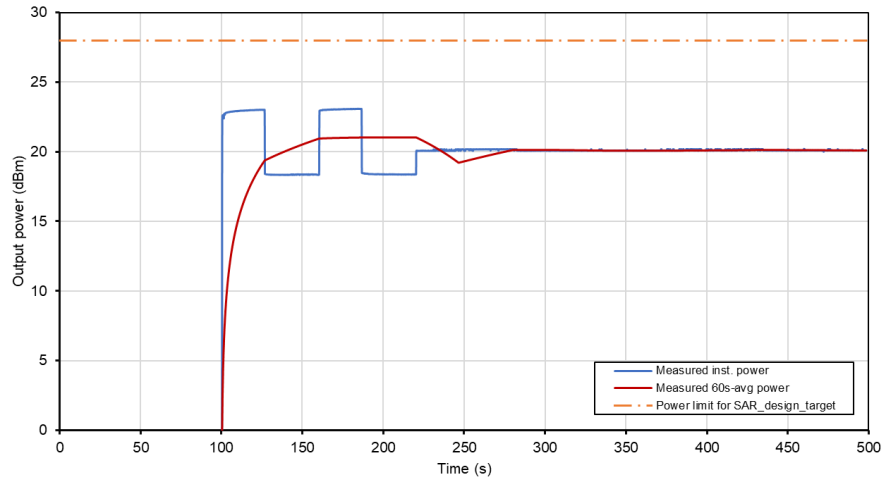
Time-Averaged Conducted Power Test Sequence A Tech: 5GNR SUB6, n66, Ant B
