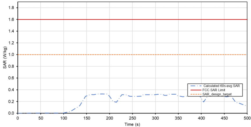
Total Time-Averaged SAR Test Sequence B Tech: WCDMA, Band 2
