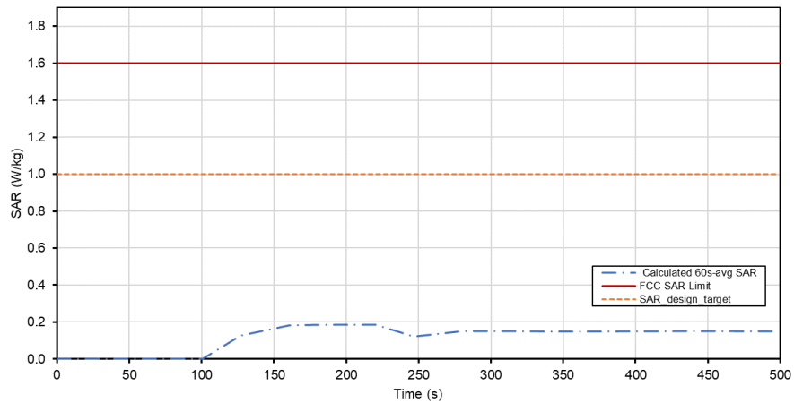
Total Time-Averaged SAR Test Sequence A Tech: 5GNR SUB6, n66, Ant B
