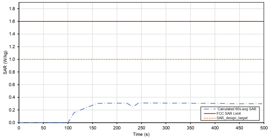
Total Time-Averaged SAR Test Sequence A Tech: GPRS, Band 1900
