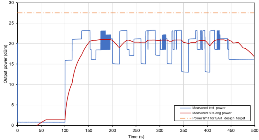
Time-Averaged Conducted Power Test Sequence B Tech: LTE, Band 66, Ant B
