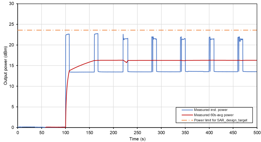
Time-Averaged Conducted Power Test Sequence A Tech: 5G NR SUB6, n41, Ant B
