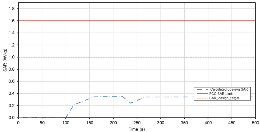
Total Time-Averaged SAR Test Sequence A Tech: WCDMA, Band 2
