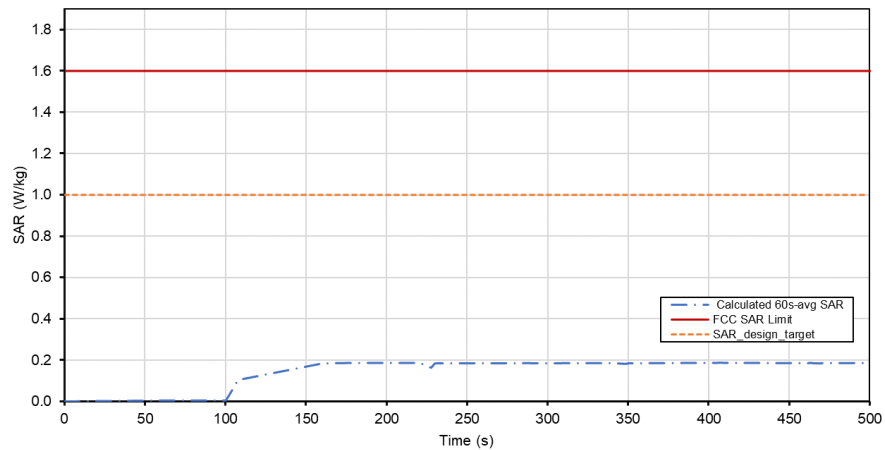
Total Time-Averaged SAR Test Sequence A Tech: 5G NR SUB6, n41, Ant B
