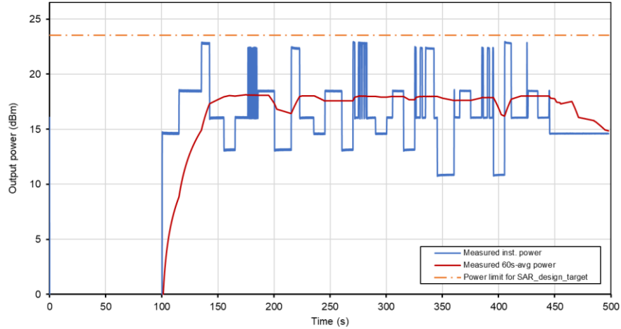
Time-Averaged Conducted Power Test Sequence B Tech: GPRS, Band 1900
