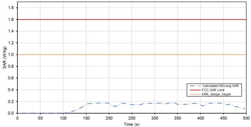
Total Time-Averaged SAR Test Sequence B Tech: 5GNR SUB6, n66, Ant B
