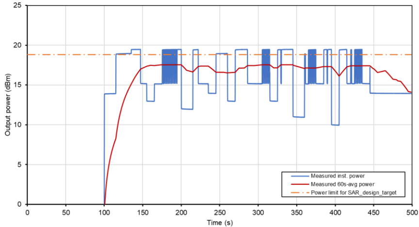
Time-Averaged Conducted Power Test Sequence B Tech: LTE, Band 48, Ant G
