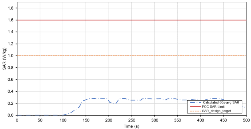
Total Time-Averaged SAR Test Sequence B Tech: GPRS, Band 1900
