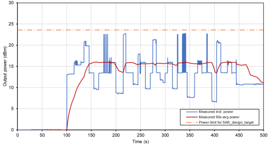
Time-Averaged Conducted Power Test Sequence B Tech: 5GNR SUB6, n41, Ant B
