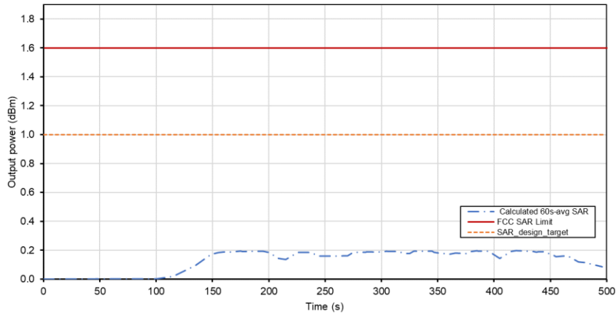
Total Time-Averaged SAR Test Sequence B Tech: WCDMA, Band 4
