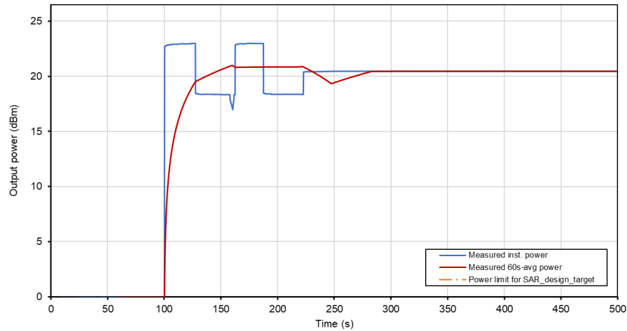
Time-Averaged Conducted Power Test Sequence A Tech: WCDMA, Band 4
