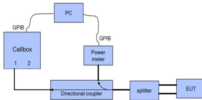
(b) Appendix A – Test Setup Photo 4, 6, 7, 8
