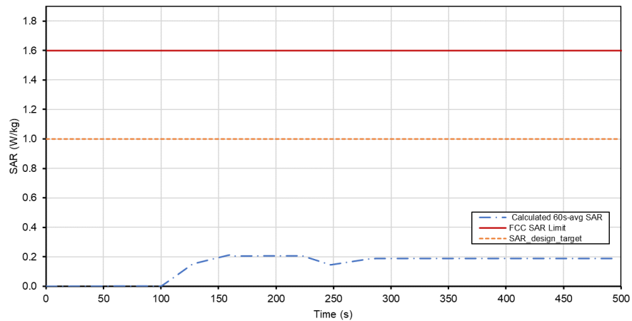
Total Time-Averaged SAR Test Sequence A Tech: WCDMA, Band 4
