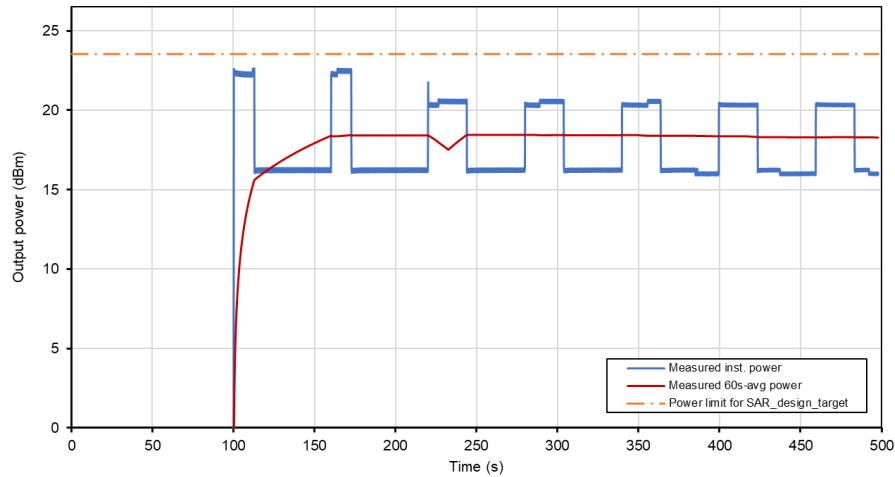
Time-Averaged Conducted Power Test Sequence A Tech: GPRS, Band 1900
