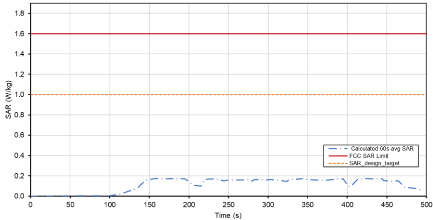
Total Time-Averaged SAR Test Sequence B Tech: 5GNR SUB6, n41, Ant B
