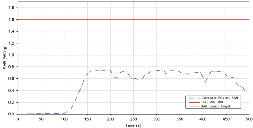
Total Time-Averaged SAR Test Sequence B Tech: LTE, Band 48, Ant G
