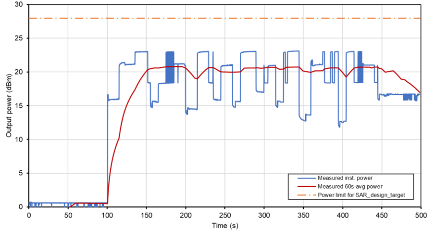
Time-Averaged Conducted Power Test Sequence B Tech: 5GNR SUB6, n66, Ant B
