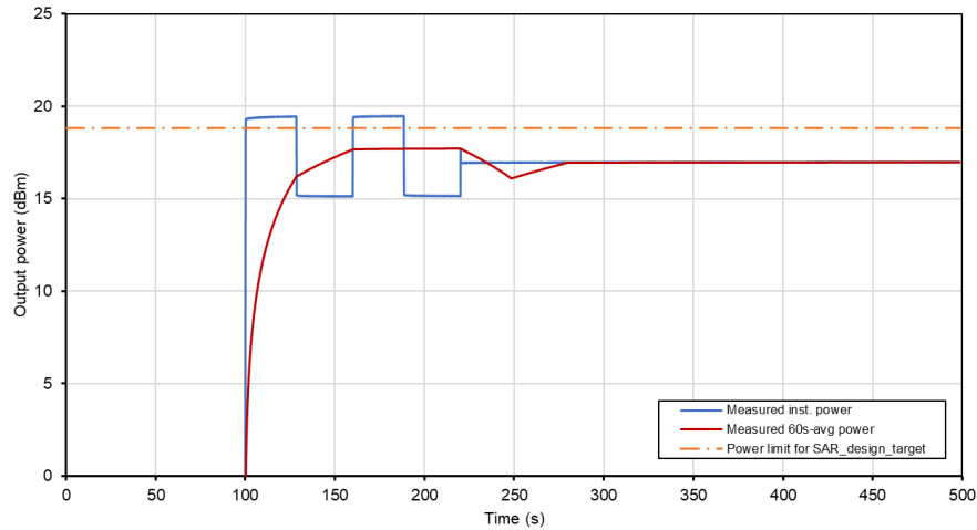
Time-Averaged Conducted Power Test Sequence A Tech: LTE, Band 48, Ant G
