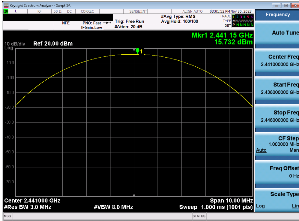
Plot 7-11. Peak Conducted Power (1Mbps – Ch. 39)
