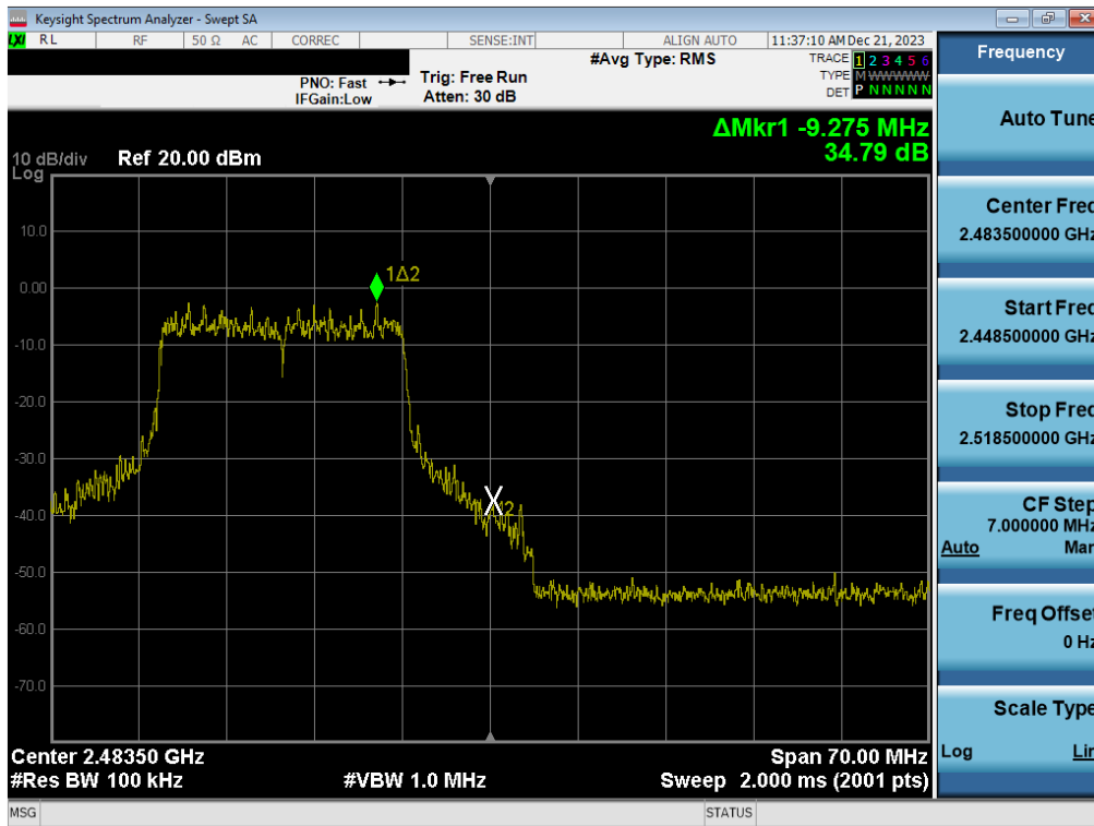
Plot 7-63. Band Edge Plot (802.11ax (2.4GHz) – Ch. 12) – MIMO ANT1
