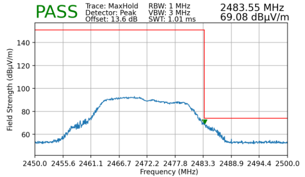
Plot 7-107. Radiated Restricted Upper Band Edge Measurement (Peak)
