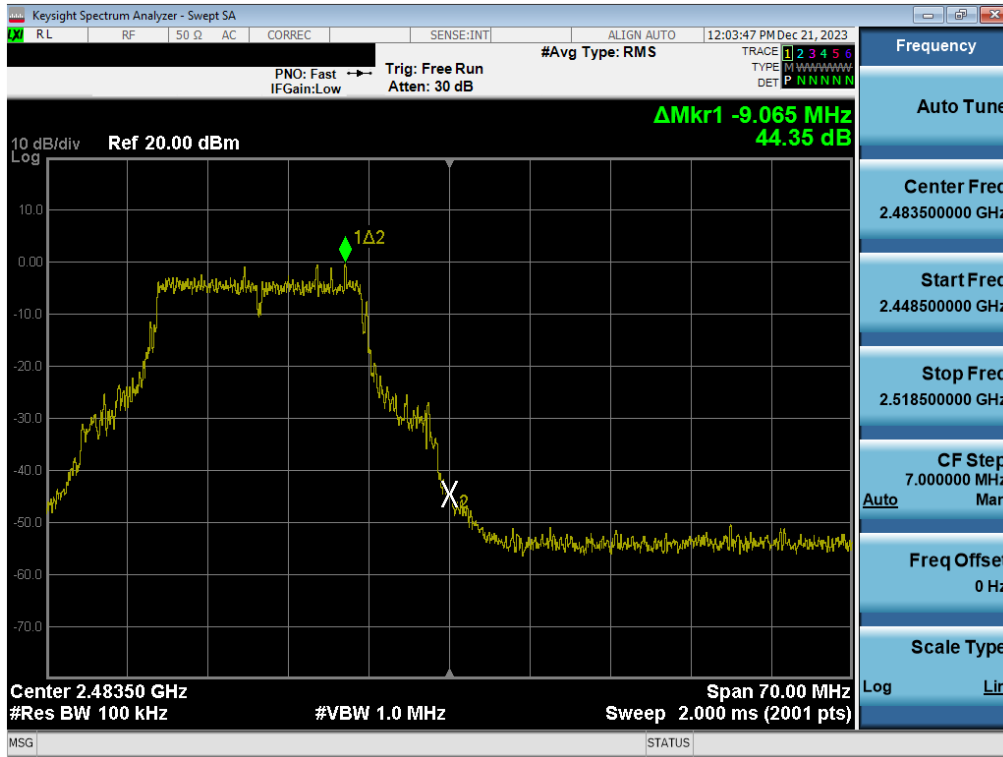
Plot 7-59. Band Edge Plot (802.11n (2.4GHz) – Ch. 12) – MIMO ANT1
