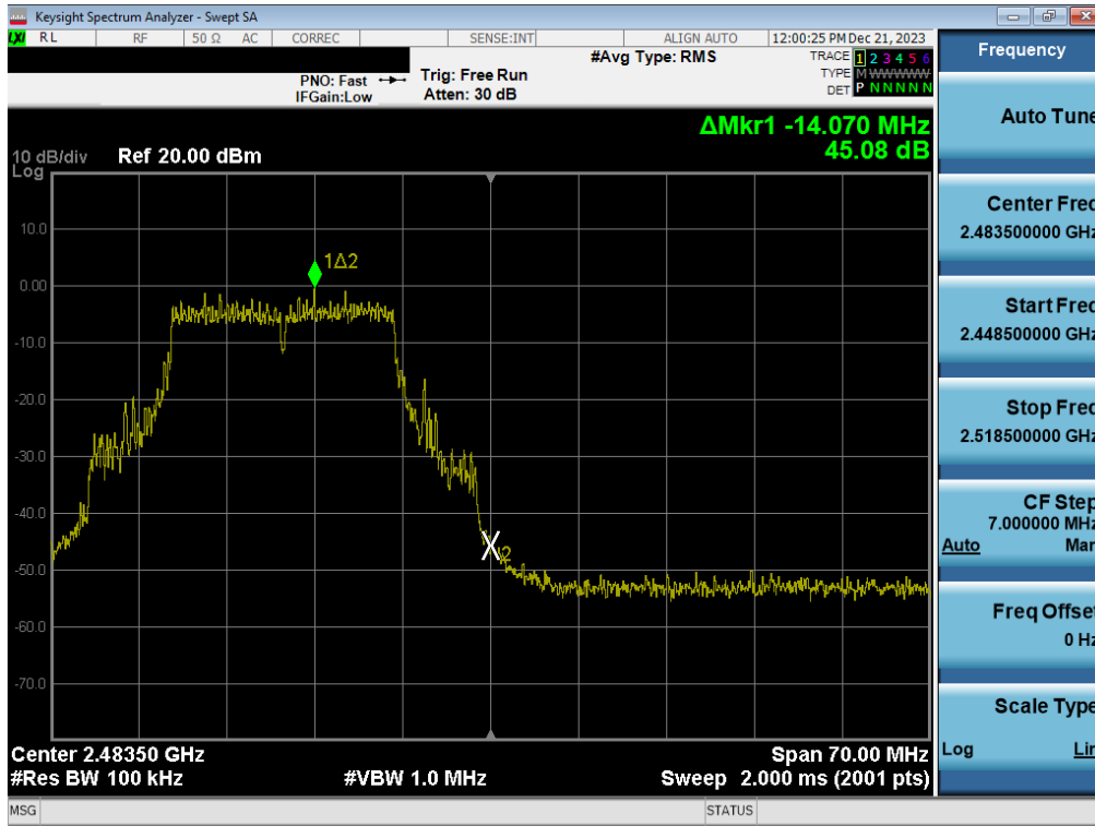
Plot 7-75. Band Edge Plot (802.11n (2.4GHz) – Ch. 12) – MIMO ANT2
