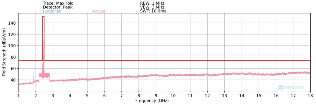
Plot 7-96. MIMO Radiated Spurious Plot above 1GHz (802.11b – Ch. 11)
