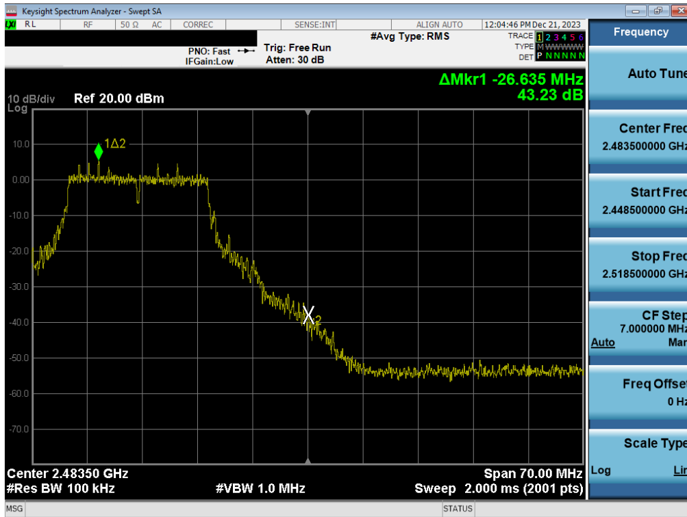
Plot 7-58. Band Edge Plot (802.11n (2.4GHz) – Ch. 11) – MIMO ANT1
