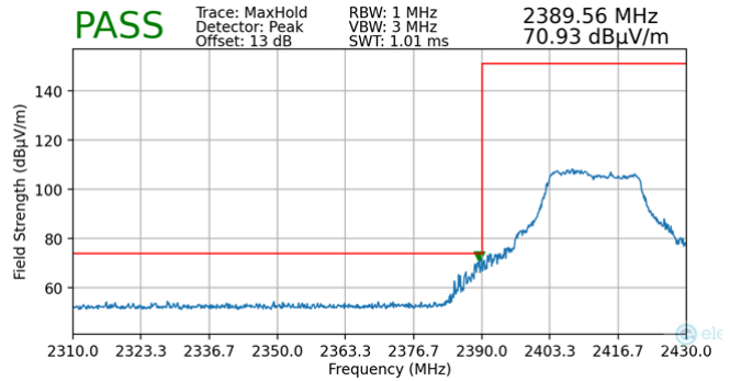
Plot 7-99. Radiated Restricted Lower Band Edge Measurement (Peak)
