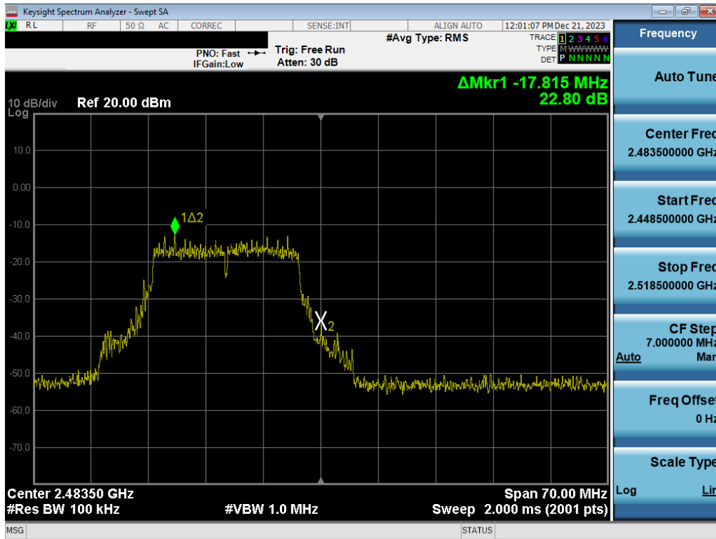
Plot 7-76. Band Edge Plot (802.11n (2.4GHz) – Ch. 13) – MIMO ANT2
