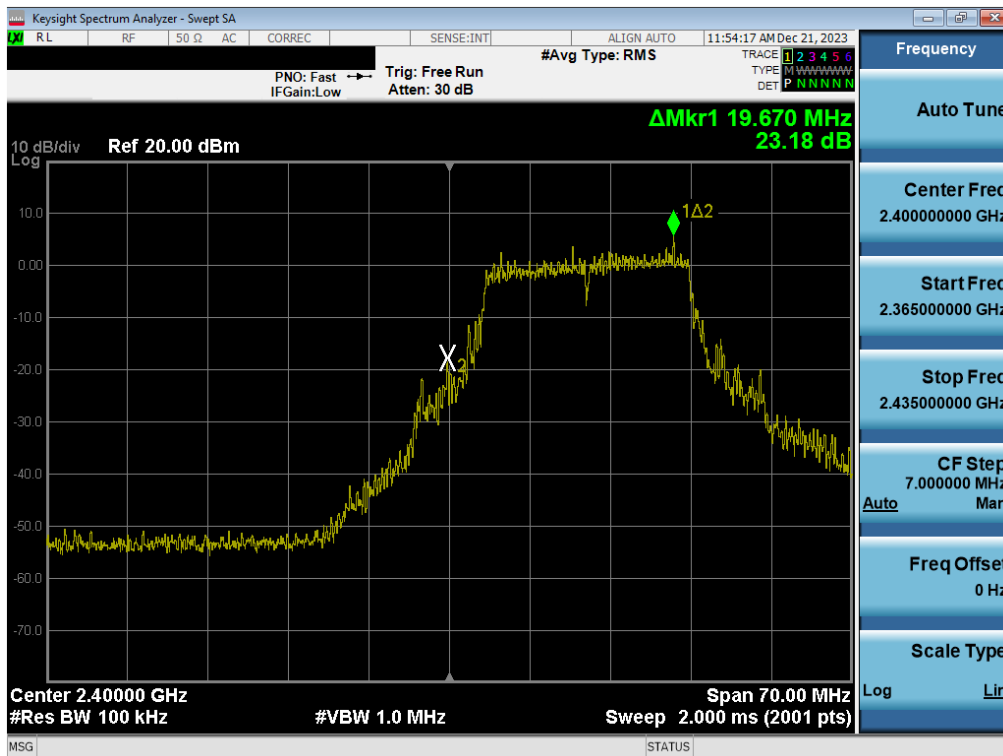
Plot 7-72. Band Edge Plot (802.11n (2.4GHz) – Ch. 1) – MIMO ANT2
