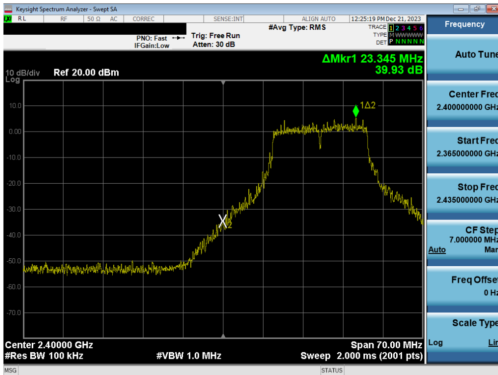
Plot 7-68. Band Edge Plot (802.11g- Ch. 2) – MIMO ANT2
