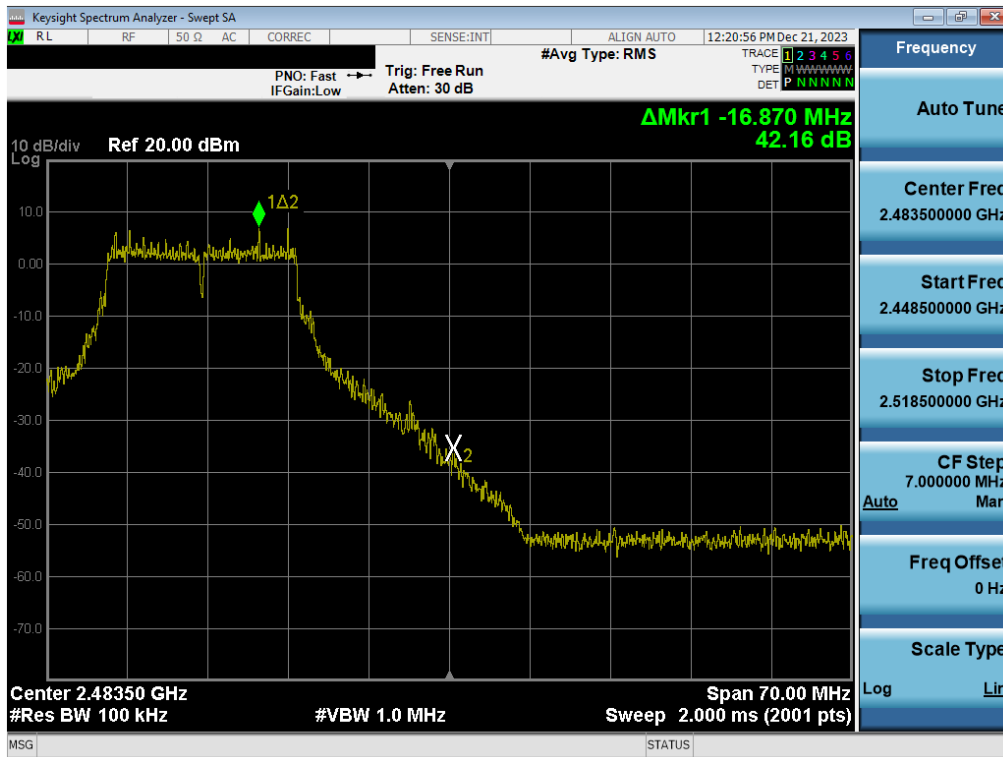
Plot 7-69. Band Edge Plot (802.11g – Ch. 11) – MIMO ANT2
