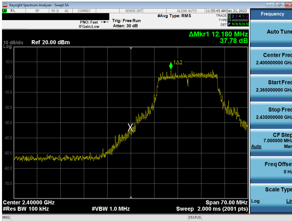
Plot 7-73. Band Edge Plot (802.11n (2.4GHz) – Ch. 2) – MIMO ANT2
