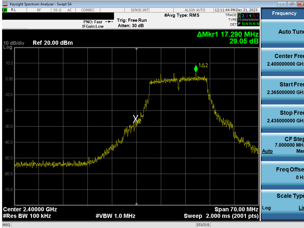
Plot 7-51. Band Edge Plot (802.11g- Ch. 1) – MIMO ANT1
