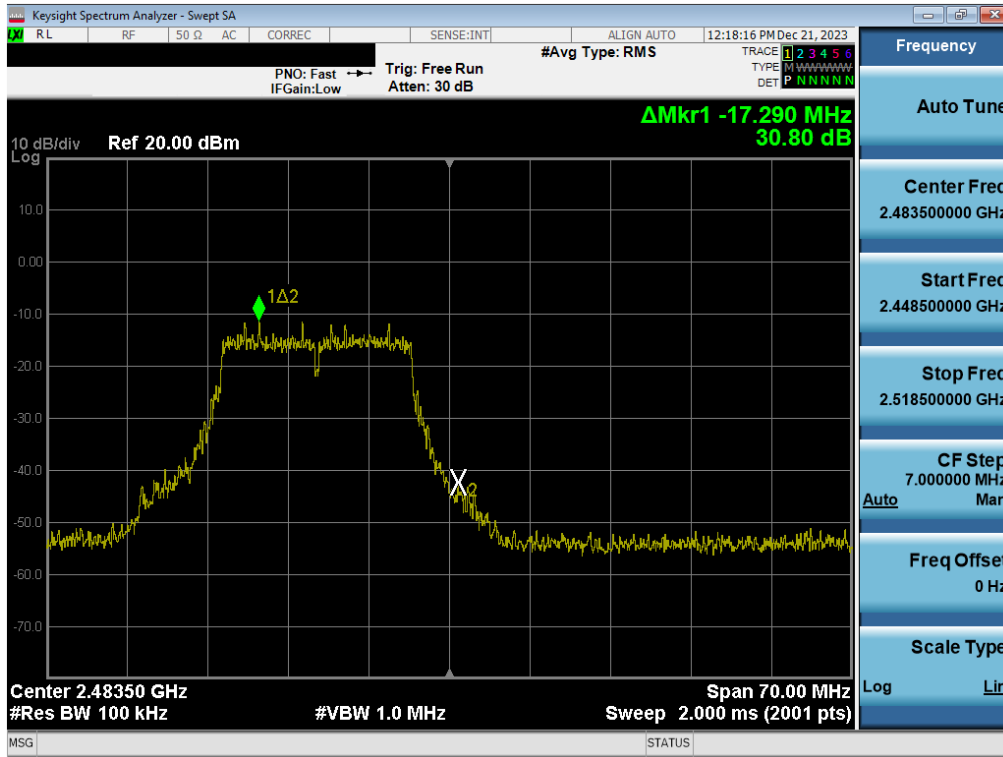
Plot 7-55. Band Edge Plot (802.11g – Ch. 13) – MIMO ANT1
