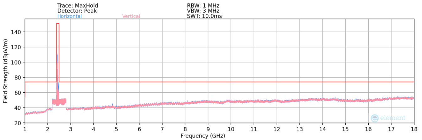
Plot 7-94. MIMO Radiated Spurious Plot above 1GHz (802.11b – Ch. 1)
