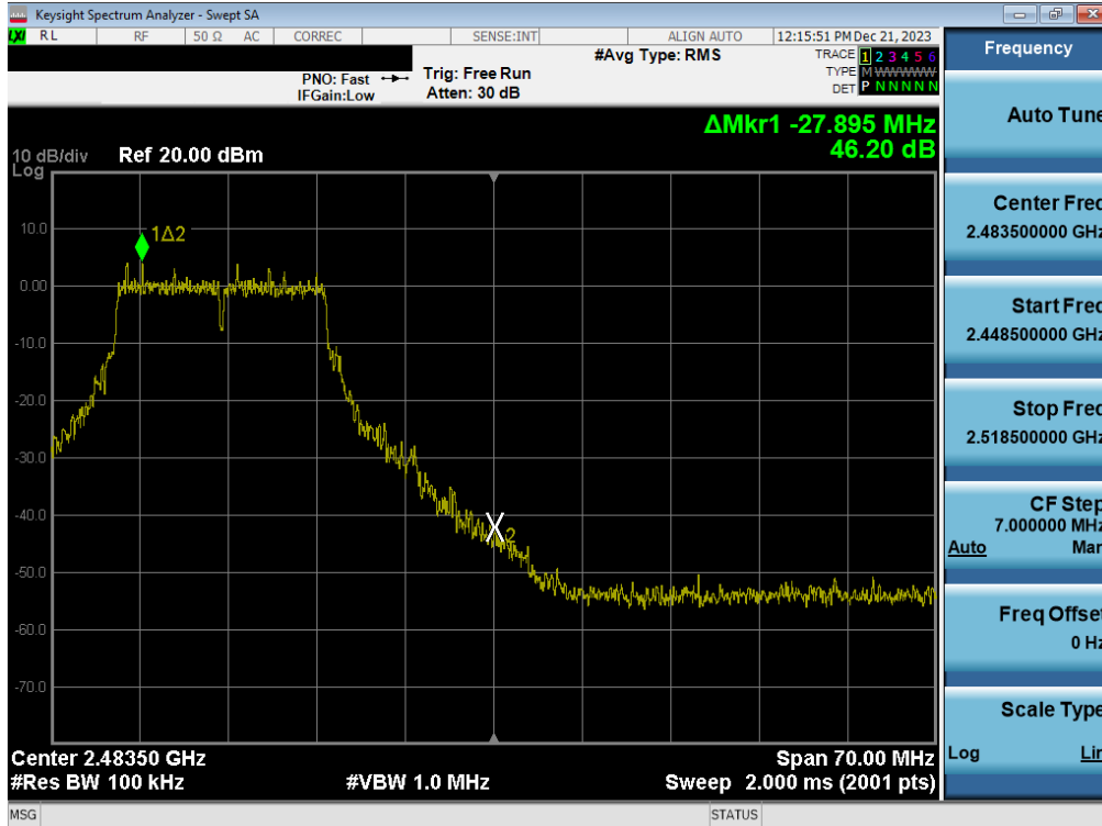
Plot 7-53. Band Edge Plot (802.11g - Ch. 11) - MIMO ANT1
