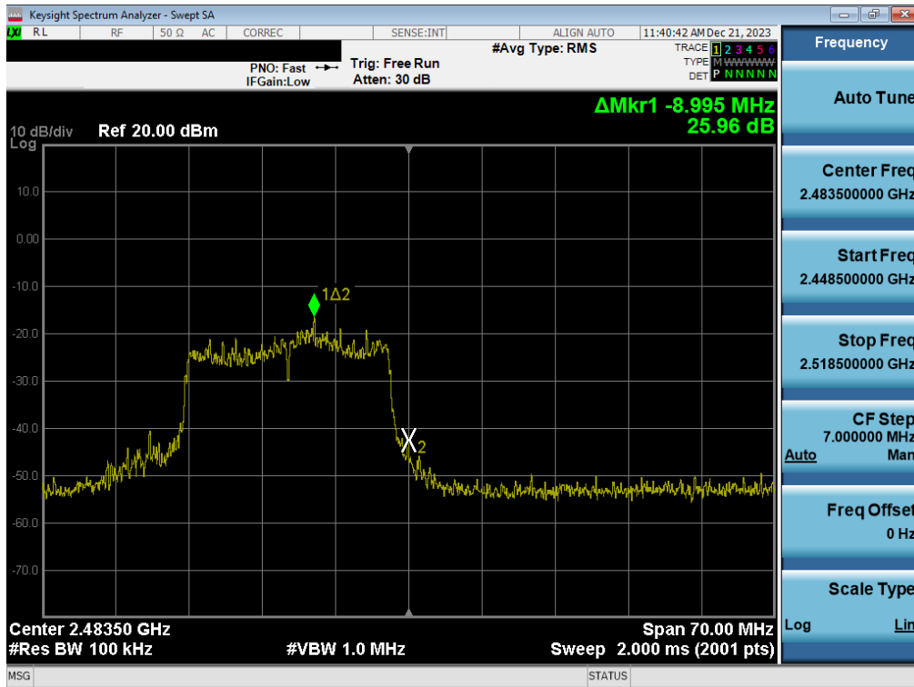
Plot 7-80. Band Edge Plot (802.11ax (2.4GHz) – Ch. 13) – MIMO ANT2
