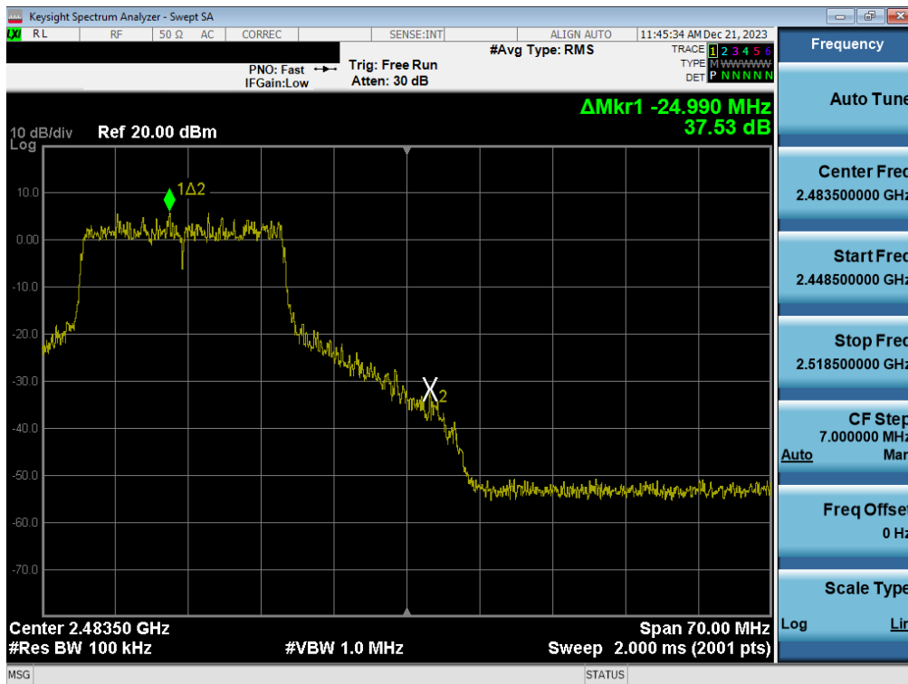
Plot 7-78. Band Edge Plot (802.11ax (2.4GHz) – Ch. 11) – MIMO ANT2
