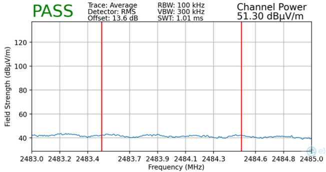
Plot 7-102. Radiated Restricted Upper Band Edge Measurement (Average)
