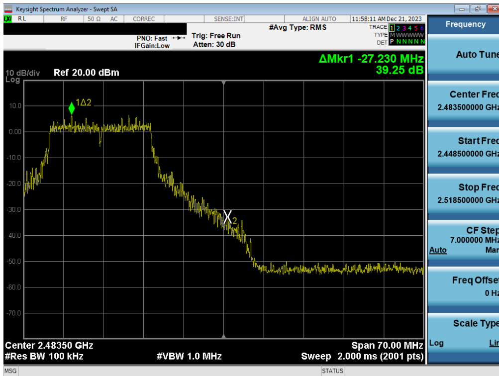
Plot 7-74. Band Edge Plot (802.11n (2.4GHz) – Ch. 11) – MIMO ANT2
