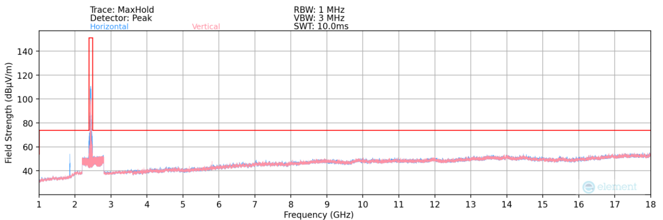
Plot 7-95. MIMO Radiated Spurious Plot above 1GHz (802.11b – Ch. 6)
