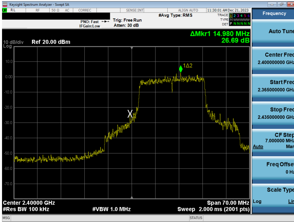
Plot 7-61. Band Edge Plot (802.11ax (2.4GHz) – Ch. 1) – MIMO ANT1
