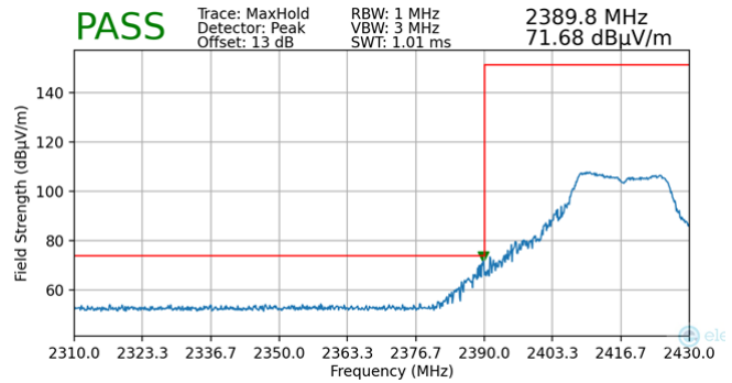
Plot 7-101. Radiated Restricted Lower Band Edge Measurement (Peak)
