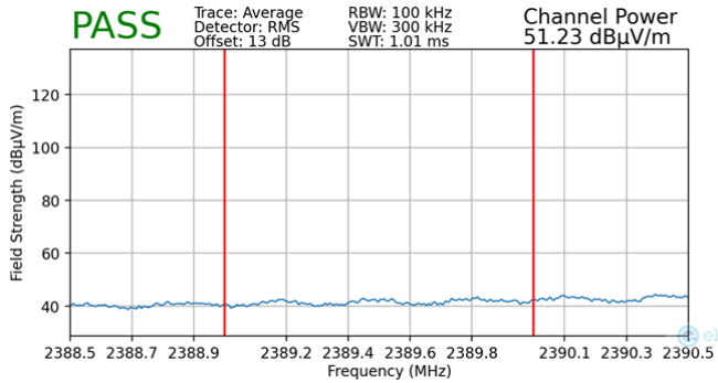
Plot 7-98. Radiated Restricted Lower Band Edge Measurement (Average)
