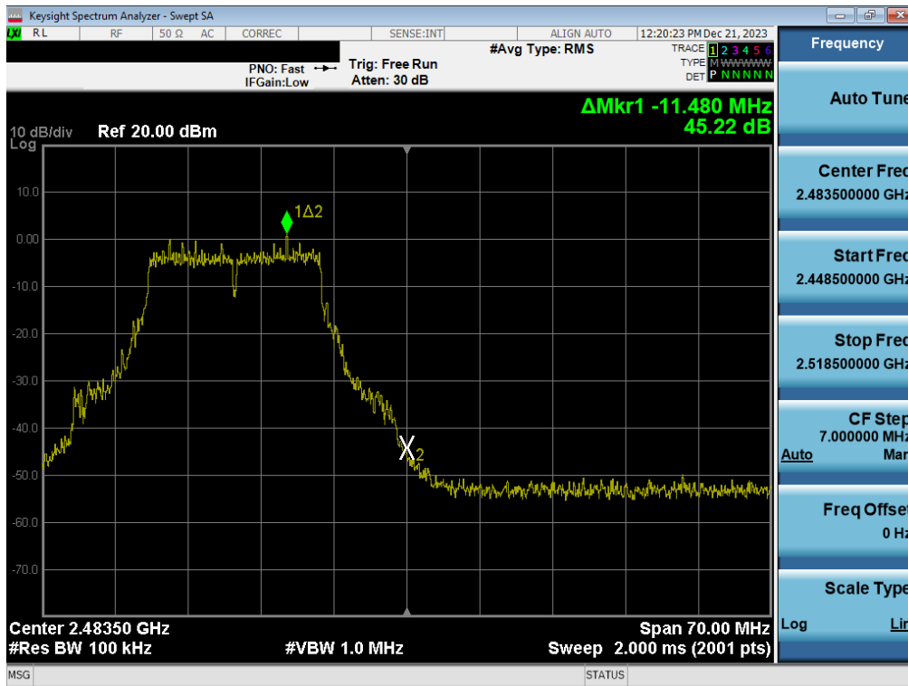
Plot 7-70. Band Edge Plot (802.11g – Ch. 12) – MIMO ANT2
