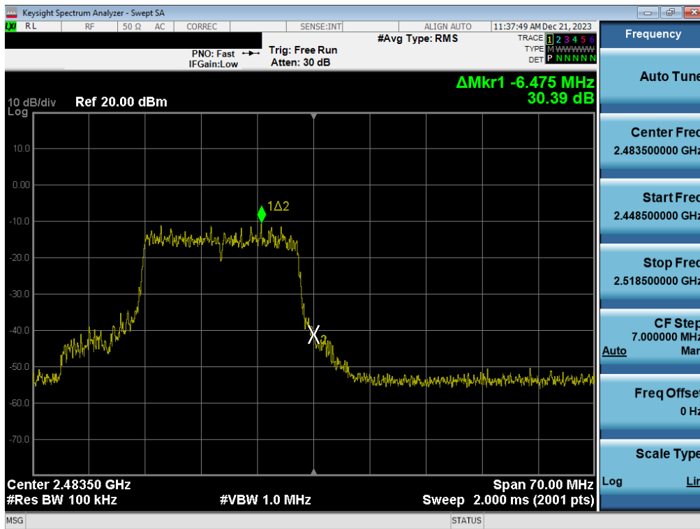
Plot 7-64. Band Edge Plot (802.11ax (2.4GHz) – Ch. 13) – MIMO ANT1
