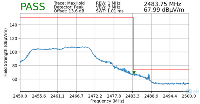
Plot 7-103. Radiated Restricted Upper Band Edge Measurement (Peak)
