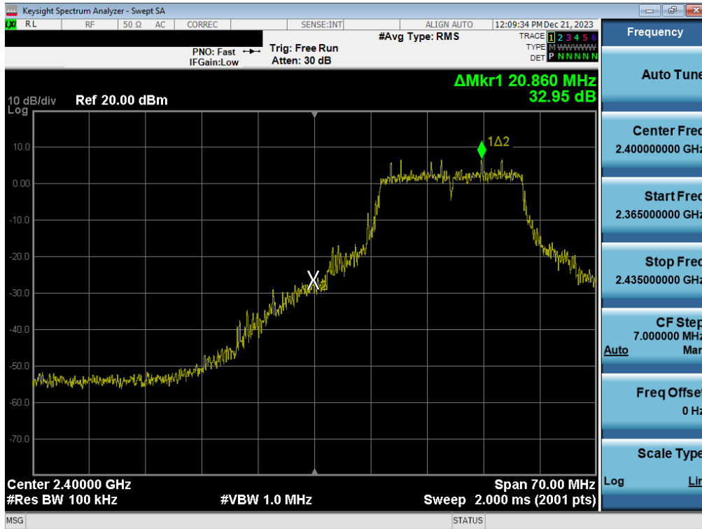
Plot 7-57. Band Edge Plot (802.11n (2.4GHz) – Ch. 2) – MIMO ANT1
