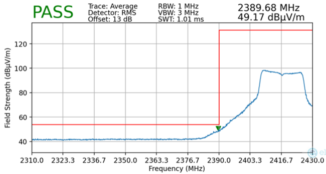
Plot 7-100. Radiated Restricted Lower Band Edge Measurement (Average)
