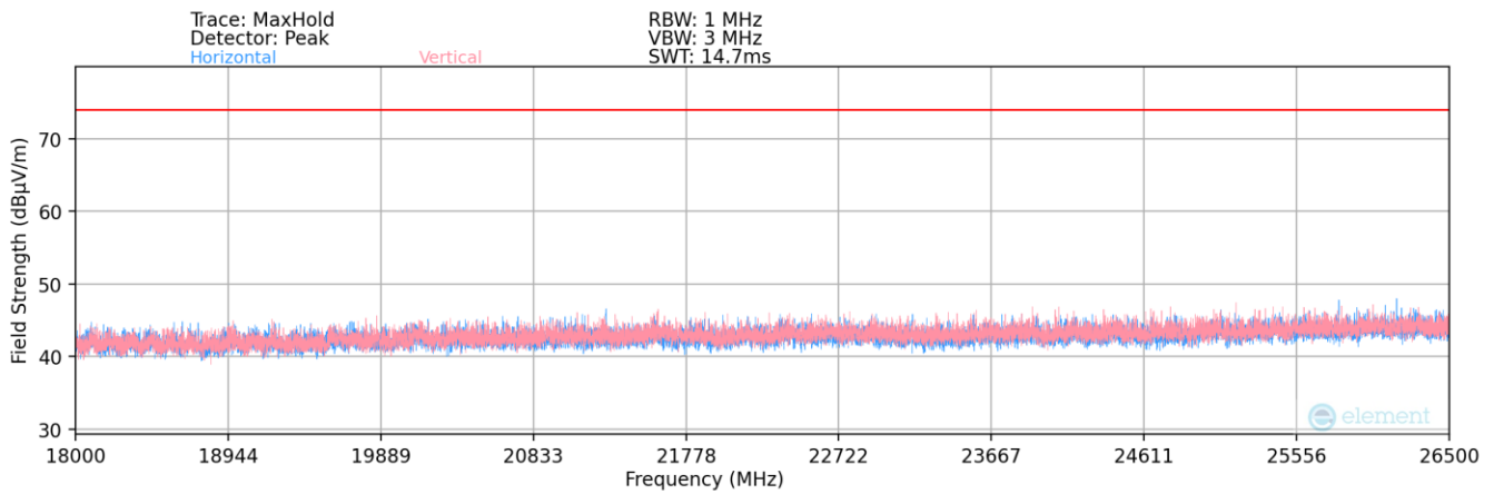
Plot 7-97. MIMO Radiated Spurious Plot above 18GHz
