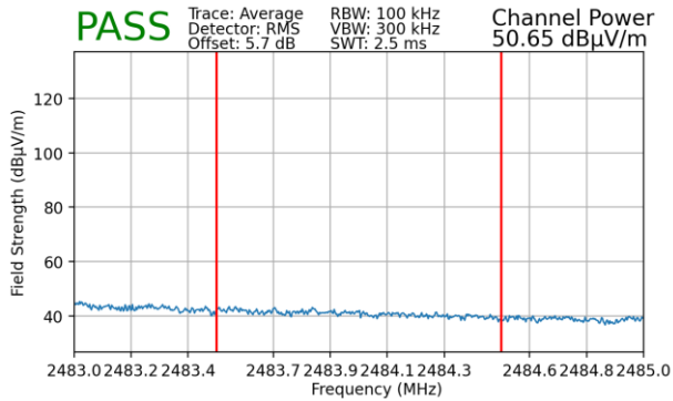
Plot 7-106. Radiated Restricted Upper Band Edge Measurement (Average)
