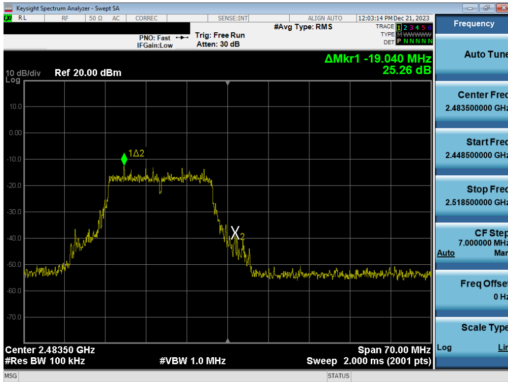
Plot 7-60. Band Edge Plot (802.11n (2.4GHz) – Ch. 13) – MIMO ANT1
