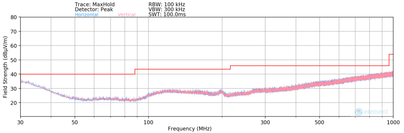
Plot 7-93. MIMO Radiated Spurious Plot below 1GHz ANT1
