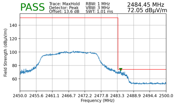
Plot 7-105. Radiated Restricted Upper Band Edge Measurement (Peak)
