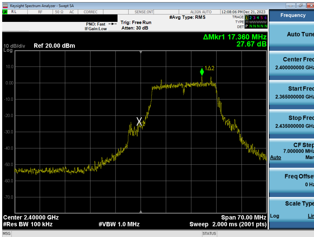
Plot 7-56. Band Edge Plot (802.11n (2.4GHz) – Ch. 1) – MIMO ANT1
