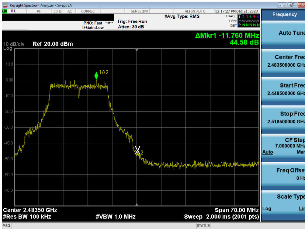
Plot 7-54. Band Edge Plot (802.11g - Ch. 12) - MIMO ANT1
