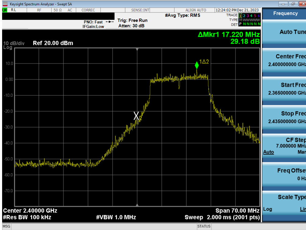
Plot 7-67. Band Edge Plot (802.11g- Ch. 1) – MIMO ANT2
