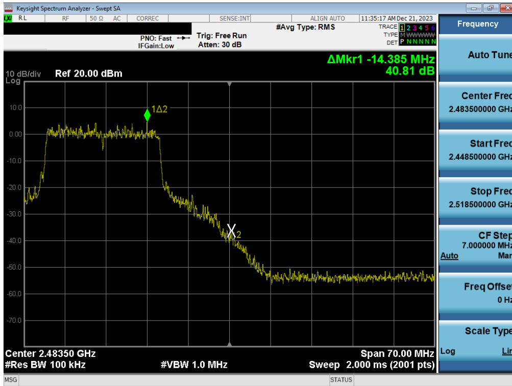
Plot 7-62. Band Edge Plot (802.11ax (2.4GHz) – Ch. 11) – MIMO ANT1
