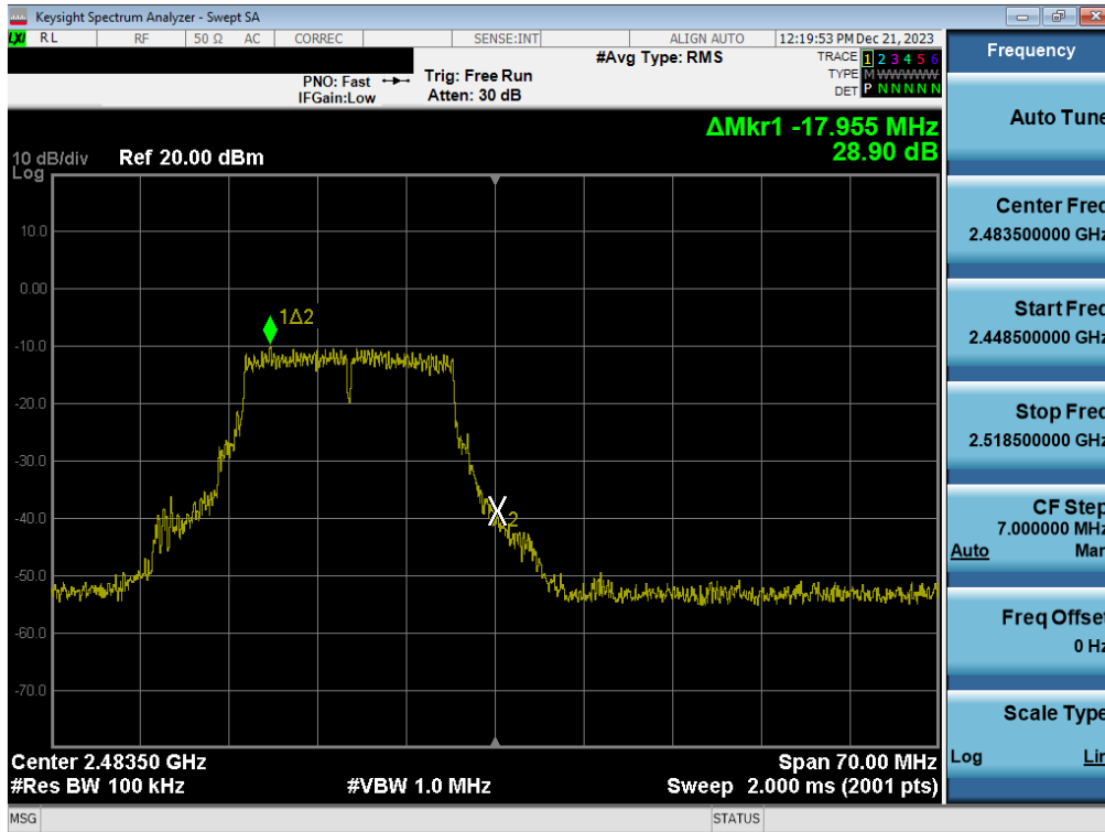
Plot 7-71. Band Edge Plot (802.11g – Ch. 13) – MIMO ANT2
