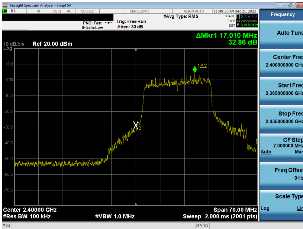
Plot 7-77. Band Edge Plot (802.11ax (2.4GHz) – Ch. 1) – MIMO ANT2
