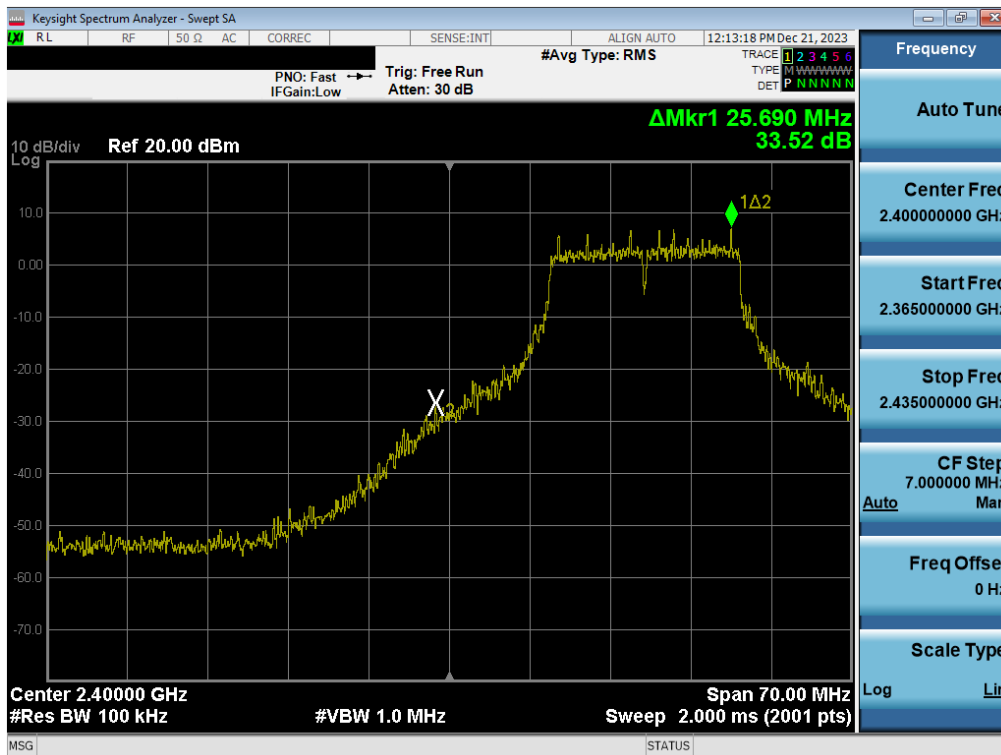
Plot 7-52. Band Edge Plot (802.11g- Ch. 2) – MIMO ANT1
