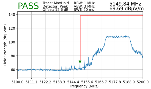
Plot 7-117. Radiated Lower Band Edge Plot MIMO (Peak – UNII Band 1 – 242 Tones)
