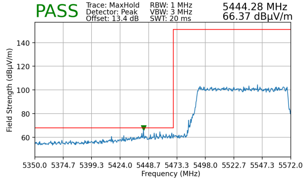
Plot 7-135. Radiated Lower Band Edge Plot MIMO (Peak – UNII Band 2C – 996 Tones)
