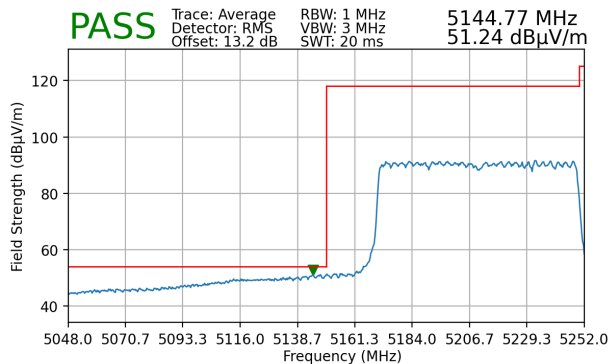
Plot 7-130. Radiated Lower Band Edge Plot MIMO (Average – UNII Band 1 – 996 Tones)
