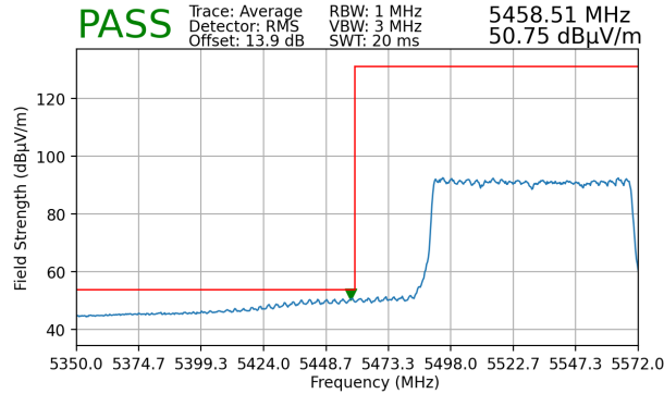
Plot 7-134. Radiated Lower Band Edge Plot MIMO (Average – UNII Band 2C – 996 Tones)
