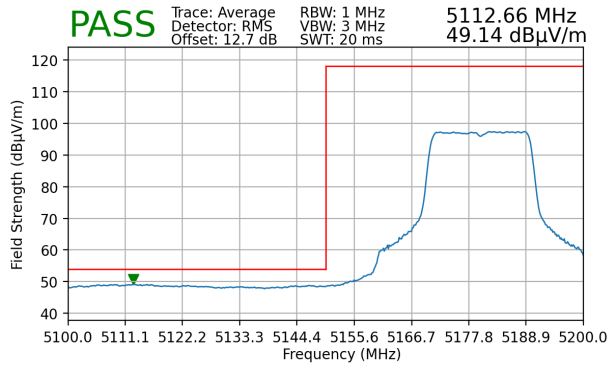
Plot 7-116. Radiated Lower Band Edge Plot MIMO (Average – UNII Band 1 – 242 Tones)
