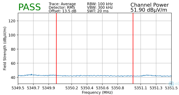
Plot 7-125. Radiated Upper Band Edge Plot MIMO (Average – UNII Band 2A – 484 Tones)
