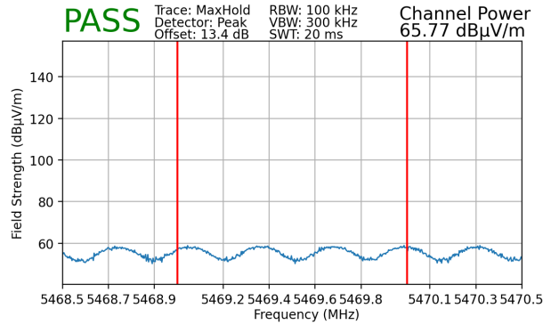
Plot 7-128. Radiated Lower Band Edge Plot MIMO (Peak – UNII Band 2C – 484 Tones)
