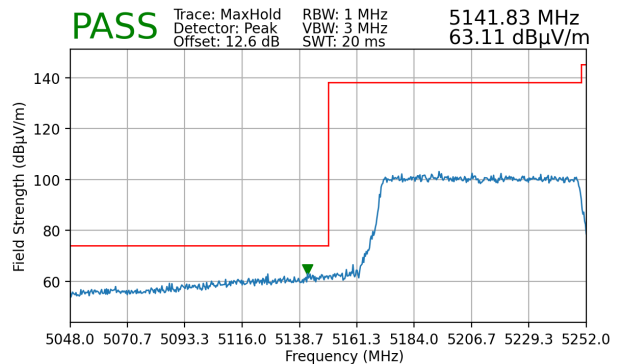
Plot 7-131. Radiated Lower Band Edge Plot MIMO (Peak – UNII Band 1 – 996 Tones)
