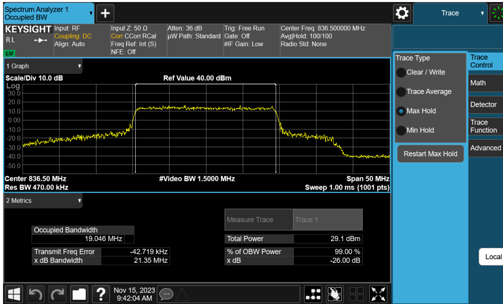
Plot 7-13. Occupied Bandwidth Plot (NR Band n5 - 20MHz 16-QAM - Full RB)
