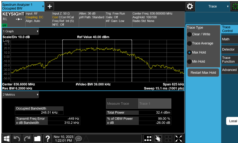
Plot 7-24. Occupied Bandwidth Plot (EDGE, Ch. 190)
