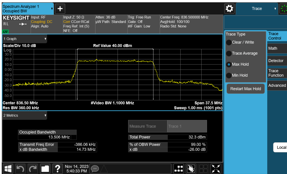
Plot 7-14. Occupied Bandwidth Plot (NR Band n5 - 15MHz \pi/2 BPSK - Full RB)
