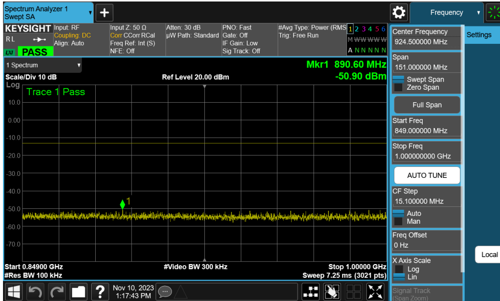
Plot 7-33. Conducted Spurious Plot (GPRS Ch. 190)
