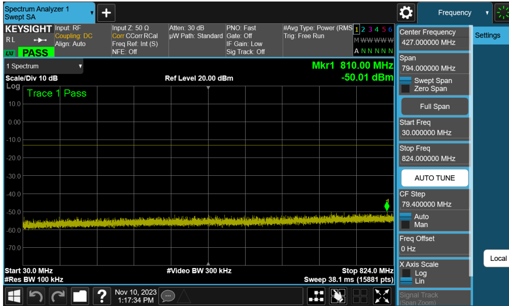
Plot 7-32. Conducted Spurious Plot (GPRS Ch. 190)
