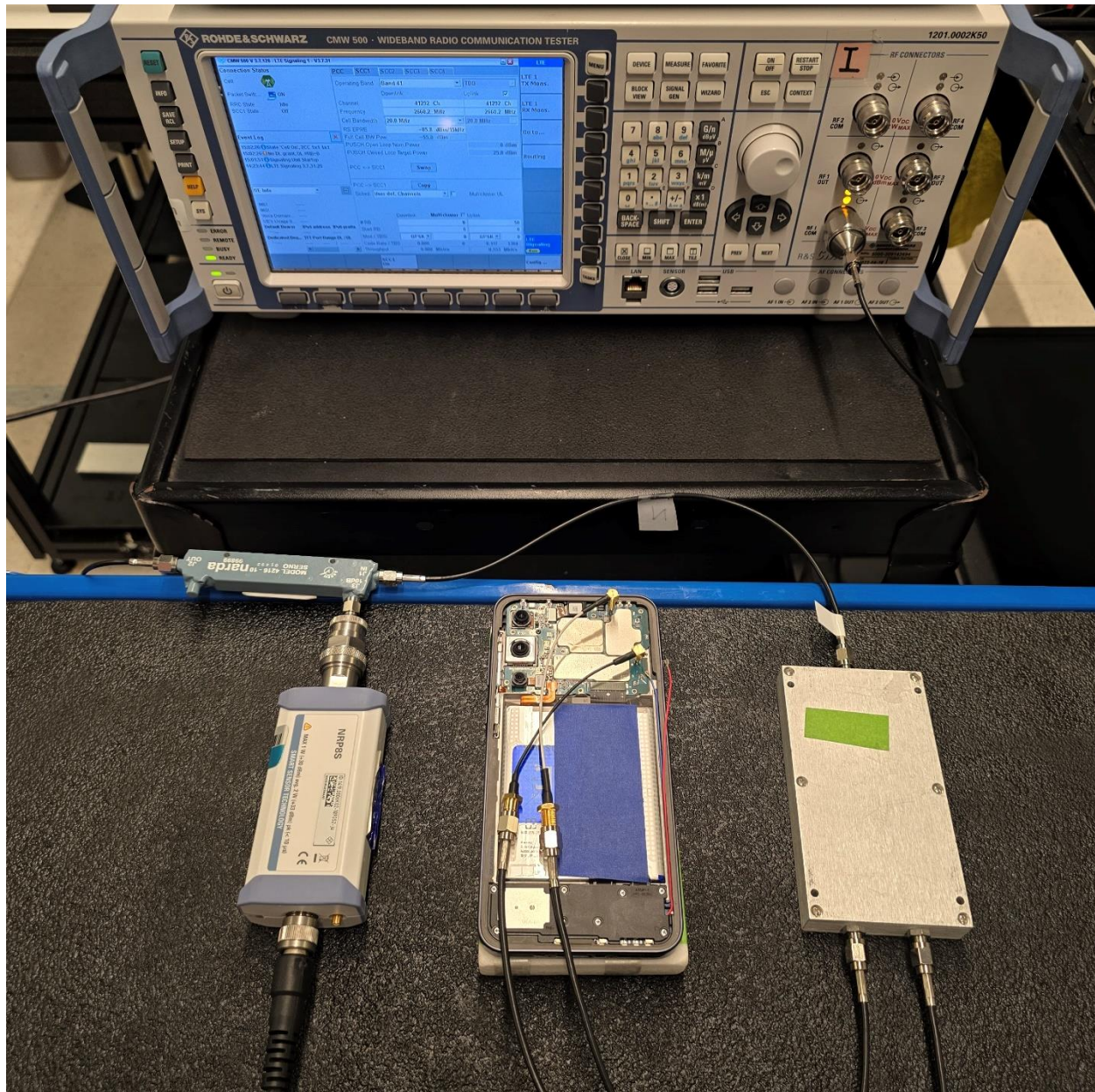
Test Setup Photo 5 - Conducted Test Setup (Figure 6-1b)
