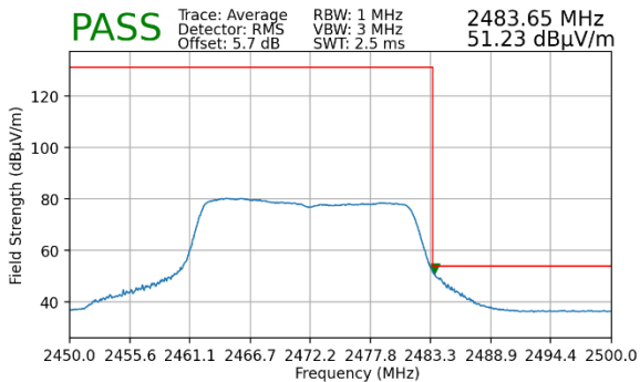
Plot 7-87. Radiated Restricted Upper Band Edge Measurement MIMO (Average – 242 Tones)
