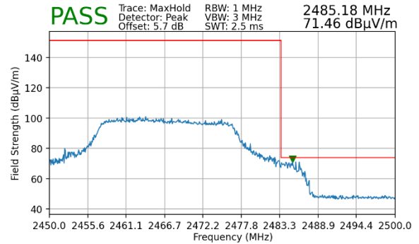
Plot 7-86. Radiated Restricted Upper Band Edge Measurement MIMO (Peak – 242 Tones)
