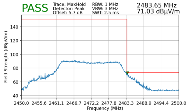
Plot 7-88. Radiated Restricted Upper Band Edge Measurement MIMO (Peak – 242 Tones)
