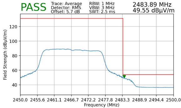
Plot 7-85. Radiated Restricted Upper Band Edge Measurement MIMO (Average – 242 Tones)
