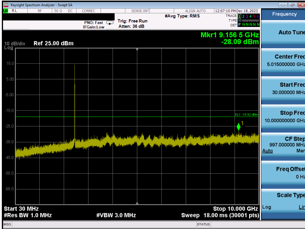
Plot 7-91. Conducted Spurious Plot (802.11b – Ch. 11) – MIMO ANT1
