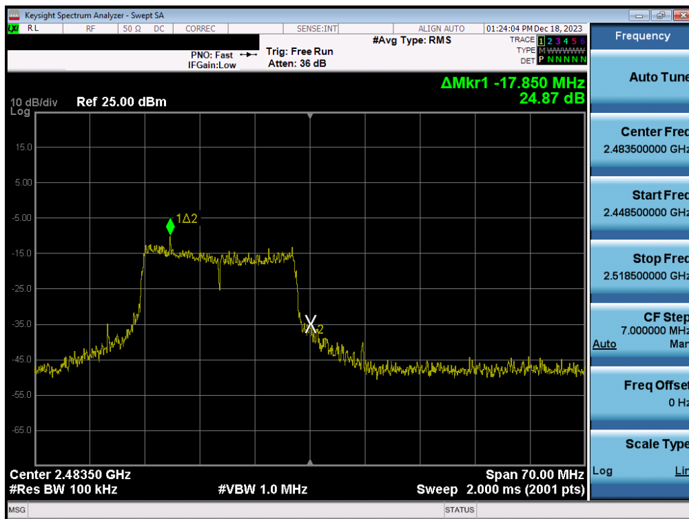
Plot 7-86. Band Edge Plot (802.11ax (2.4GHz) – Ch. 13) – MIMO ANT2
