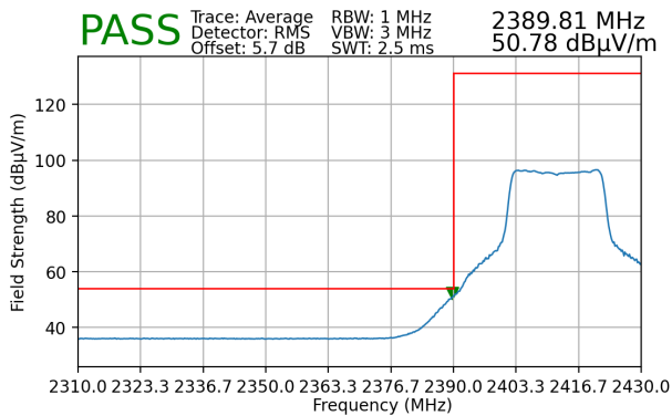
Plot 7-104. Radiated Restricted Lower Band Edge Measurement (Average)
