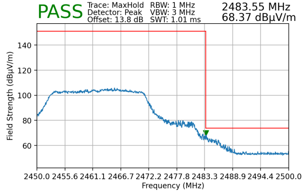
Plot 7-109. Radiated Restricted Upper Band Edge Measurement (Peak)
