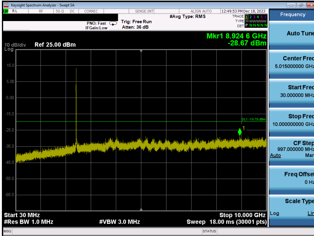
Plot 7-95. Conducted Spurious Plot (802.11b – Ch. 6) – MIMO ANT2
