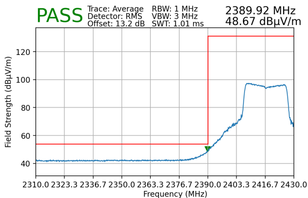
Plot 7-106. Radiated Restricted Lower Band Edge Measurement (Average)
