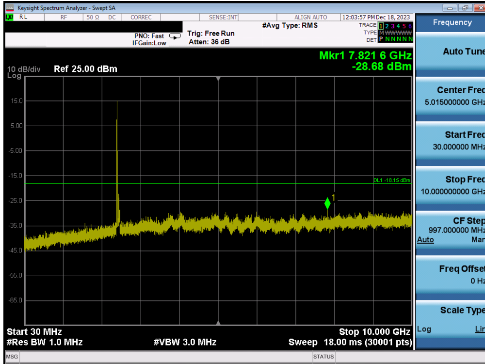
Plot 7-87. Conducted Spurious Plot (802.11b – Ch. 1) – MIMO ANT1
