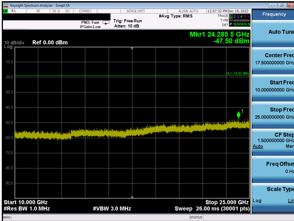
Plot 7-92. Conducted Spurious Plot (802.11b – Ch. 11) – MIMO ANT1
