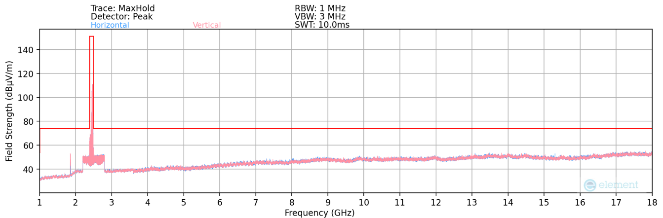
Plot 7-102. MIMO Radiated Spurious Plot above 1GHz (802.11b – Ch. 11)
