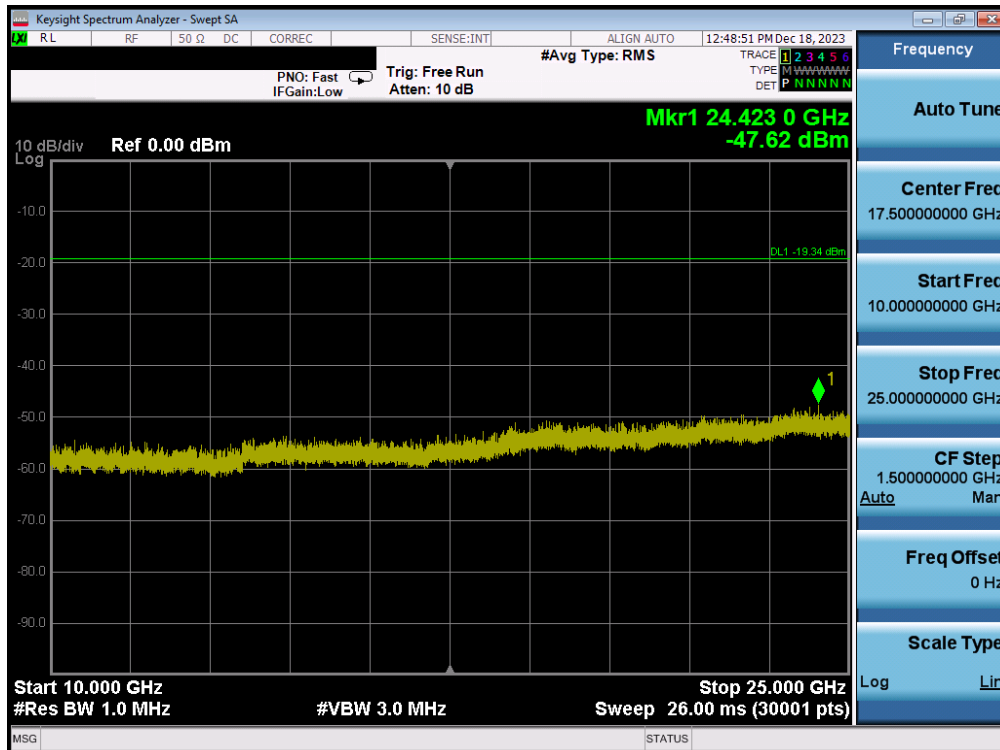
Plot 7-94. Conducted Spurious Plot (802.11b – Ch. 1) – MIMO ANT2
