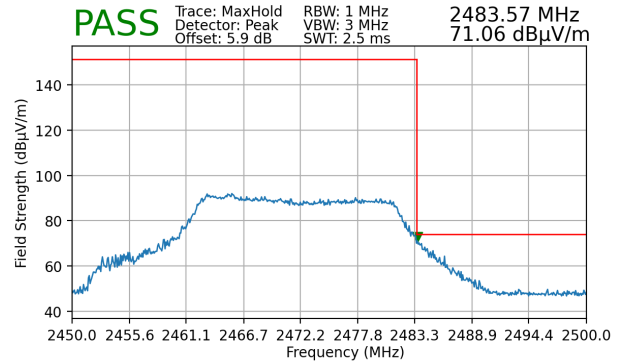
Plot 7-113. Radiated Restricted Upper Band Edge Measurement (Peak)
