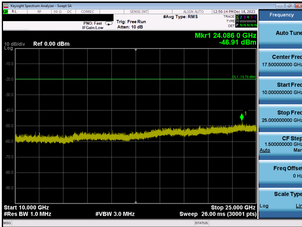
Plot 7-96. Conducted Spurious Plot (802.11b – Ch. 6) – MIMO ANT2
