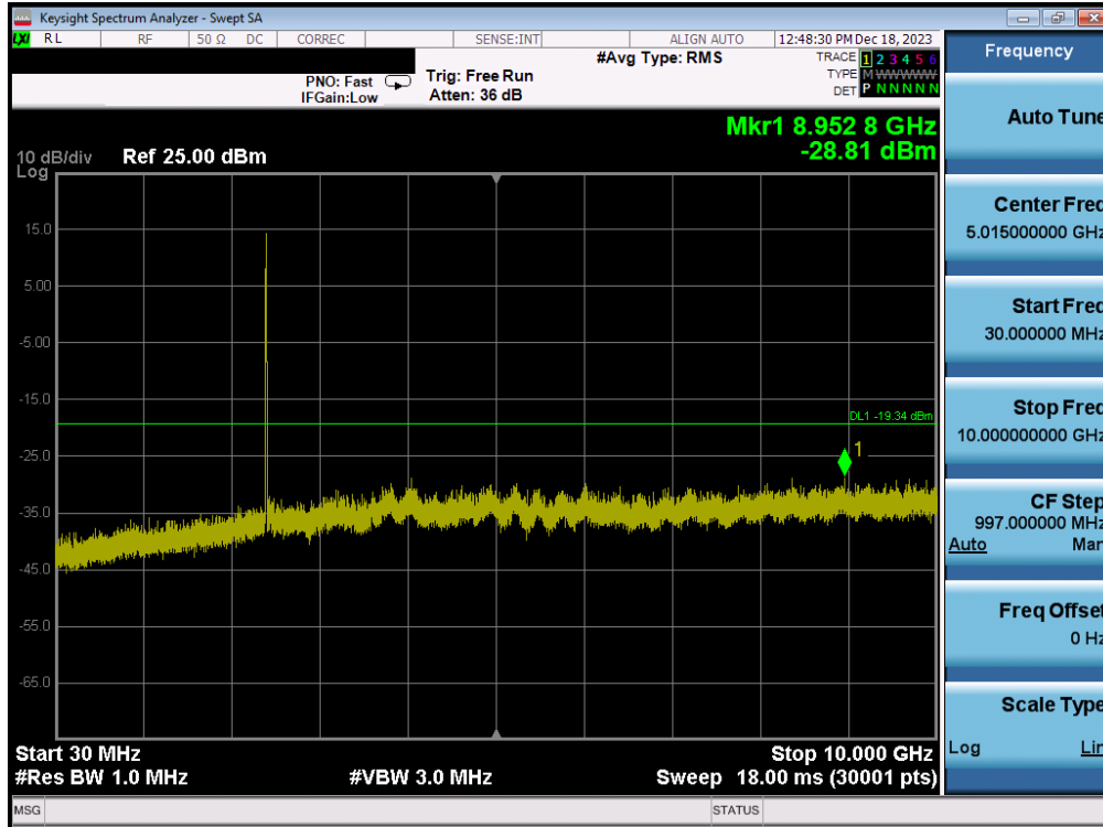
Plot 7-93. Conducted Spurious Plot (802.11b – Ch. 1) – MIMO ANT2
