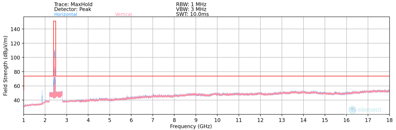
Plot 7-101. MIMO Radiated Spurious Plot above 1GHz (802.11b – Ch. 6)
