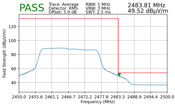
Plot 7-110. Radiated Restricted Upper Band Edge Measurement (Average)
