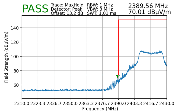
Plot 7-107. Radiated Restricted Lower Band Edge Measurement (Peak)
