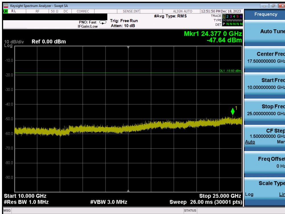
Plot 7-98. Conducted Spurious Plot (802.11b – Ch. 11) – MIMO ANT2
