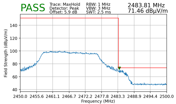
Plot 7-111. Radiated Restricted Upper Band Edge Measurement (Peak)
