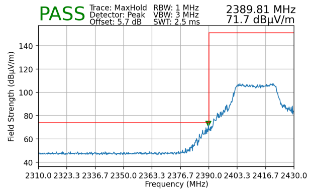
Plot 7-105. Radiated Restricted Lower Band Edge Measurement (Peak)
