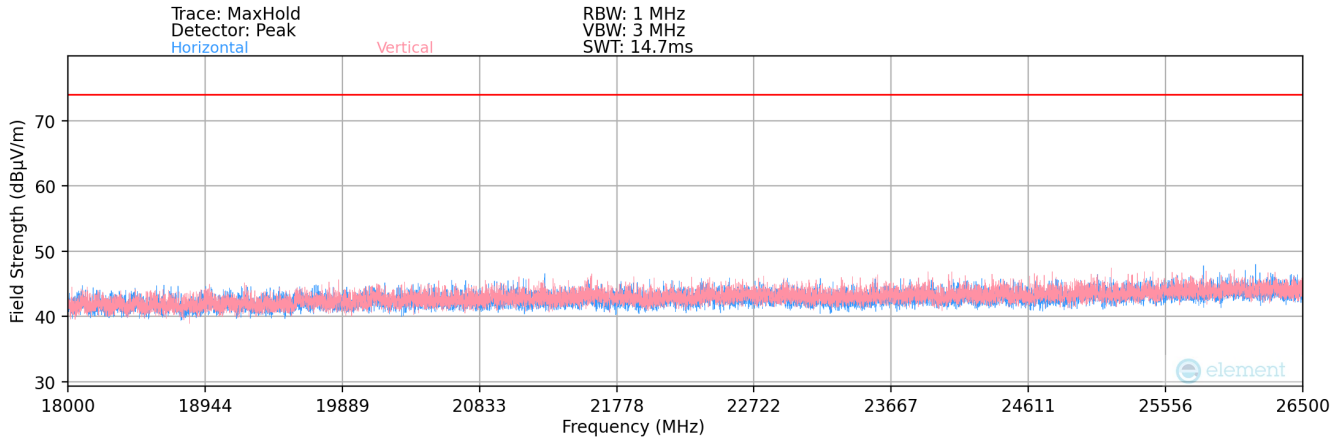
Plot 7-103. MIMO Radiated Spurious Plot above 18GHz
