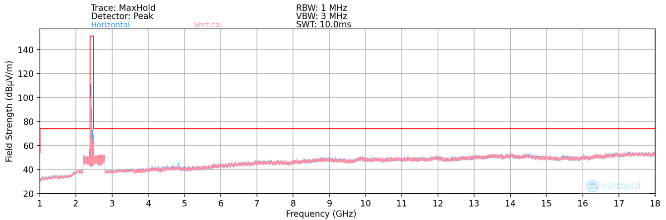
Plot 7-100. MIMO Radiated Spurious Plot above 1GHz (802.11b – Ch. 1)
