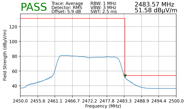
Plot 7-112. Radiated Restricted Upper Band Edge Measurement (Average)
