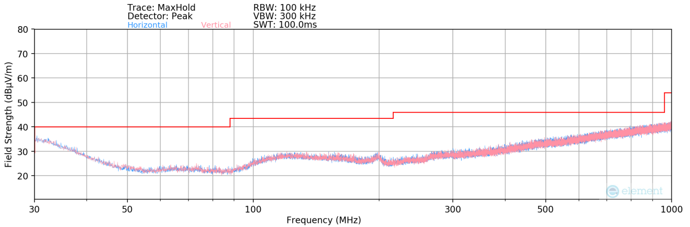
Plot 7-99. MIMO Radiated Spurious Plot below 1GHz
