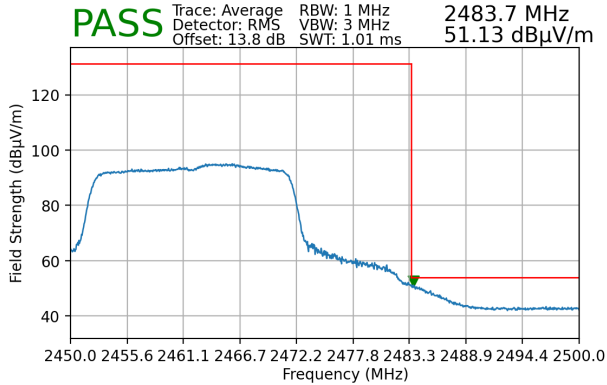
Plot 7-108. Radiated Restricted Upper Band Edge Measurement (Average)
