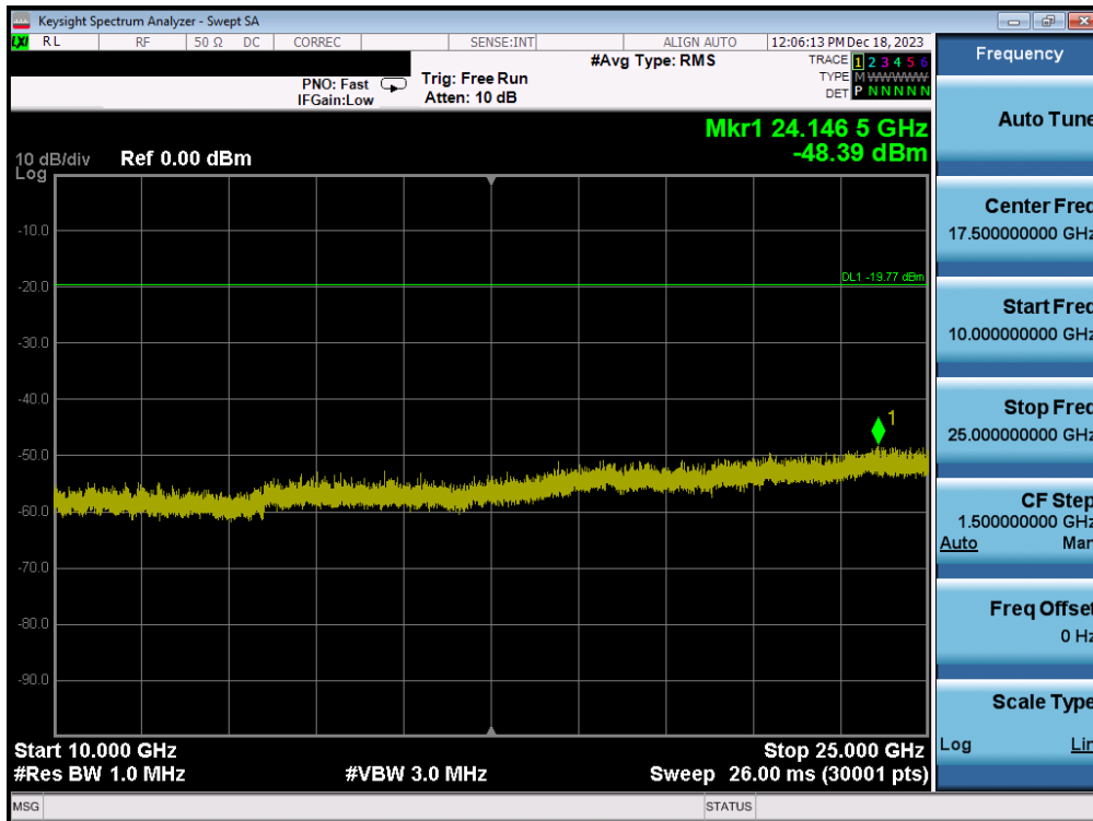
Plot 7-90. Conducted Spurious Plot (802.11b – Ch. 6) – MIMO ANT1
