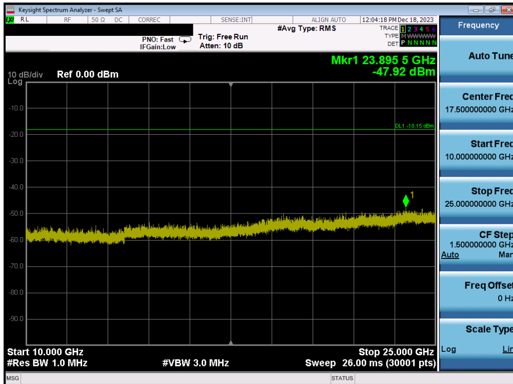
Plot 7-88. Conducted Spurious Plot (802.11b – Ch. 1) – MIMO ANT1
