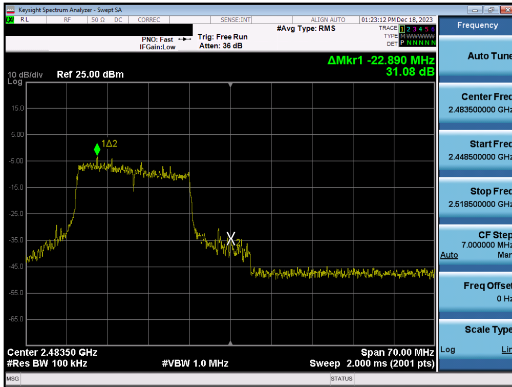
Plot 7-85. Band Edge Plot (802.11ax (2.4GHz) – Ch. 12) – MIMO ANT2
