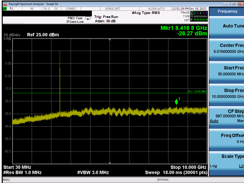
Plot 7-97. Conducted Spurious Plot (802.11b – Ch. 11) – MIMO ANT2
