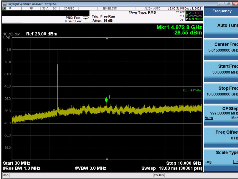
Plot 7-89. Conducted Spurious Plot (802.11b – Ch. 6) – MIMO ANT1
