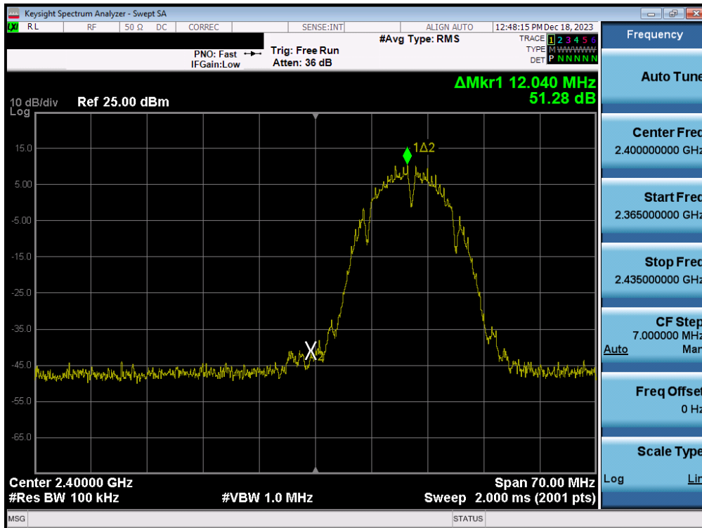
Plot 7-68. Band Edge Plot (802.11b – Ch. 1) – MIMO ANT2
