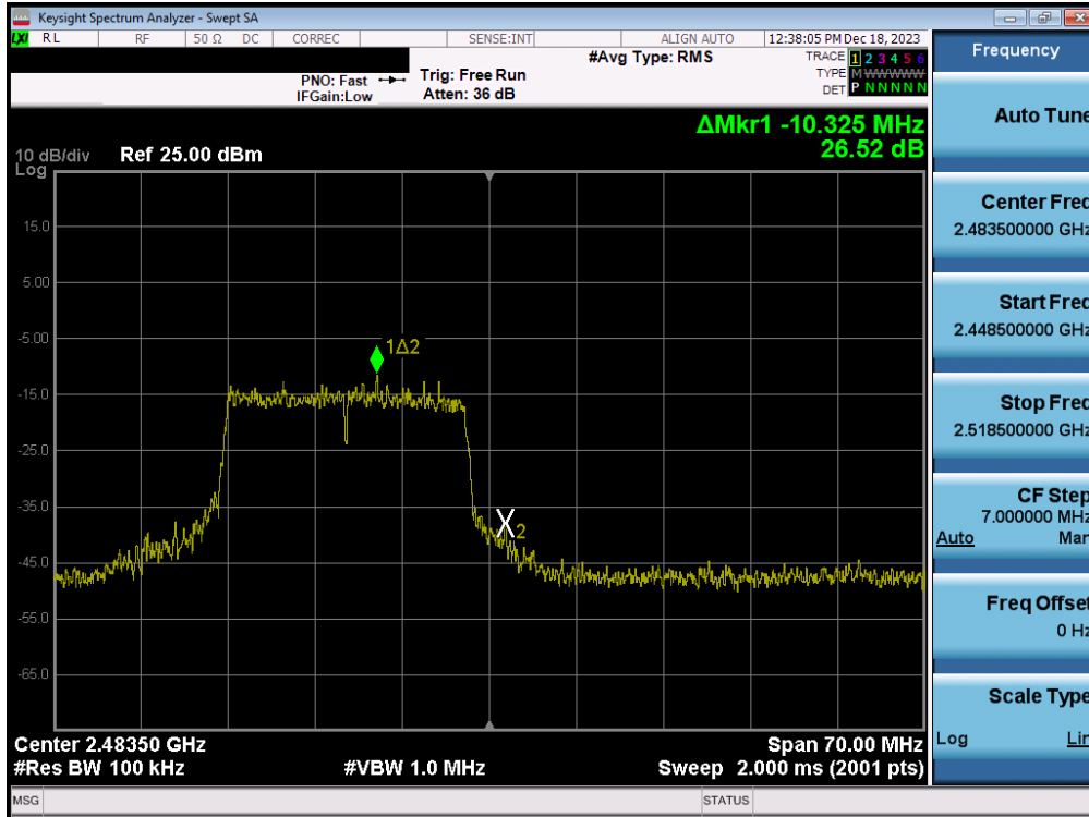
Plot 7-67. Band Edge Plot (802.11ax (2.4GHz) – Ch. 13) – MIMO ANT1
