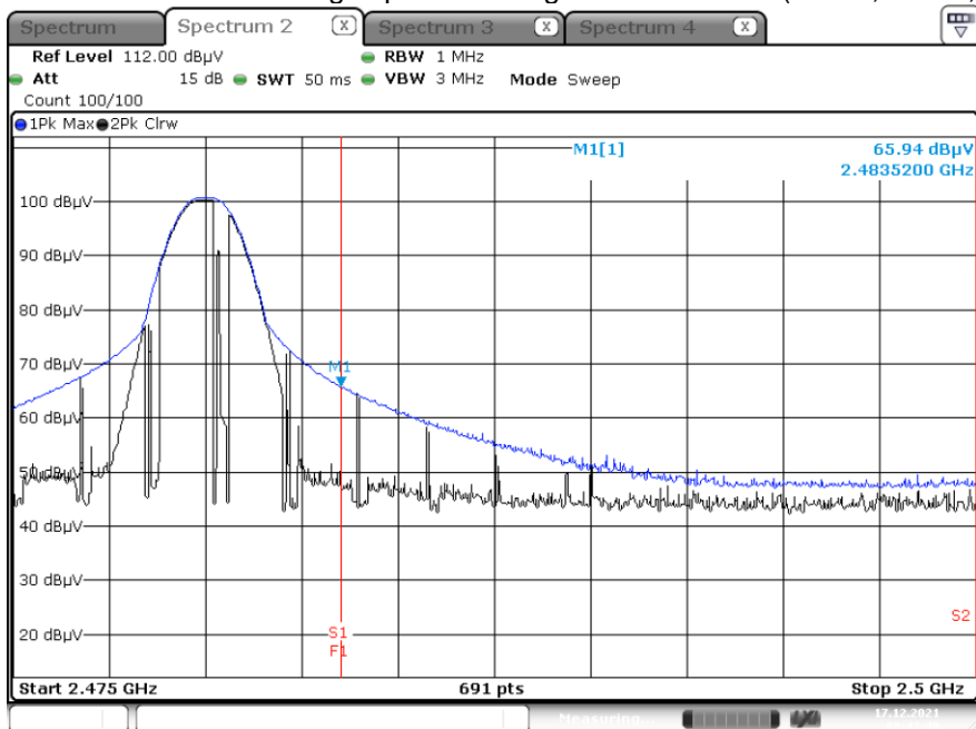
Radiated Restricted Band Edges plot – Average &amp; Peak Result (GFSK, Ch.78, Y-V)
