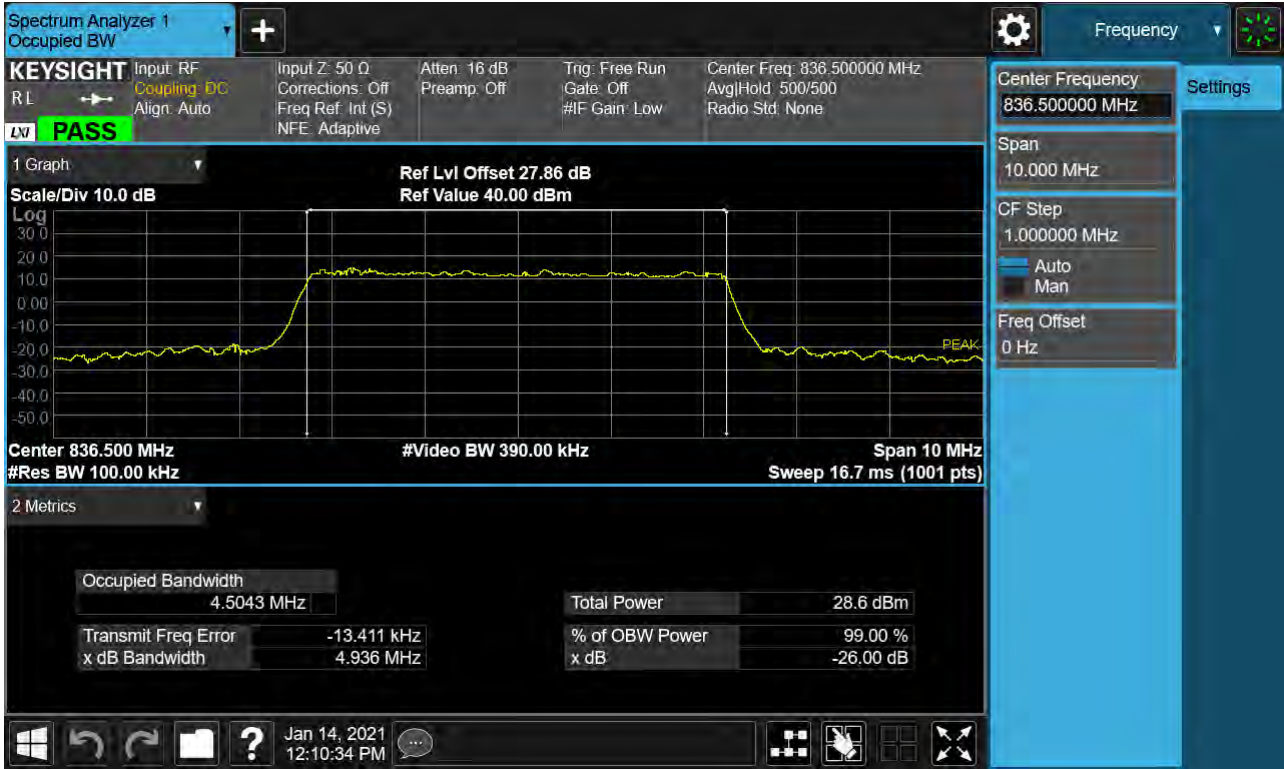
Sub6 n5. Occupied Bandwidth Plot (5M BW Ch.167300 256QAM_ RB25_0)
