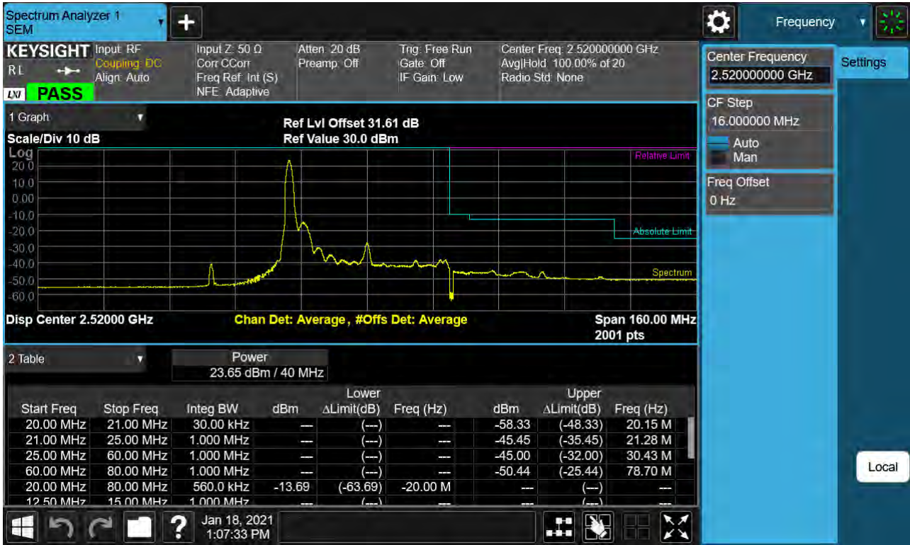
Sub6 n41. Low Channel Edge Plot (40 MHz Ch.504000 BPSK_RB1)-2
