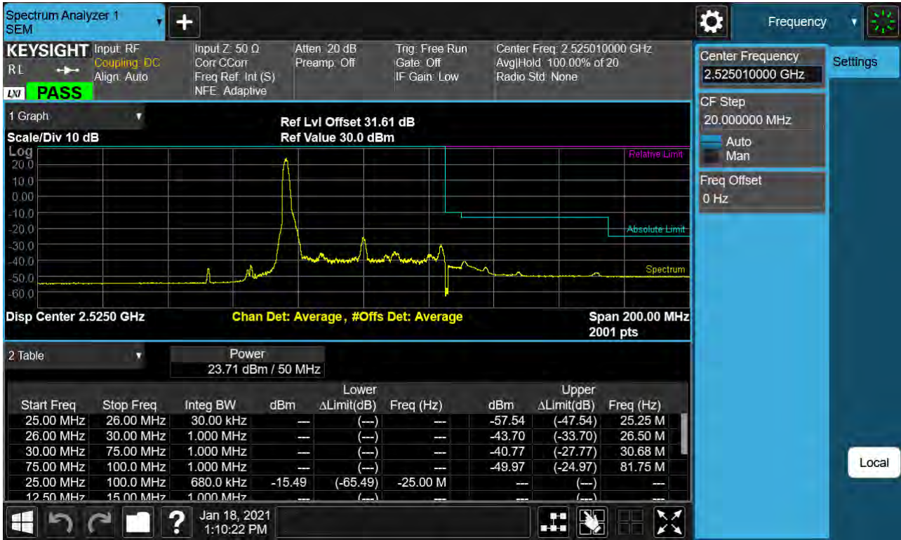
Sub6 n41. Low Channel Edge Plot (50 MHz Ch.505002 BPSK_RB1)-2
