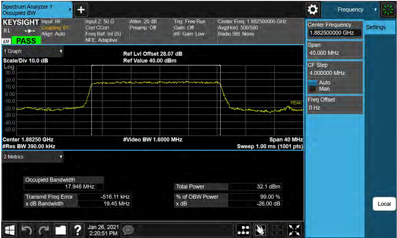
Sub6 n25. Occupied Bandwidth Plot (20M BW Ch.376500 BPSK RB 106_0)
