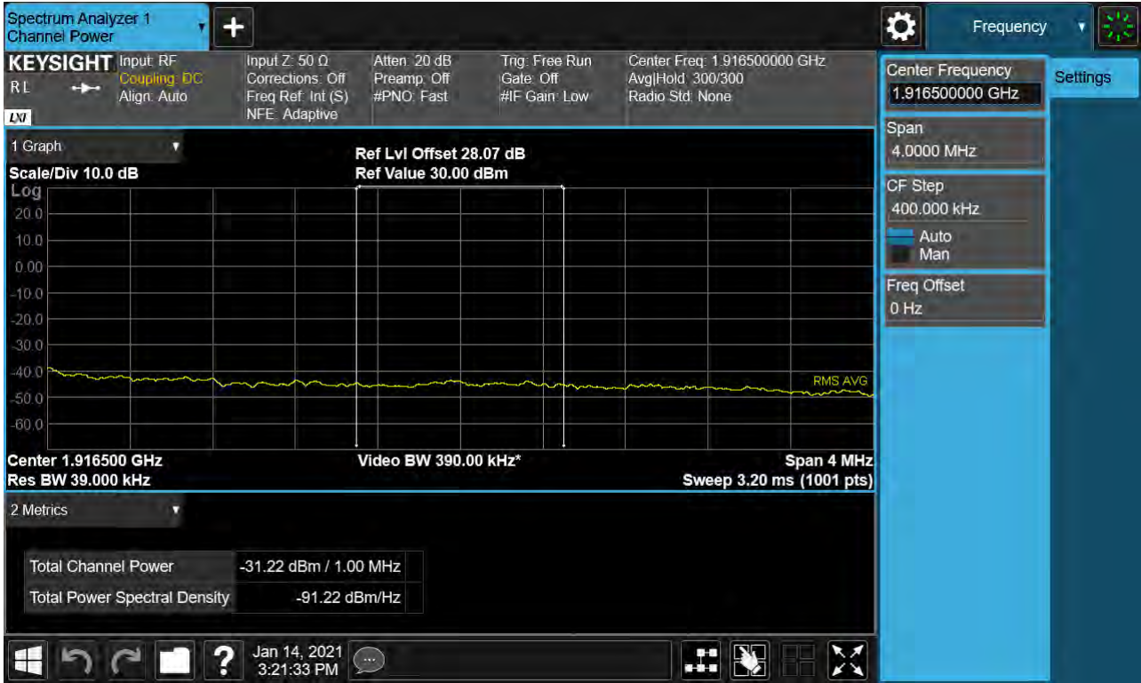
Sub6 n25. Upper Extended Band Edge Plot (20M BW Ch.381000 BPSK_RB106_0) -2
