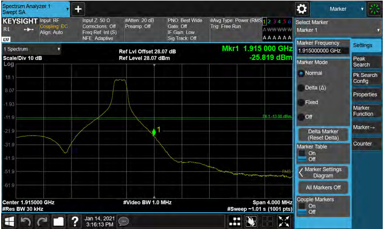
Sub6 n25. Upper Band Edge Plot (15M BW Ch.381500 BPSK_RB1_Offset 78)
