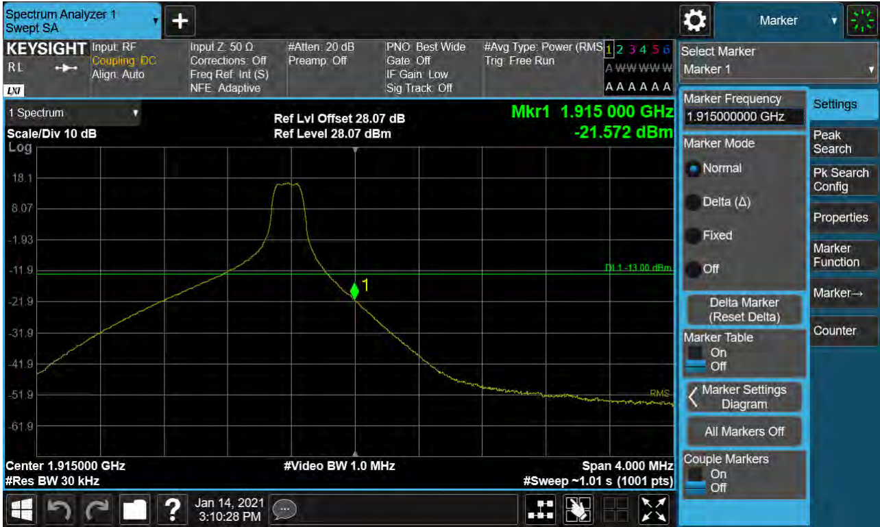
Sub6 n25. Upper Band Edge Plot (10M BW Ch.382000 BPSK_RB1_Offset 51)
