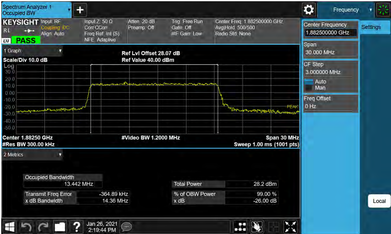
Sub6 n25. Occupied Bandwidth Plot (15M BW Ch.376500 256QAM RB 79_0)
