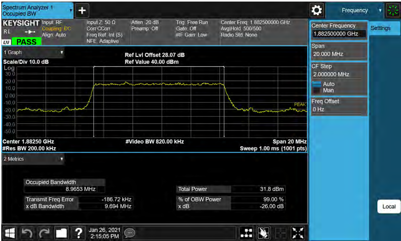
Sub6 n25. Occupied Bandwidth Plot (10M BW Ch.376500 BPSK RB 52_0)
