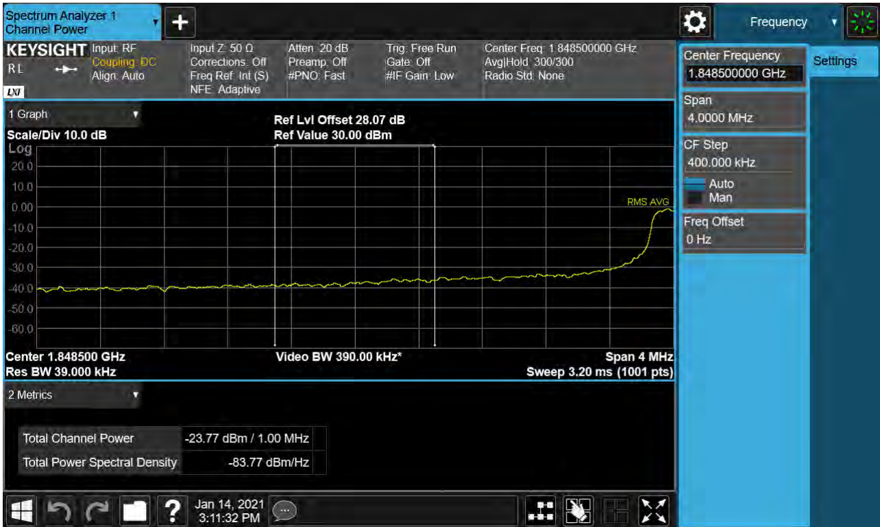
Sub6 n25. Lower Extended Band Edge Plot (15M BW Ch.371500 BPSK_RB79_0) -2
