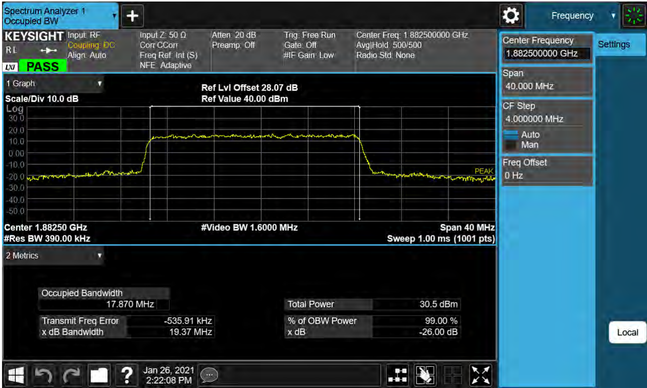
Sub6 n25. Occupied Bandwidth Plot (20M BW Ch.376500 64QAM RB 106_0)
