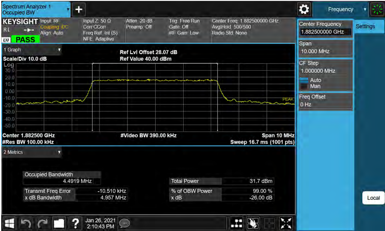
Sub6 n25. Occupied Bandwidth Plot (5M BW Ch.376500 BPSK RB 25_0)
