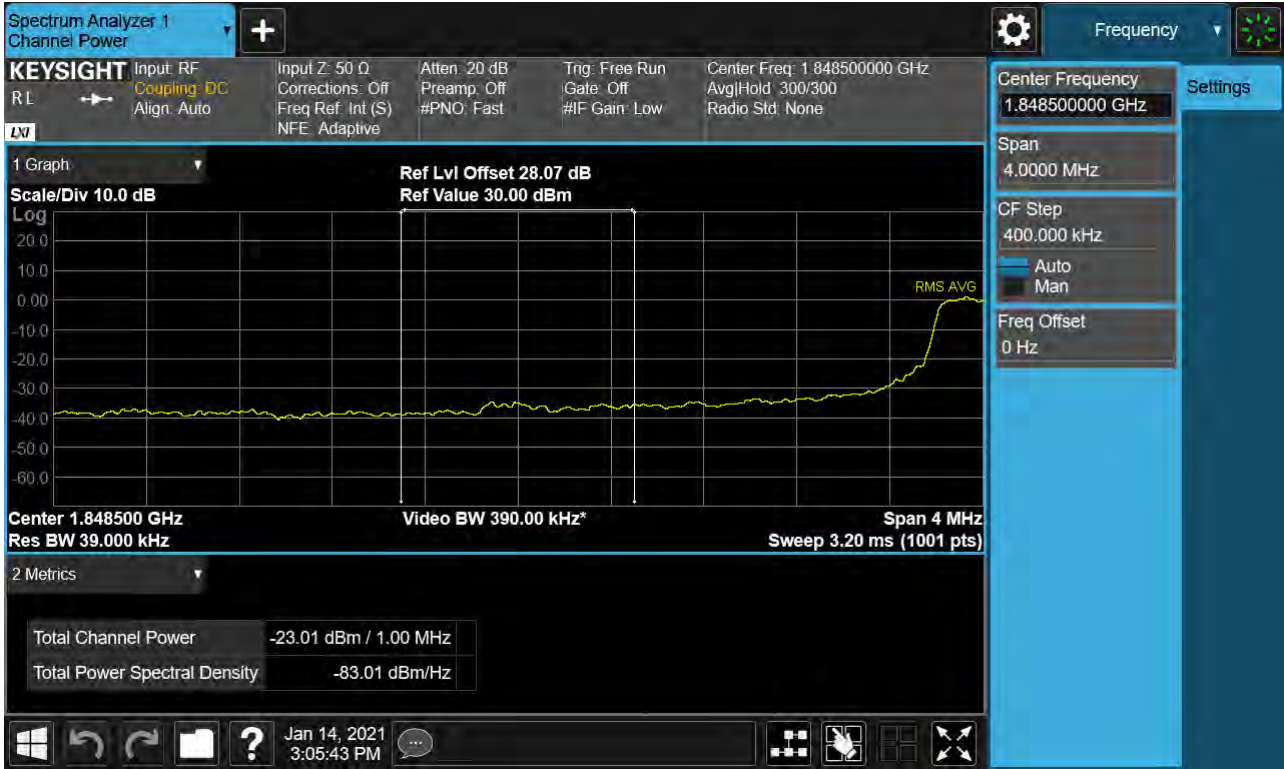
Sub6 n25. Lower Extended Band Edge Plot (10M BW Ch.371000 BPSK_RB52_0) -2
