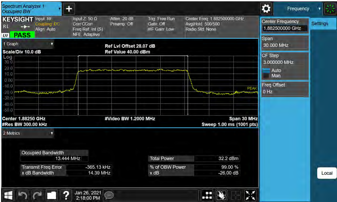
Sub6 n25. Occupied Bandwidth Plot (15M BW Ch.376500 BPSK RB 79_0)
