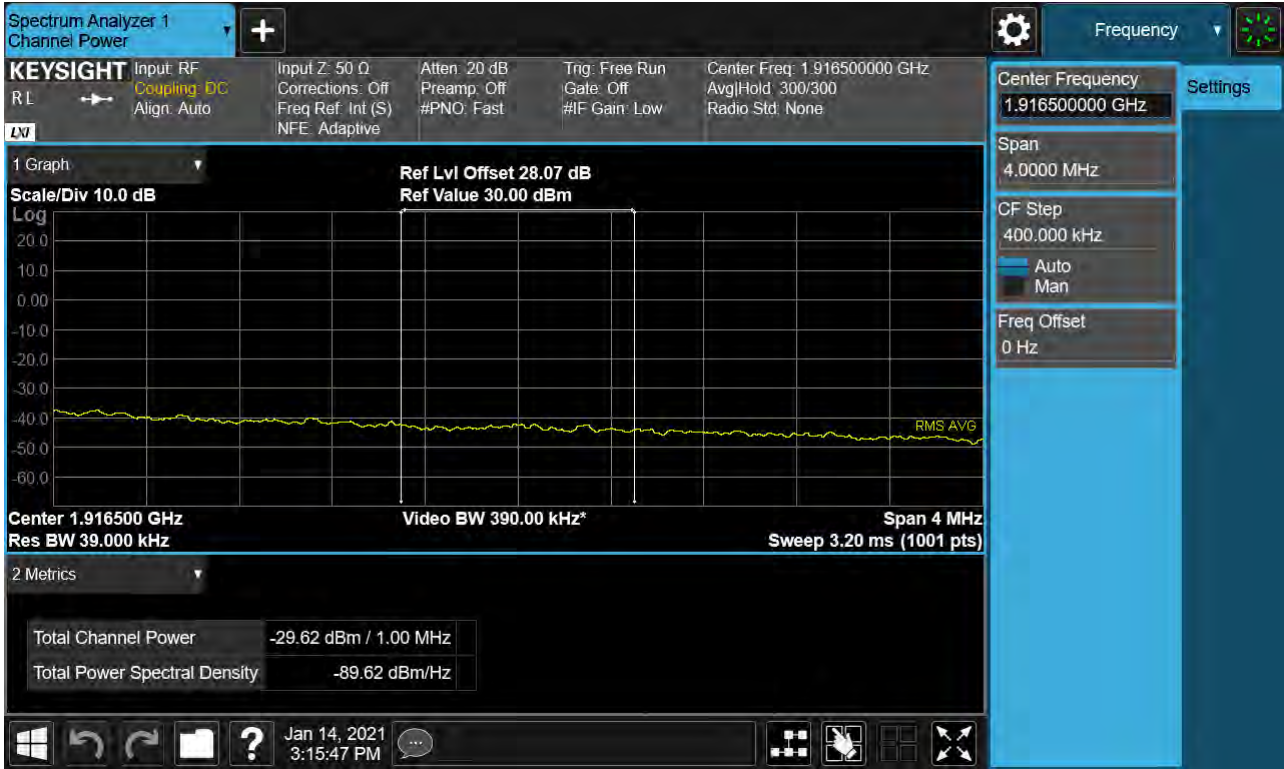
Sub6 n25. Upper Extended Band Edge Plot (15M BW Ch.381500 BPSK_RB79_0) -2
