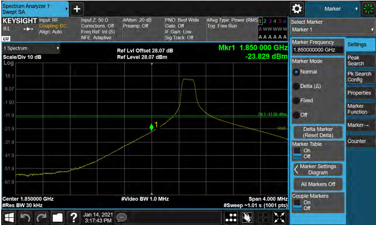
Sub6 n25. Lower Band Edge Plot (20M BW Ch.372000 BPSK_RB1_Offset 0)
