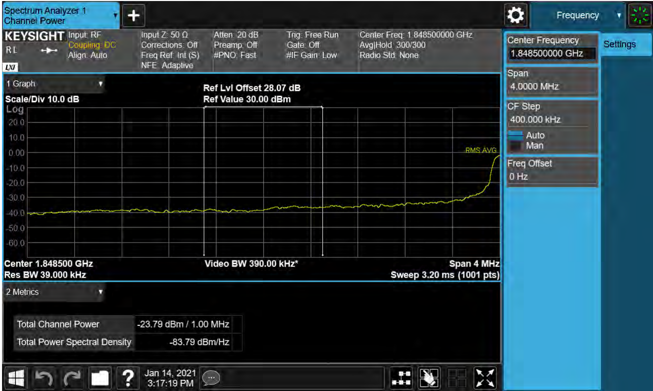
Sub6 n25. Lower Extended Band Edge Plot (20M BW Ch.372000 BPSK_RB106_0) -2
