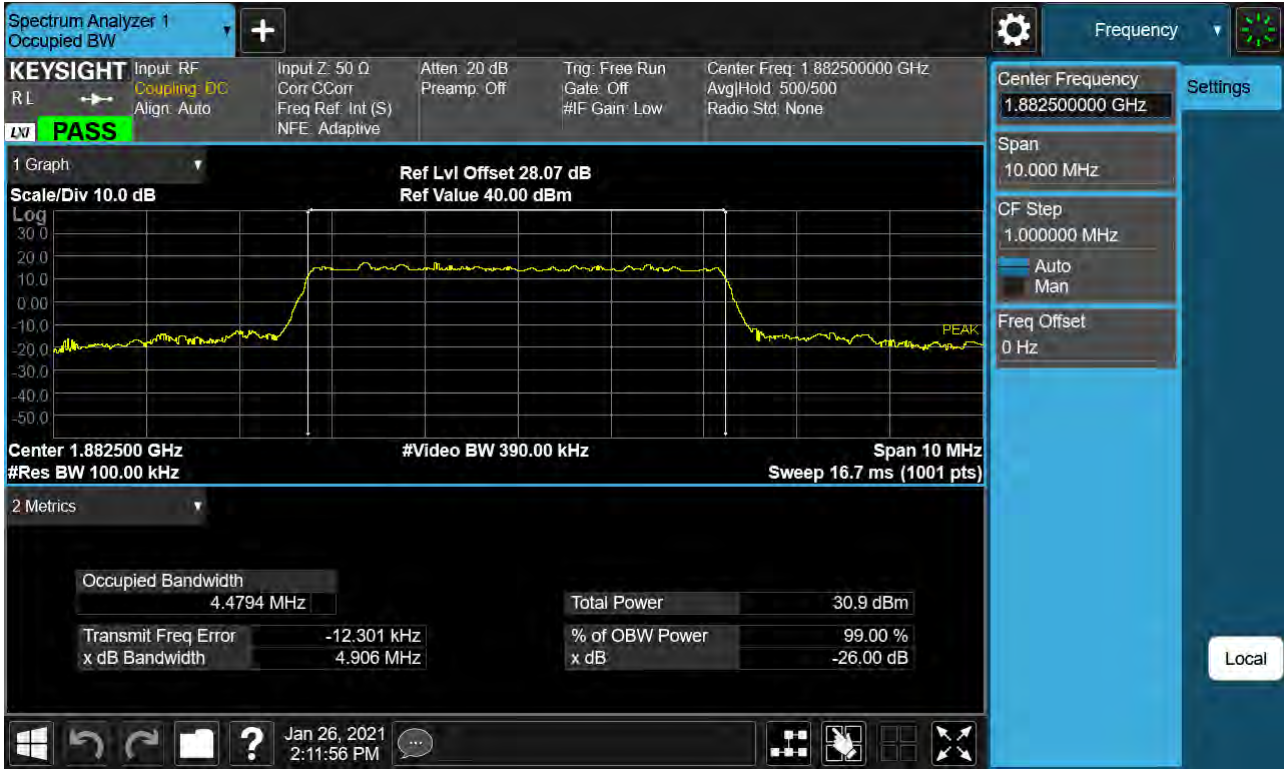
Sub6 n25. Occupied Bandwidth Plot (5M BW Ch.376500 16QAM RB 25_0)
