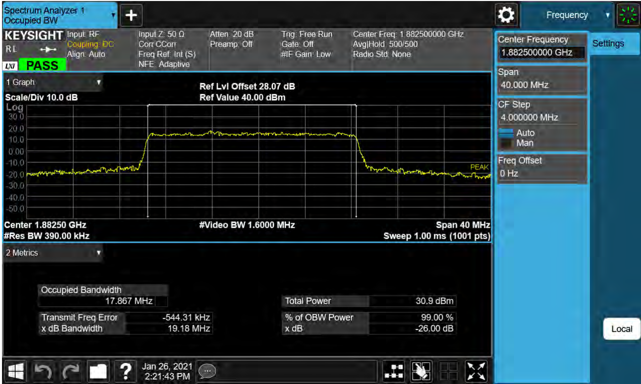
Sub6 n25. Occupied Bandwidth Plot (20M BW Ch.376500 16QAM RB 106_0)
