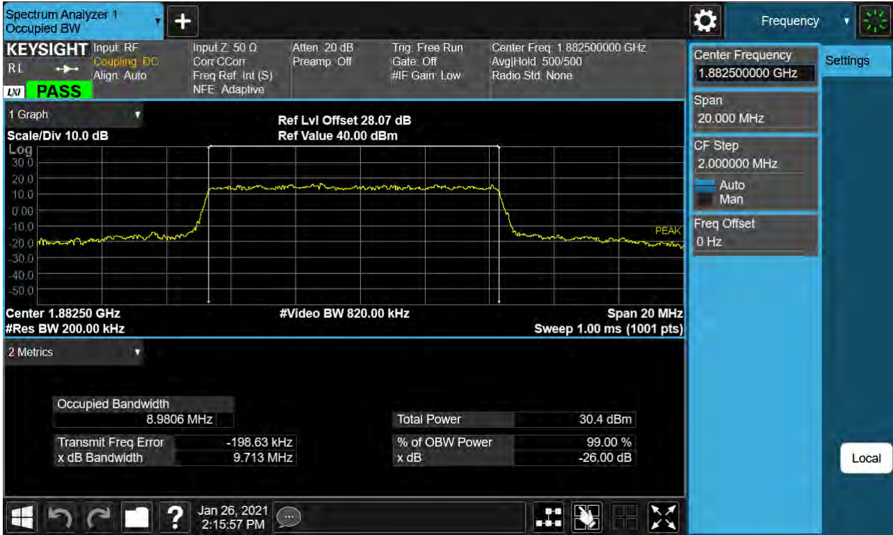
Sub6 n25. Occupied Bandwidth Plot (10M BW Ch.376500 16QAM RB 52_0)
