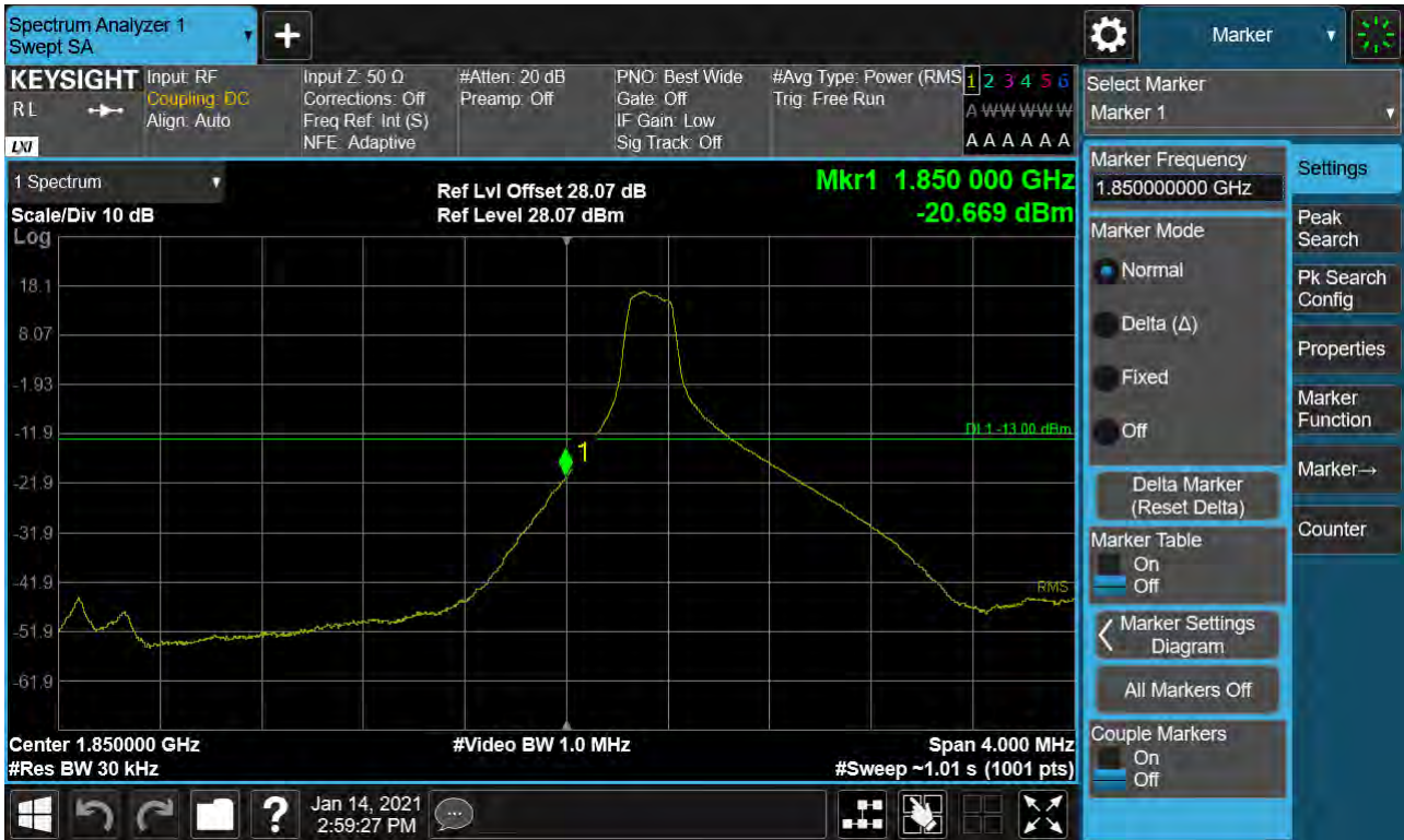
Sub6 n25. Lower Band Edge Plot (5M BW Ch.370500 BPSK_RB1_Offset 0)
