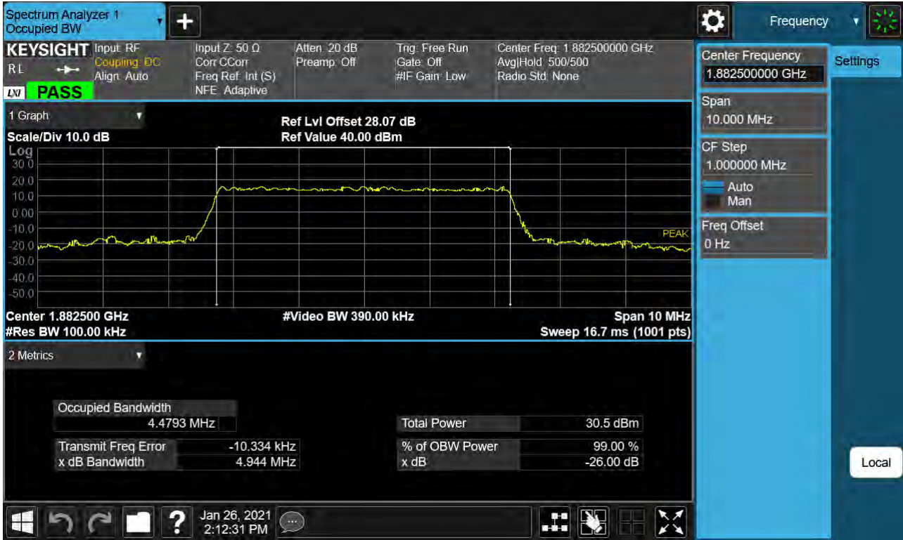
Sub6 n25. Occupied Bandwidth Plot (5M BW Ch.376500 64QAM RB 25_0)
