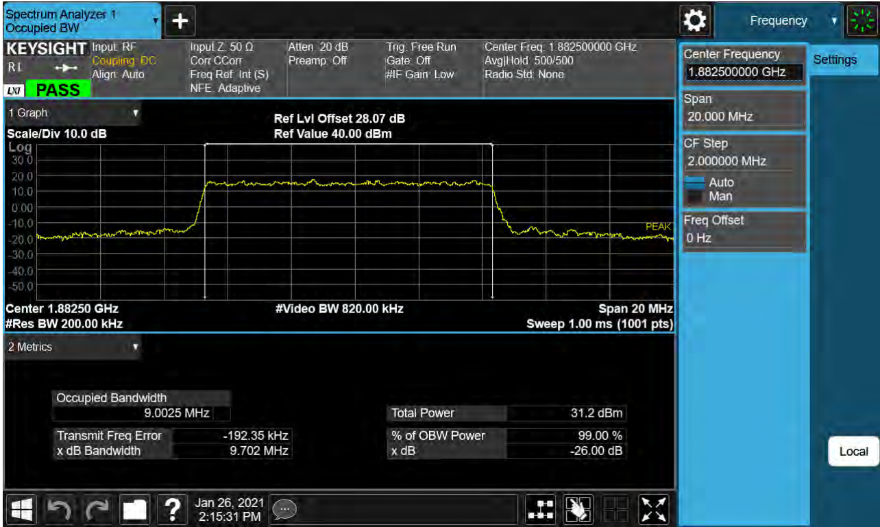
Sub6 n25. Occupied Bandwidth Plot (10M BW Ch.376500 QPSK RB 52_0)
