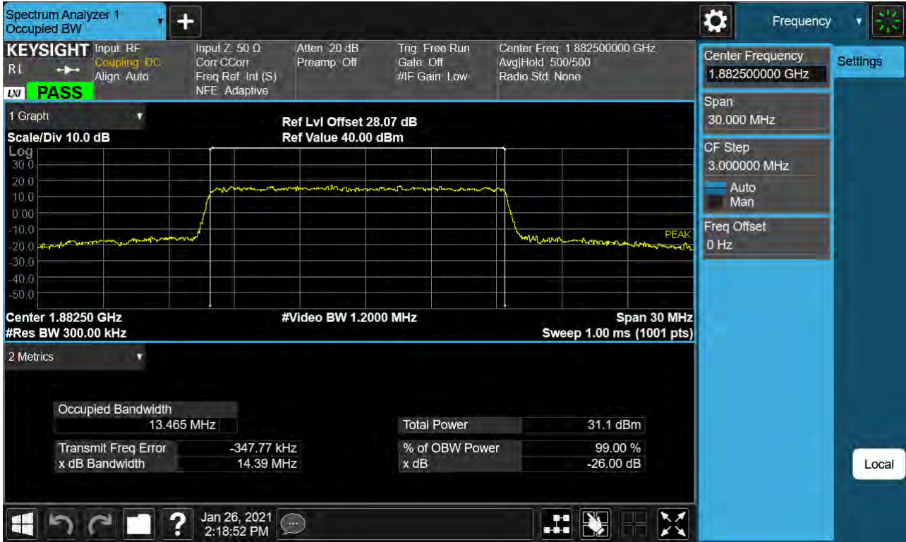
Sub6 n25. Occupied Bandwidth Plot (15M BW Ch.376500 16QAM RB 79_0)
