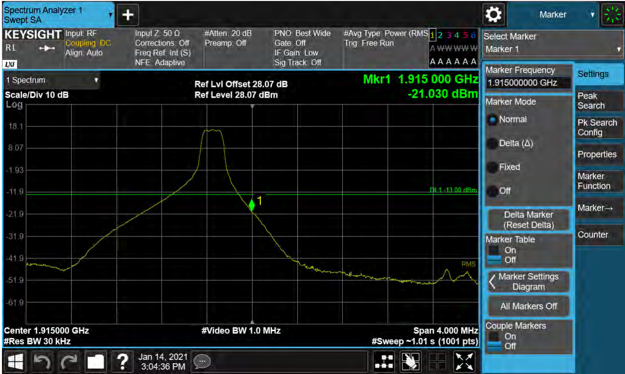
Sub6 n25. Upper Band Edge Plot (5M BW Ch.382500 BPSK_RB1_Offset 24)
