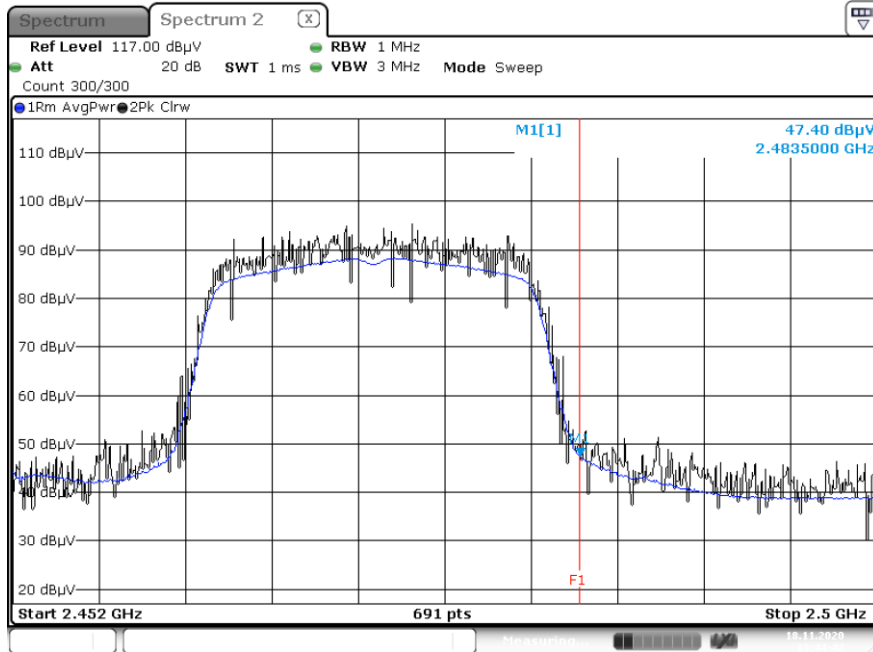
Radiated Restricted Band Edges plot – Average Reading (802.11n (HT20)_MCS0 Ch.13)
