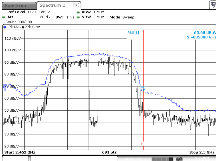
Radiated Restricted Band Edges plot – Peak Reading (802.11n (HT20)_ MCS0 Ch.13)
