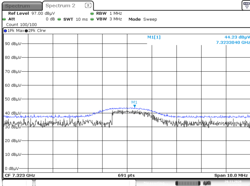
Radiated Spurious Emissions plot – Average & Peak Reading (GFSK, Ch.39 3rd Harmonic, X-H)
