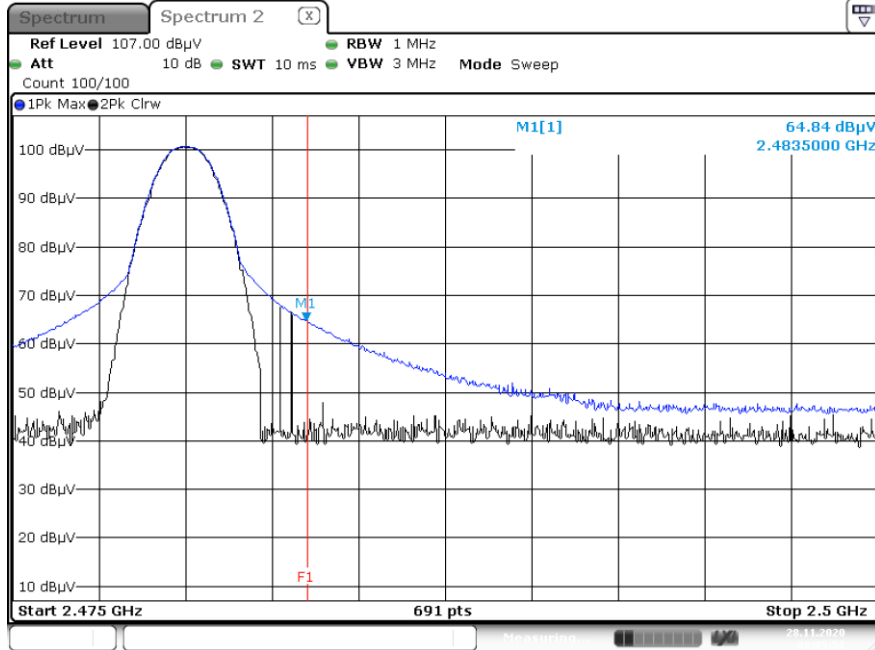
Radiated Restricted Band Edges plot – Average & Peak Reading (GFSK, Ch.78)
