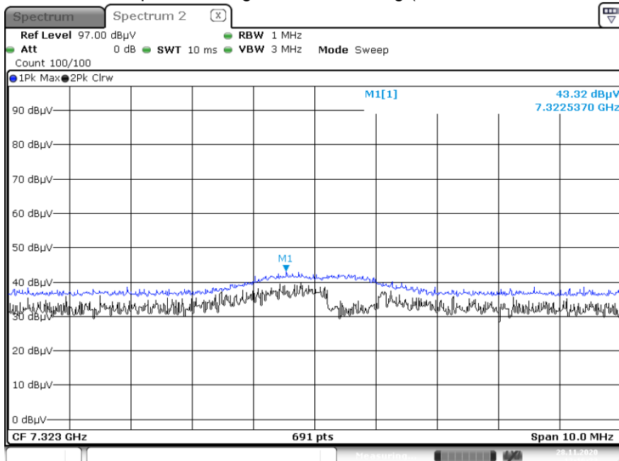
Radiated Spurious Emissions plot – Average & Peak Reading ( \pi/4 DQPSK, Ch.39 3rd Harmonic, X-H)
