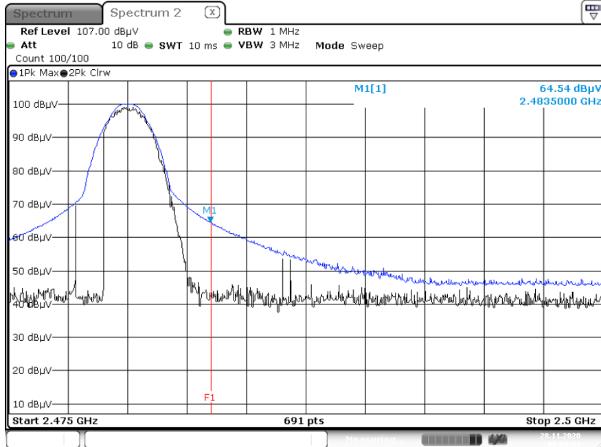
Radiated Restricted Band Edges plot – Average & Peak Reading ( \pi/4 DQPSK, Ch.78)
