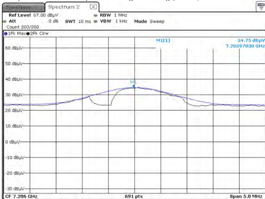
Radiated Spurious Emissions plot – Average Reading (GFSK, Ch.0 3rd Harmonic, Y-H)
