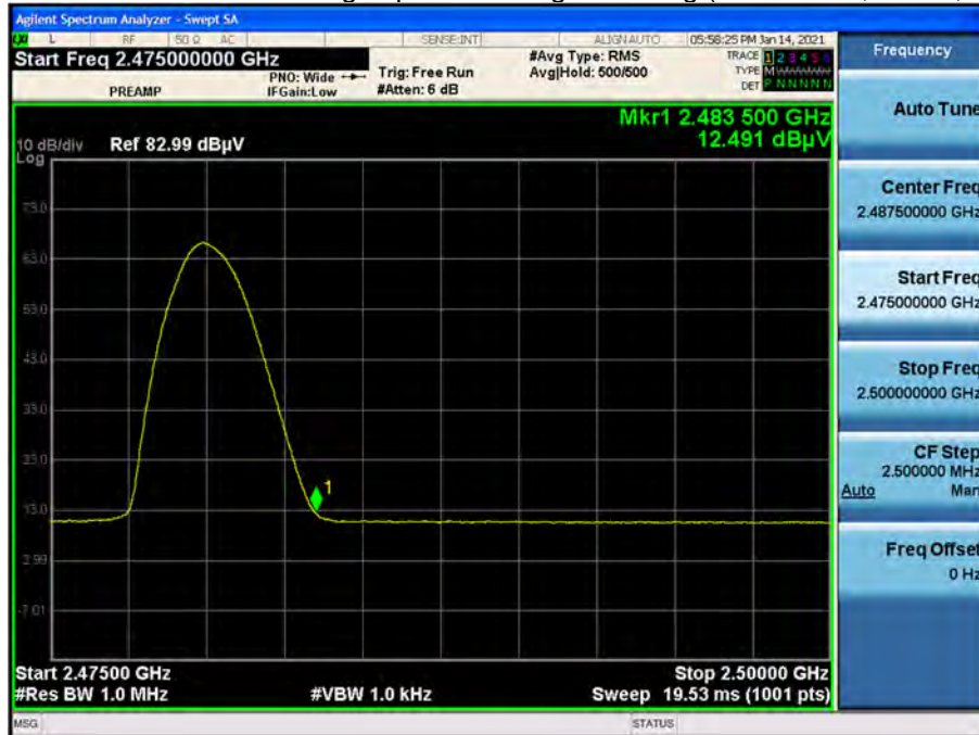
Radiated Restricted Band Edges plot – Average Reading ( \pi/4 DQPSK, Ch.78, X-H)
