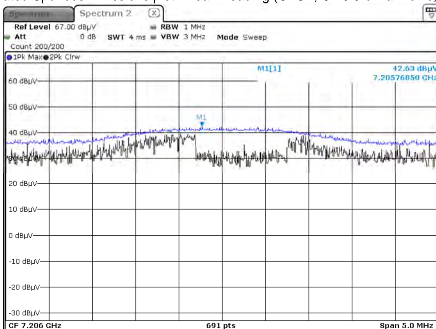
Radiated Spurious Emissions plot –Peak Reading (GFSK, Ch.0 3rd Harmonic, Y-H)
