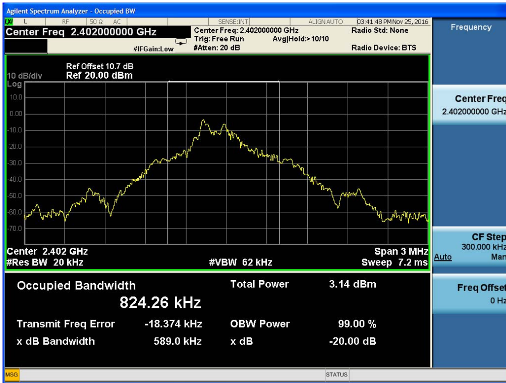
Occupied Bandwidth plot (Low)
