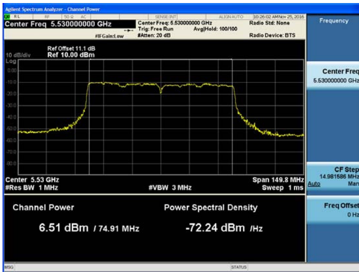
802.11ac_VHT80 UNII 2C BAND Average Power (5530 ~ 5610 MHz) CH 106 MCS3
