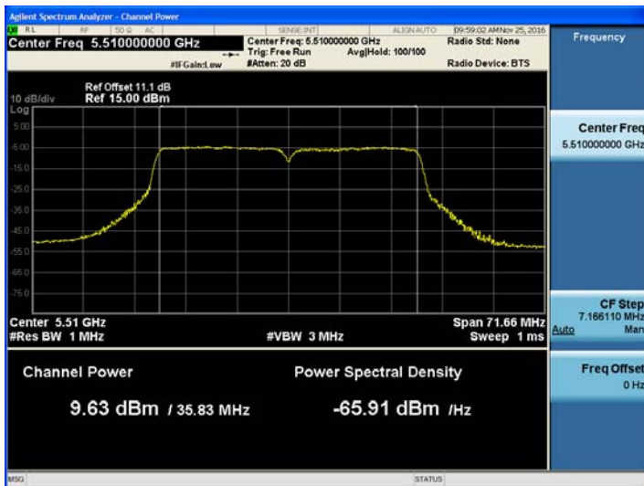
802.11ac_VHT40 UNII 2C BAND Average Power (5510 MHz ~5670 MHz) CH 102 MCS3
