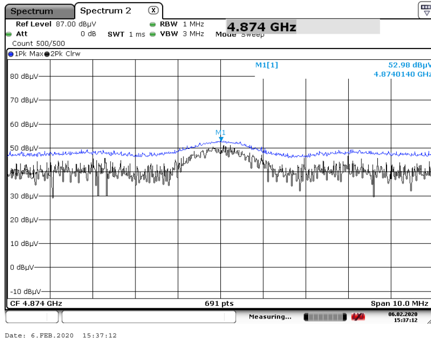
Radiated Spurious Emissions plot – Peak Reading (802.11b_1 Mbps, Ch.6 2nd Harmonic)
