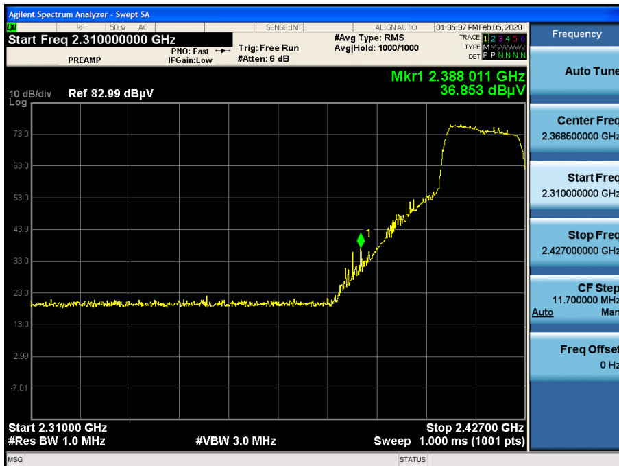
Radiated Restricted Band Edges plot – Peak Reading (802.11n (HT20)_ Ch.2)
