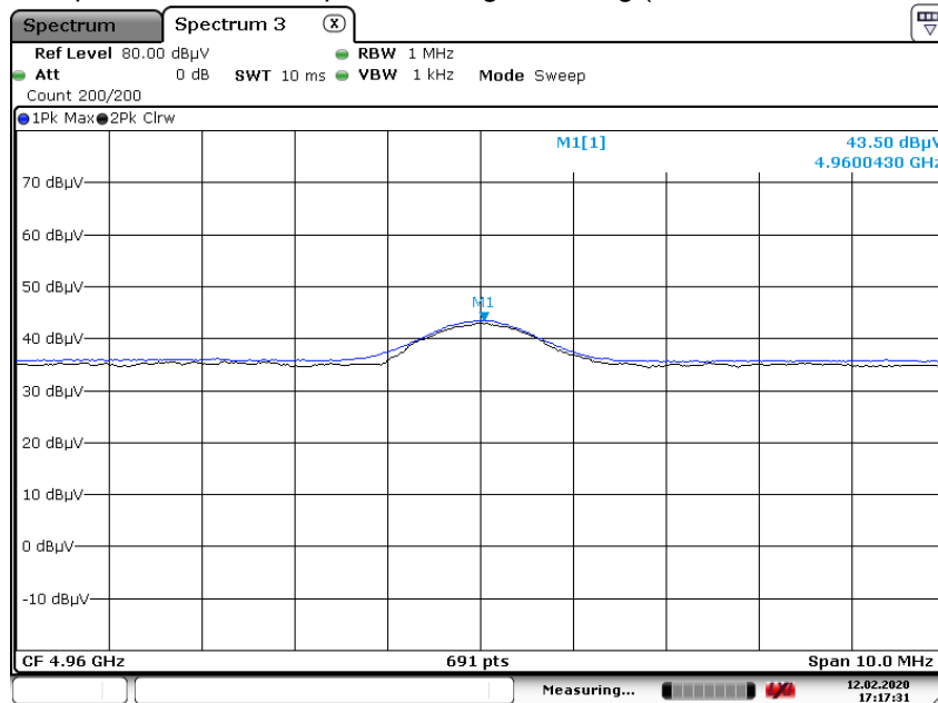
Radiated Spurious Emissions plot – Average Reading (GFSK, Ch.78 2nd Harmonic)
