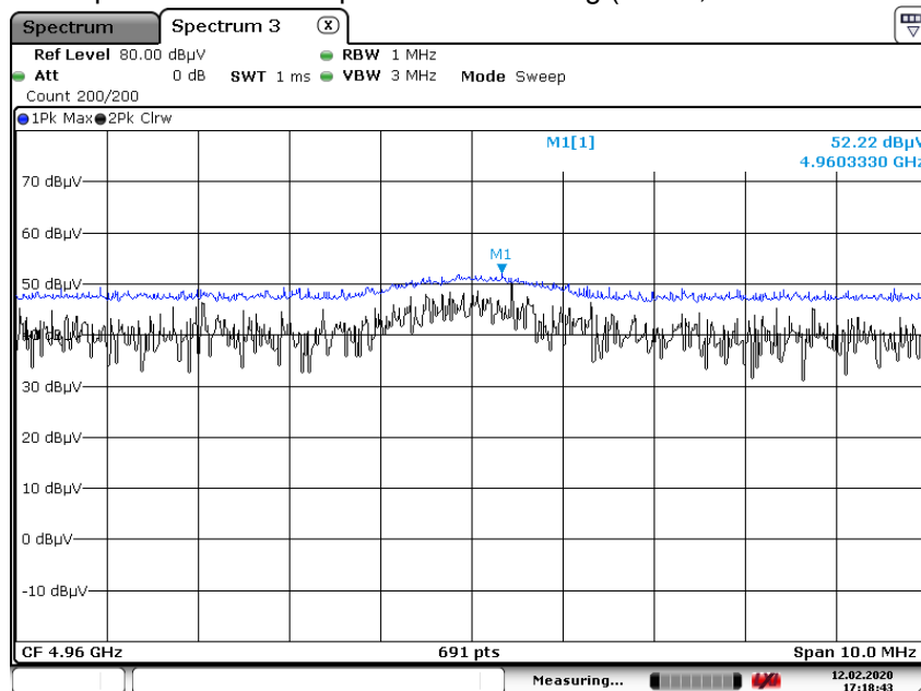
Radiated Spurious Emissions plot – Peak Reading (GFSK, Ch.78 2nd Harmonic)
