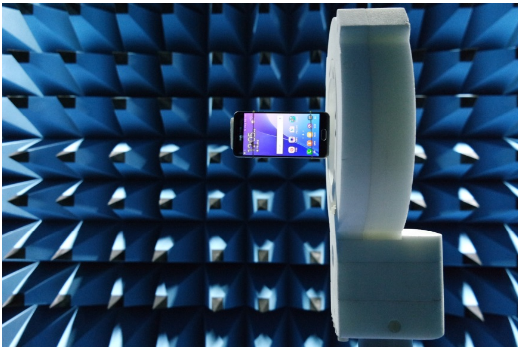
Figure 2. 2G/3G/LTE ERP/EIRP and LTE RSE testing setup
