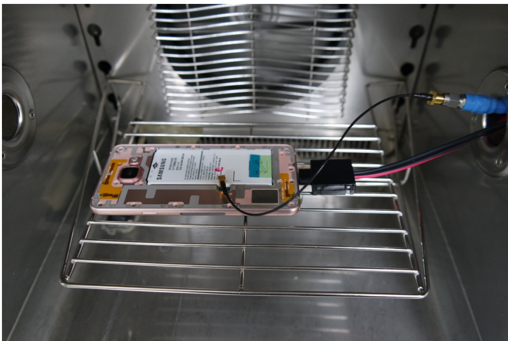
Figure 4. LTE conducted testing setup
