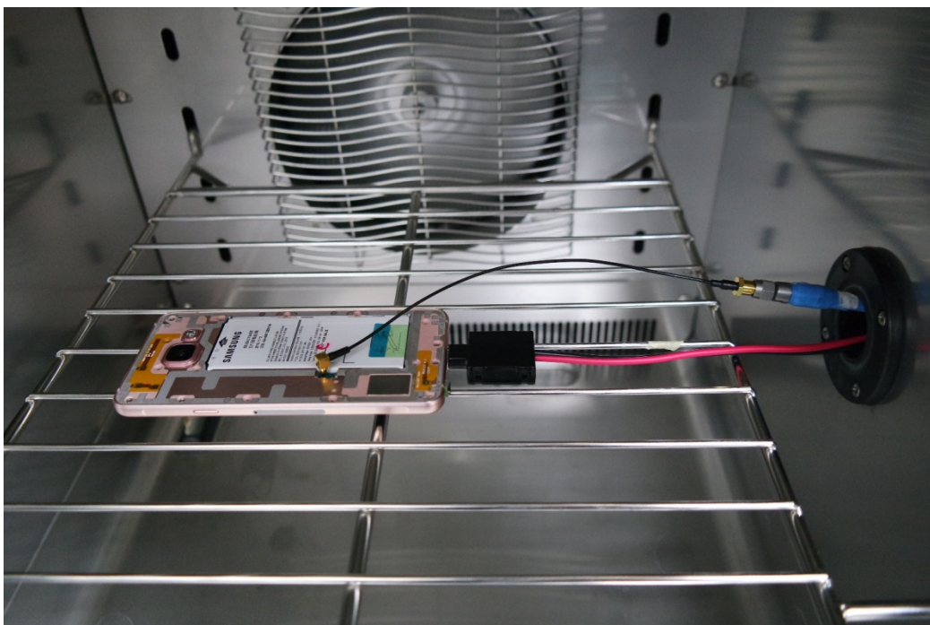
Figure 3. 2G/3G conducted testing setup
