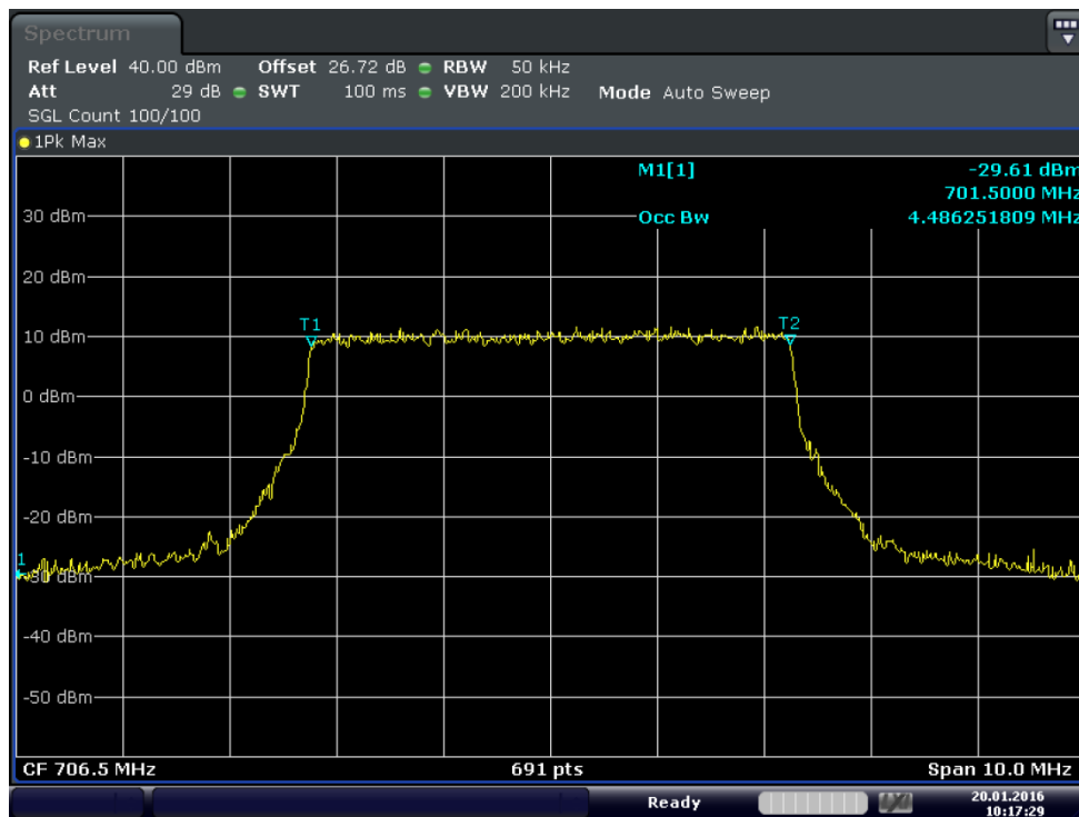
Plot 6-1. Occupied Bandwidth Plot (Band 17 – 5MHz QPSK - RB Size 25)
