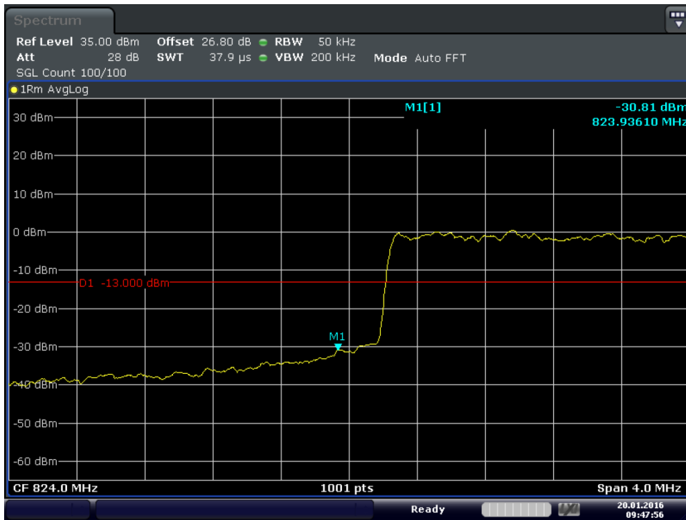
Plot 6-47. Lower Band Edge Plot (Band 5 – 5.0MHz – QPSK – RB Size 25)
