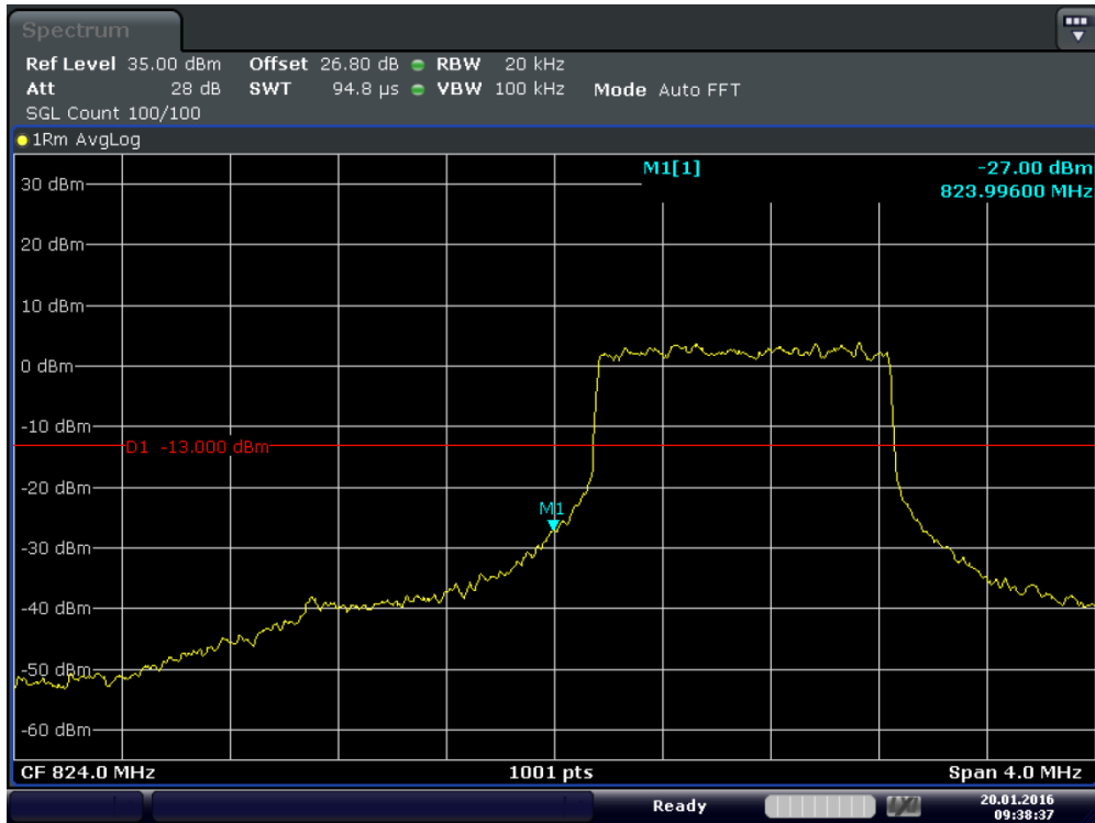
Plot 6-39. Lower Band Edge Plot (Band5 – 1.4MHz – QPSK – RB Size 6)
