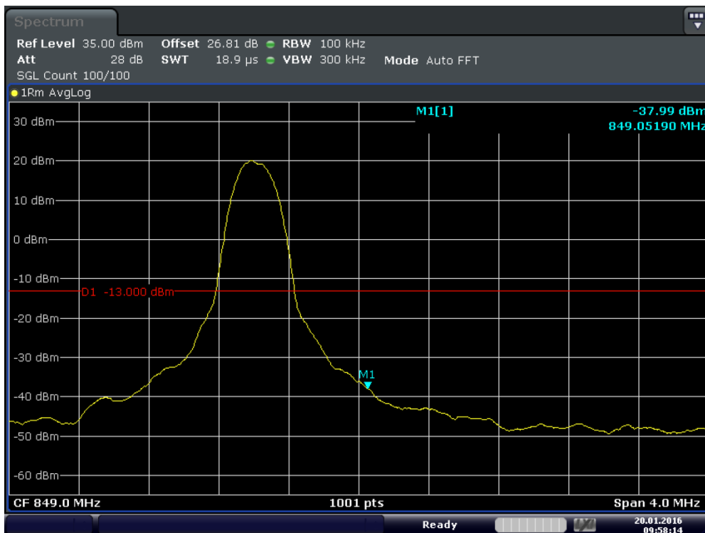
Plot 6-54. Upper Band Edge Plot (Band 5 – 10.0MHz – QPSK – RB Size 1 – RB Offset 49)
