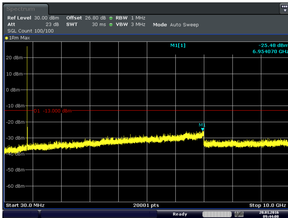
Plot 6-22. Conducted Spurious Plot (Band 5-3.0MHz-QPSK-RB Size 1-RB Offset 14- Ch.20415)
