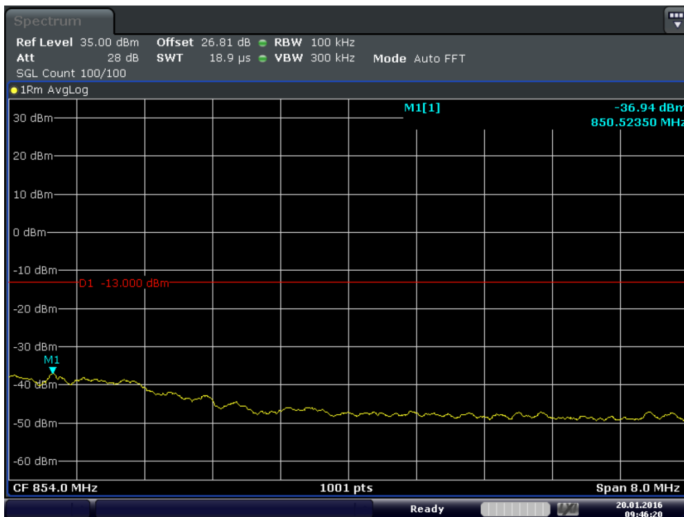
Plot 6-46. Extended Upper Band Edge Plot (Band 5 – 3.0MHz – QPSK – RB Size 15)
