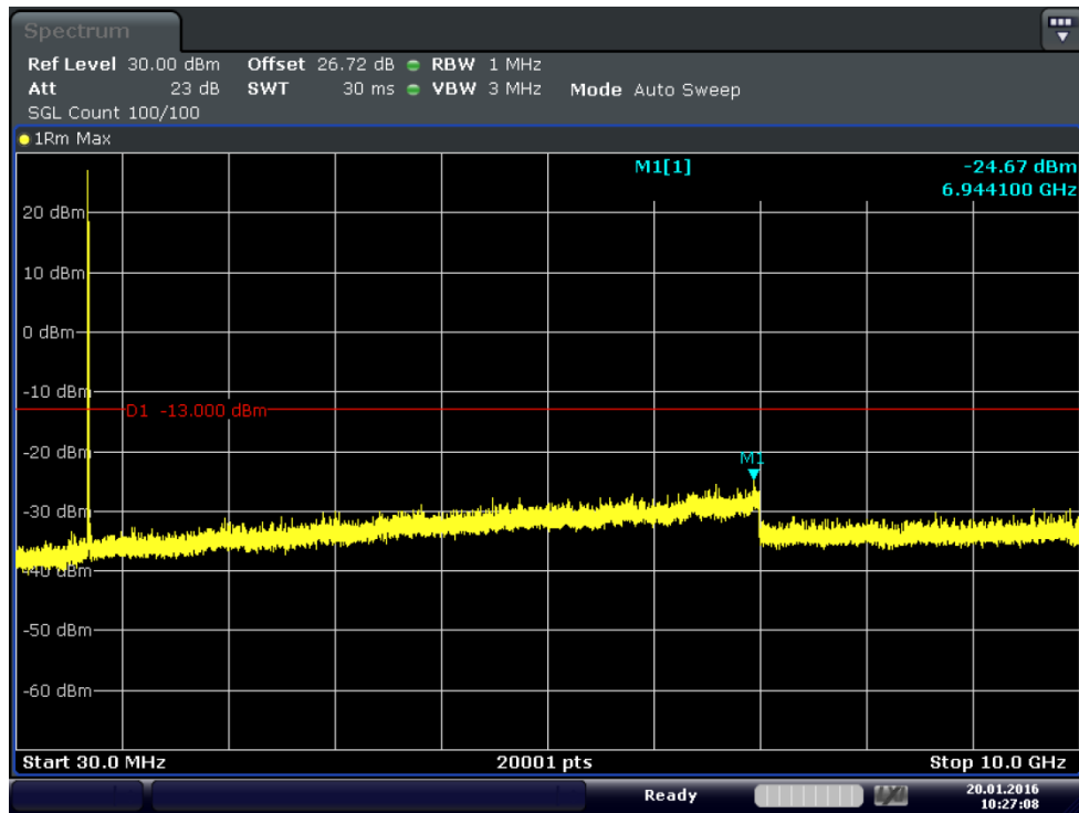
Plot 6-16. Conducted Spurious Plot (Band 17-10MHz-QPSK-RB Size 1-RB Offset 0-Ch.23780)
