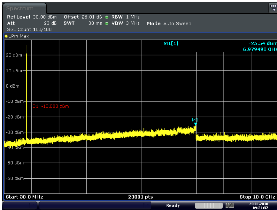
Plot 6-27. Conducted Spurious Plot (Band 5-5.0MHz-QPSK-RB Size 1-RB Offset 0- Ch.20625)
