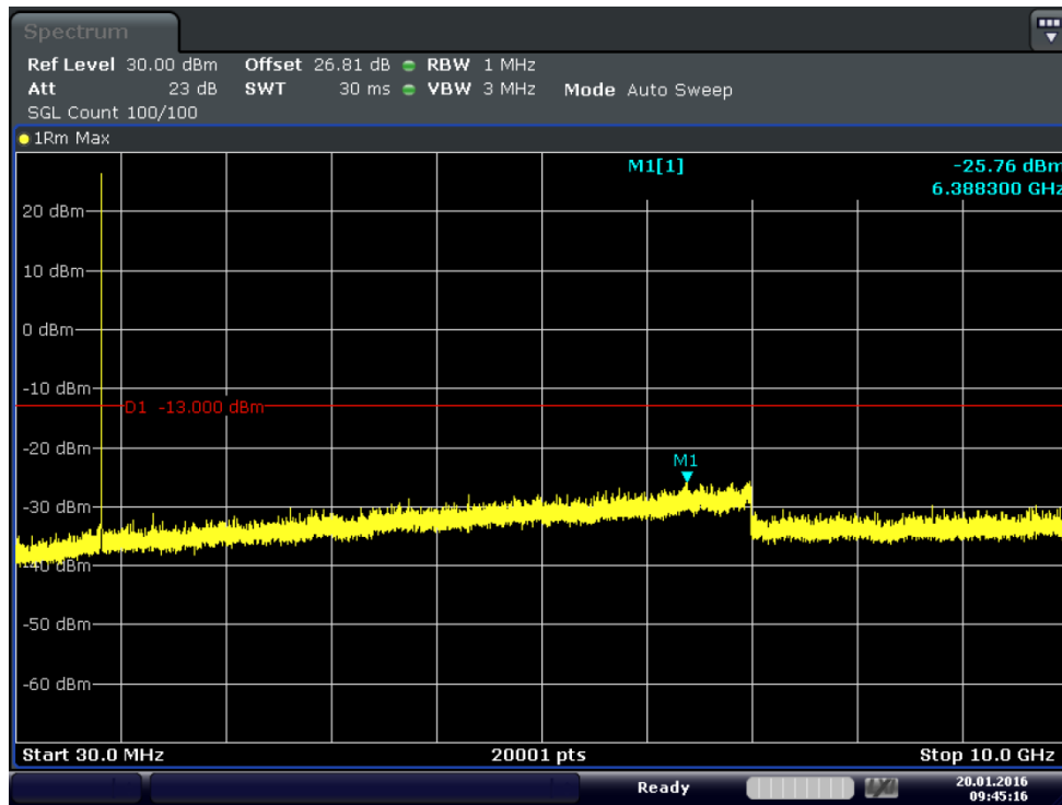
Plot 6-23. Conducted Spurious Plot (Band 5–3.0MHz–QPSK–RB Size 1–RB Offset 14– Ch.20525)
