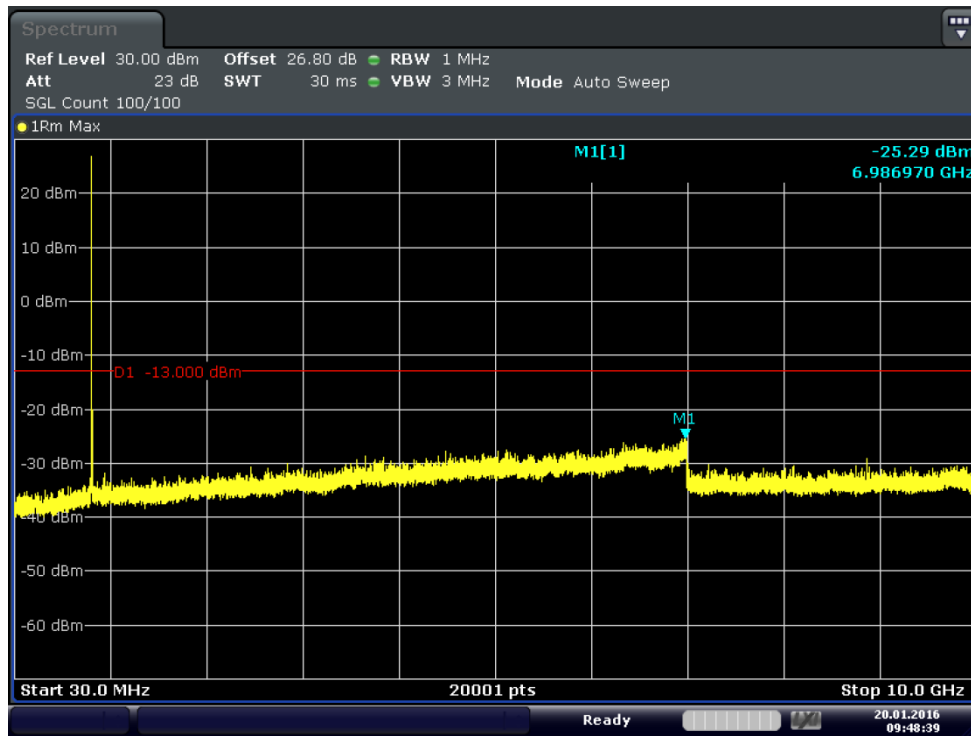
Plot 6-25. Conducted Spurious Plot (Band 5-5.0MHz-QPSK-RB Size 1-RB Offset 0- Ch.20425)
