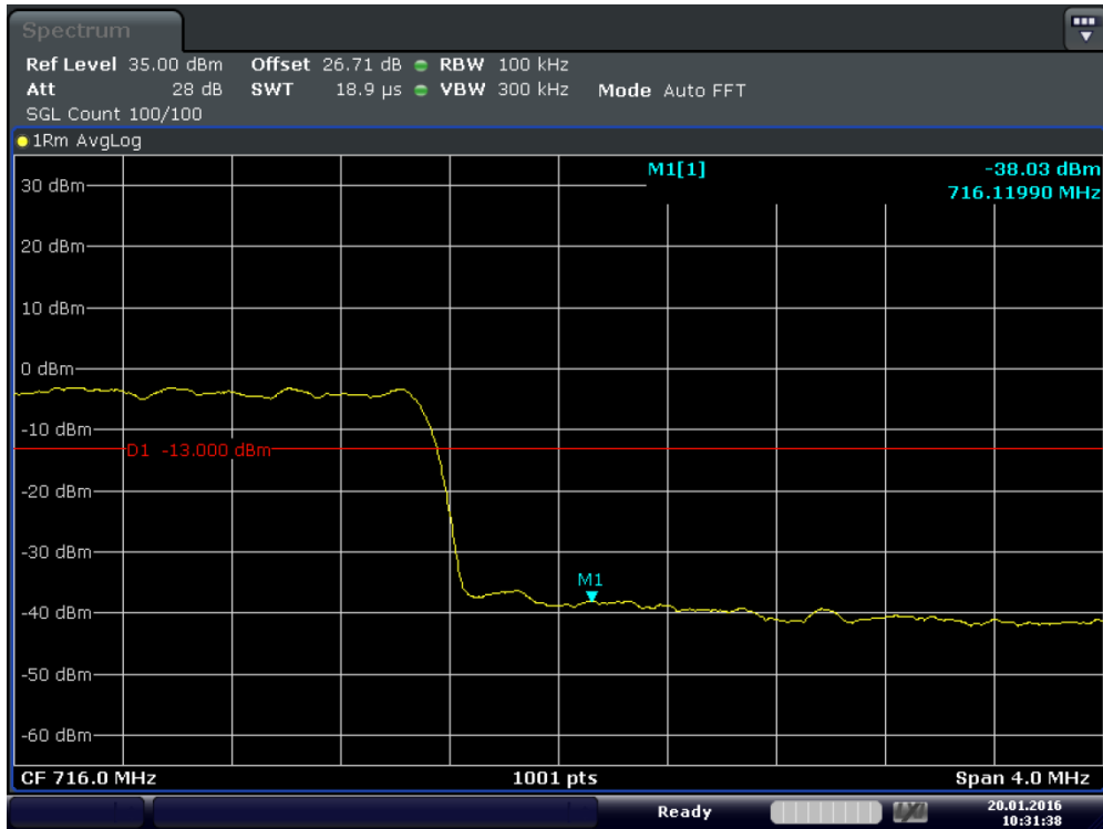
Plot 6-37. Upper Band Edge Plot (Band17 – 10MHz – QPSK – RB Size 50)
