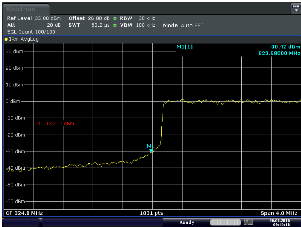
Plot 6-43. Lower Band Edge Plot (Band 5 – 3.0MHz – QPSK – RB Size 15)
