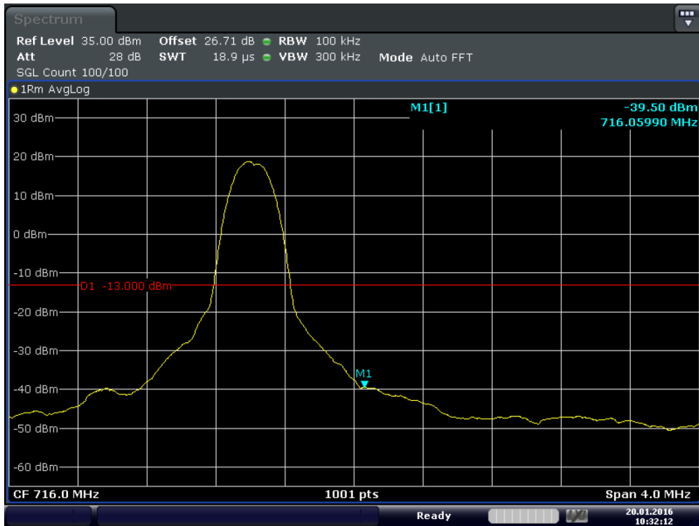
Plot 6-38. Upper Band Edge Plot (Band17 – 10MHz – QPSK – RB Size 1 – RB Offset 49)
