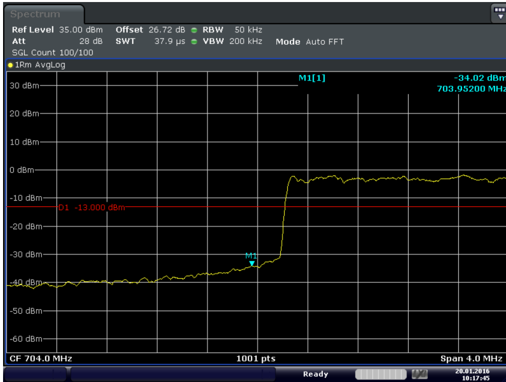
Plot 6-31. Lower Band Edge Plot (Band17 – 5MHz – QPSK – RB Size 25)
