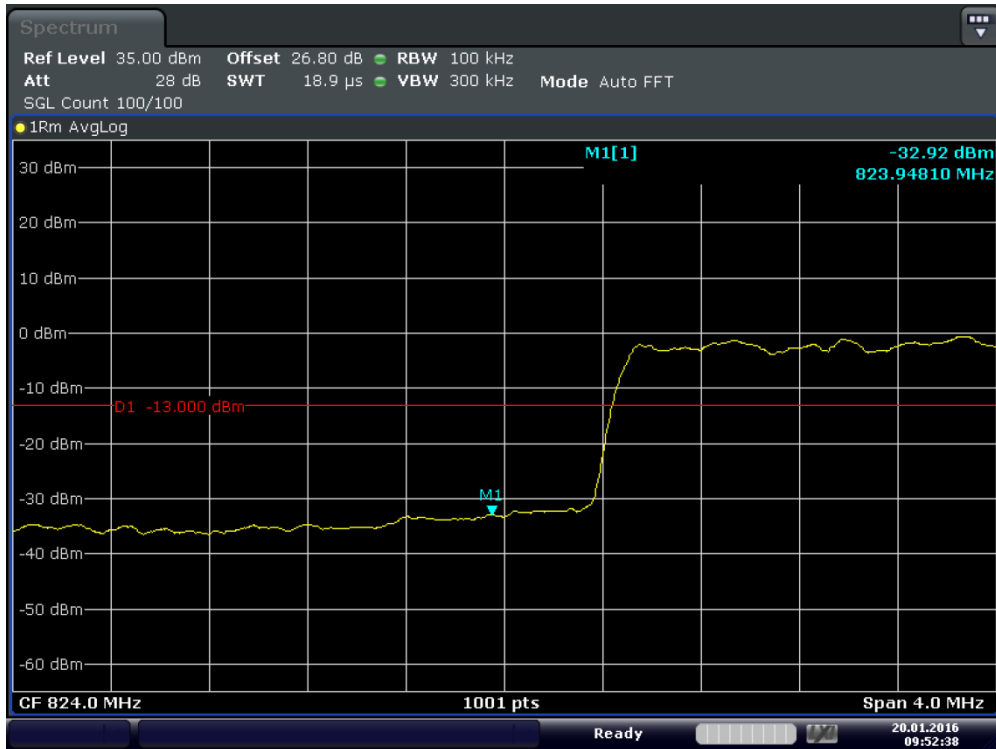
Plot 6-51. Lower Band Edge Plot (Band 5 – 10.0MHz – QPSK – RB Size 50)
