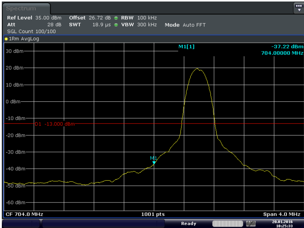
Plot 6-36. Lower Band Edge Plot (Band17 – 10MHz – QPSK – RB Size 1 – RB Offset 0)
