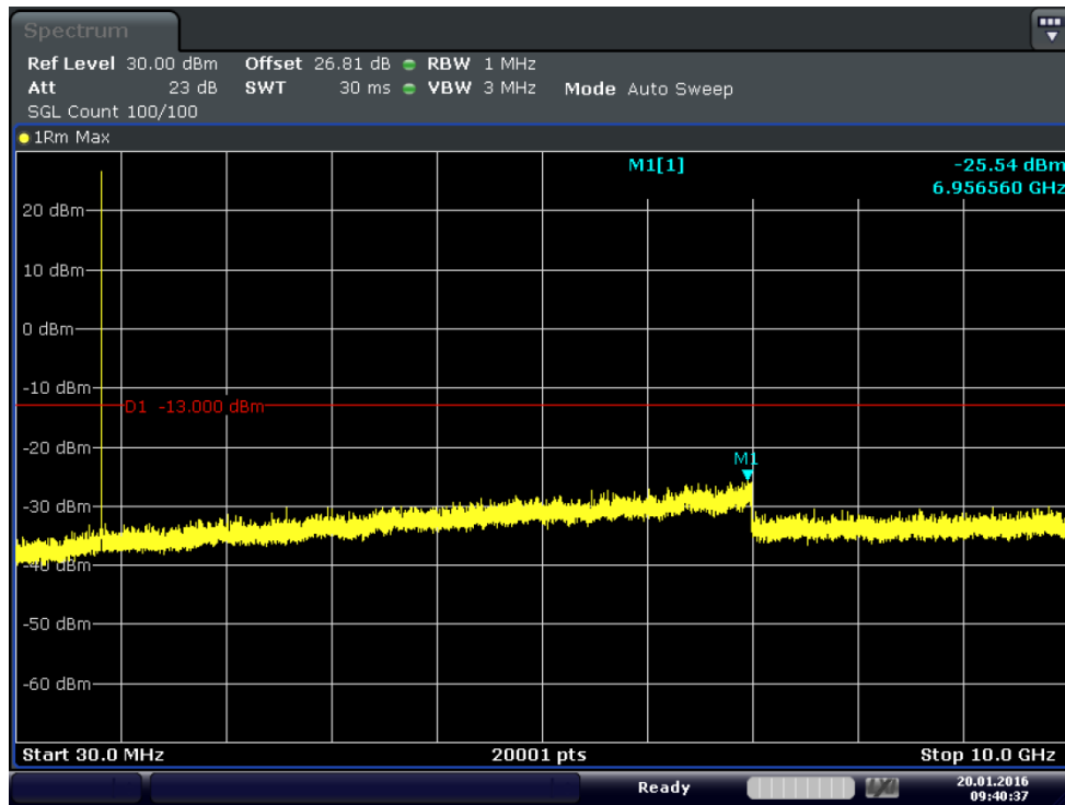
Plot 6-20. Conducted Spurious Plot (Band 5-1.4MHz-QPSK-RB Size 3-RB Offset 2-Ch.20525)
