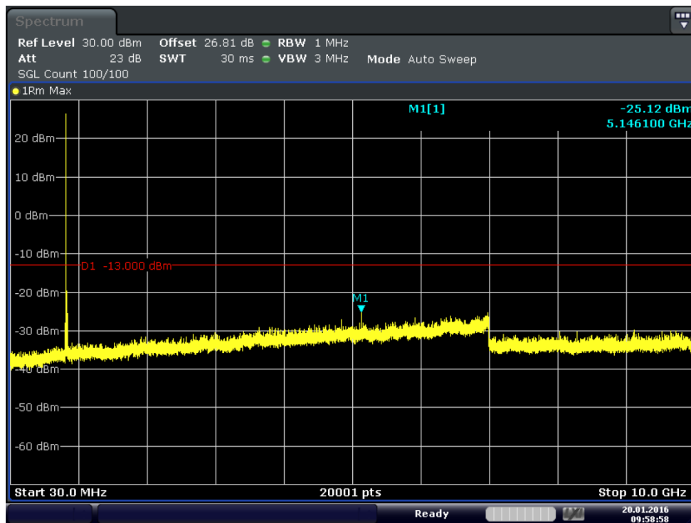
Plot 6-30. Conducted Spurious Plot (Band 5–10.0MHz–QPSK–RB Size 1–RB Offset 0– Ch.20600)
