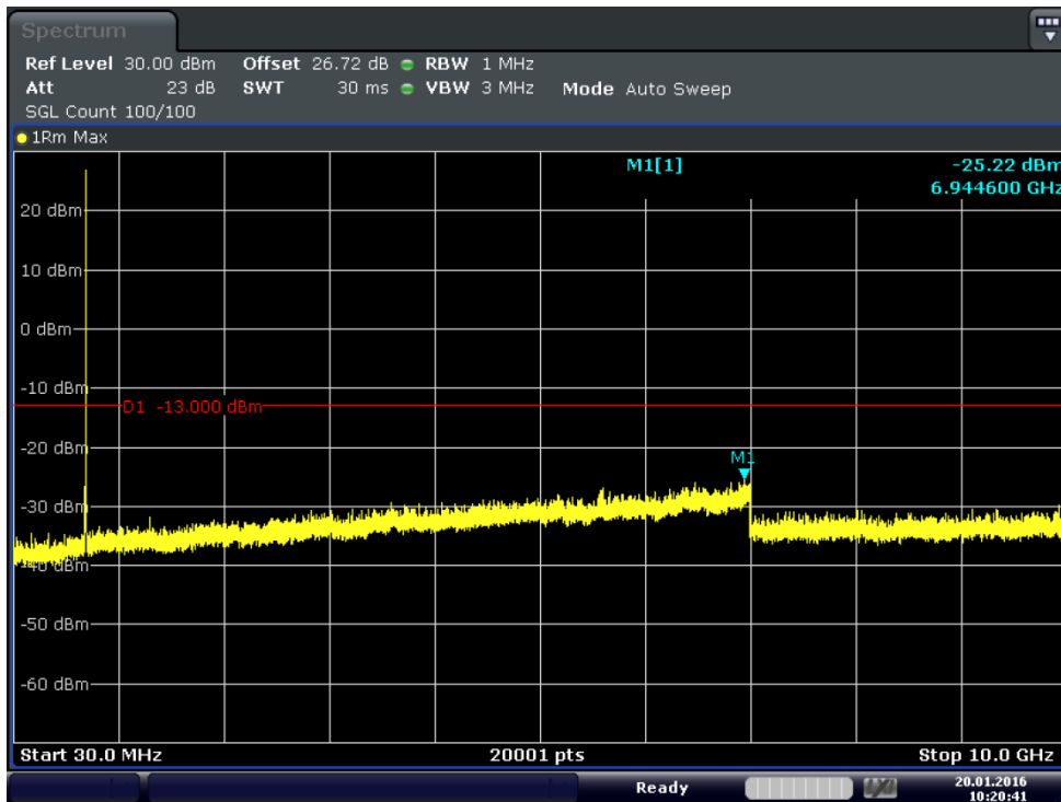
Plot 6-13. Conducted Spurious Plot (Band 17-5MHz-QPSK-RB Size 1-RB Offset 24-Ch.23755)
