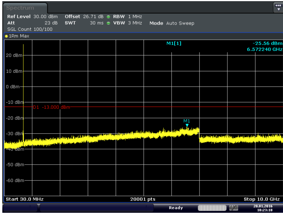
Plot 6-15. Conducted Spurious Plot (Band 17-5MHz-QPSK-RB Size 1-RB Offset 0-Ch.23825)
