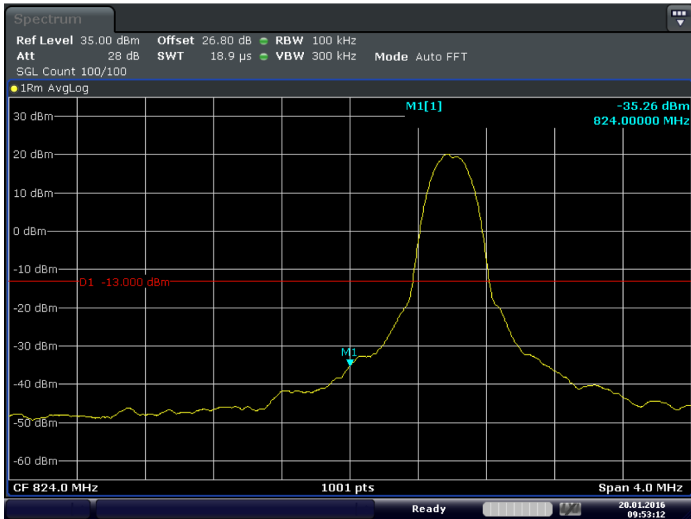
Plot 6-52. Lower Band Edge Plot (Band 5 – 10.0MHz – QPSK – RB Size 1 – RB Offset 0)
