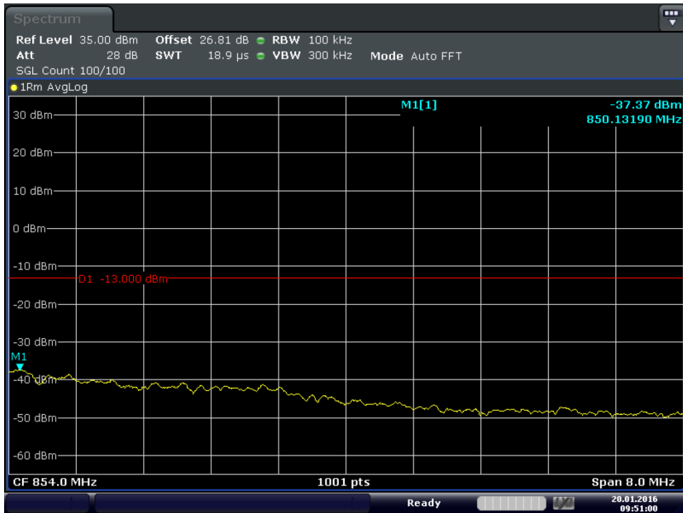
Plot 6-50. Extended Upper Band Edge Plot (Band 5 – 5.0MHz – QPSK – RB Size 25)
