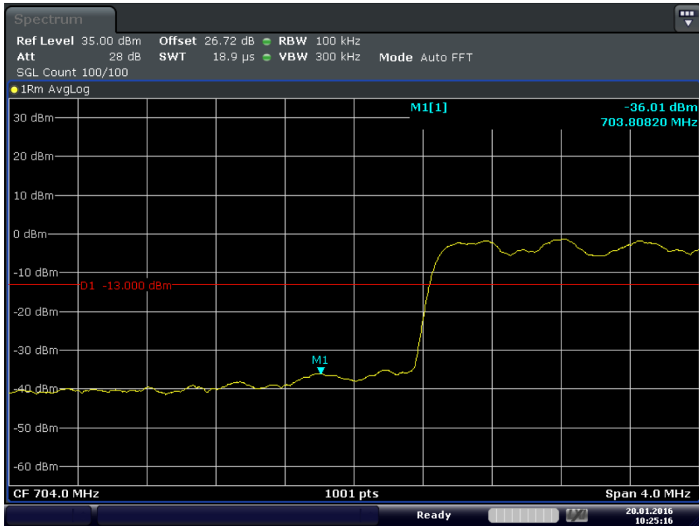
Plot 6-35. Lower Band Edge Plot (Band17 – 10MHz – QPSK – RB Size 50)
