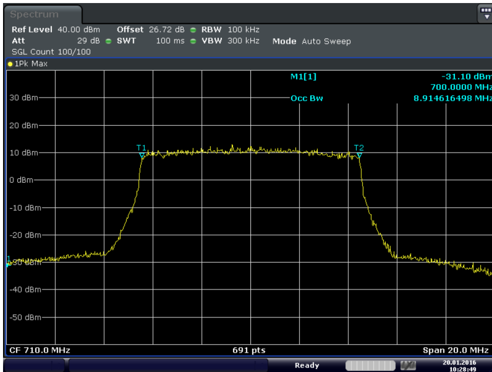
Plot 6-4. Occupied Bandwidth Plot (Band 17 – 10MHz 16QAM - RB Size 50)
