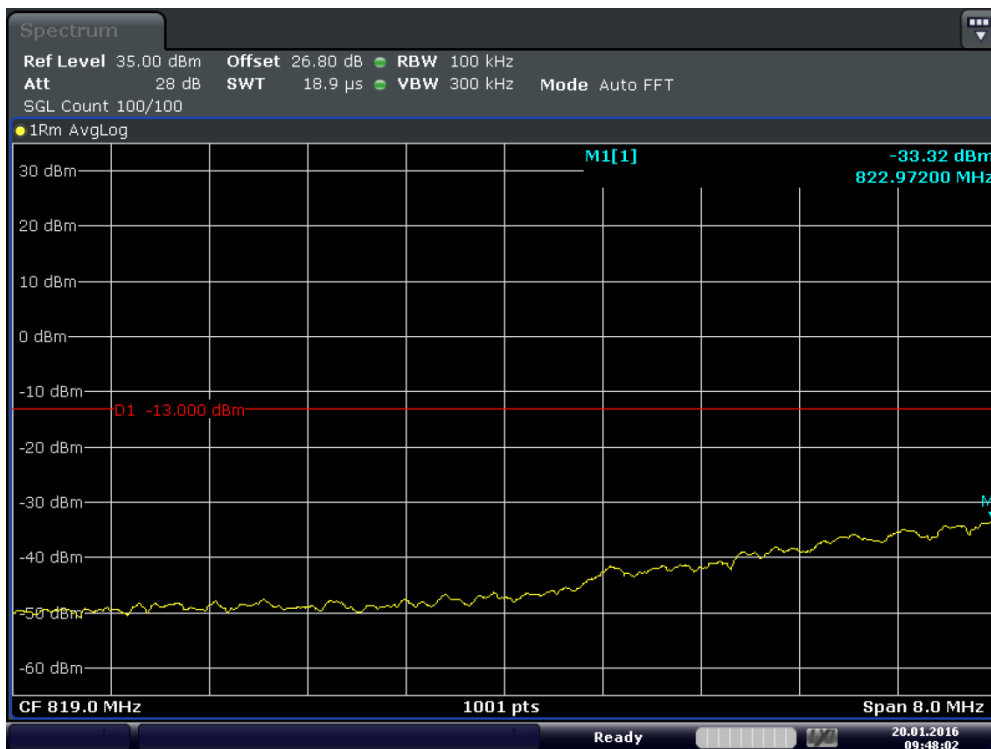
Plot 6-48. Extended Lower Band Edge Plot (Band 5 – 5.0MHz – QPSK – RB Size 25)
