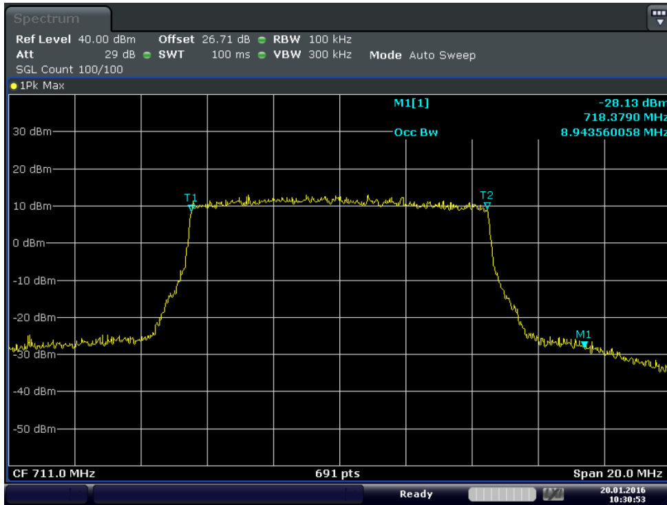
Plot 6-3. Occupied Bandwidth Plot (Band 17 – 10MHz QPSK - RB Size 50)
