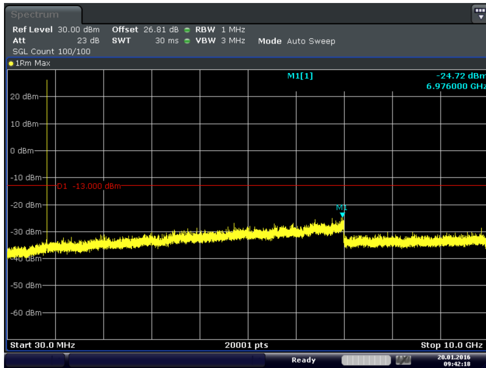
Plot 6-21. Conducted Spurious Plot (Band 5-1.4MHz-QPSK-RB Size 1-RB Offset 5- Ch.20643)
