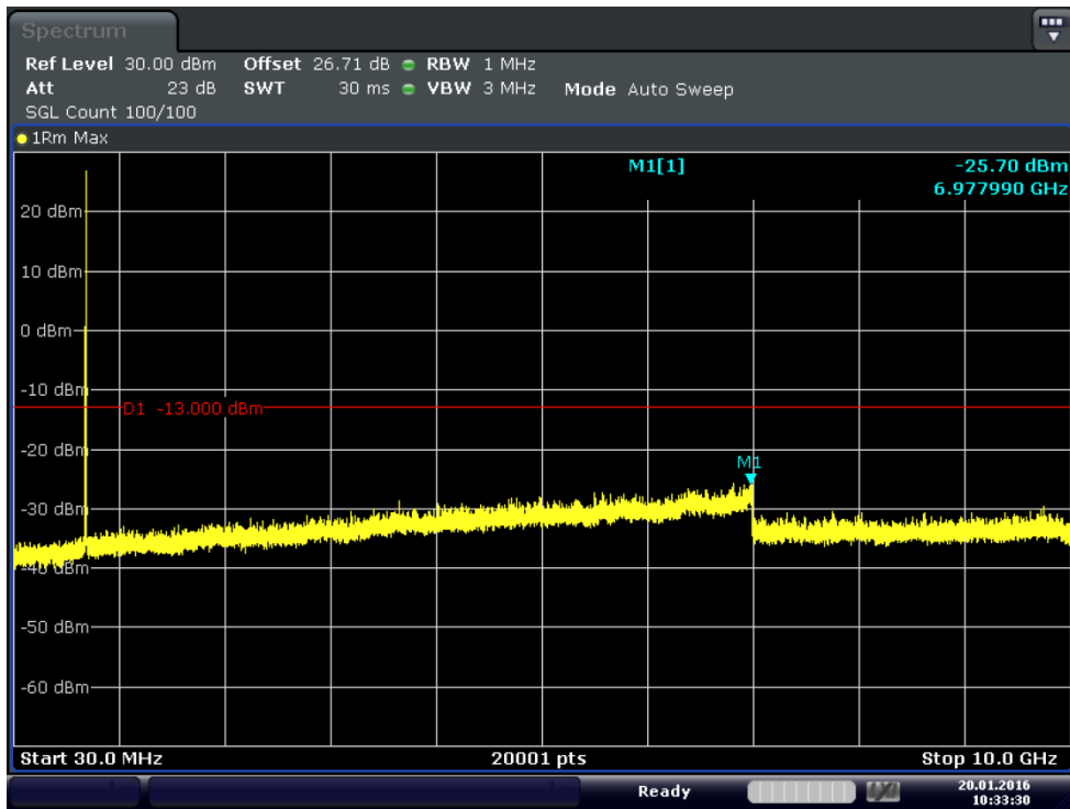
Plot 6-18. Conducted Spurious Plot (Band 17-10MHz-QPSK-RB Size 1-RB Offset 0-Ch.23800)
