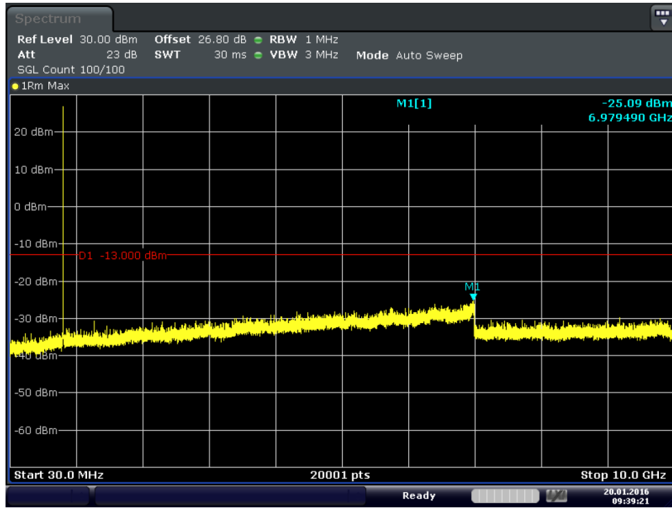
Plot 6-19. Conducted Spurious Plot (Band 5-1.4MHz-QPSK-RB Size 1-RB Offset 2-Ch.20407)
