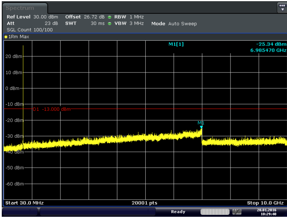
Plot 6-17. Conducted Spurious Plot (Band 17-10MHz-QPSK-RB Size 1-RB Offset 24-Ch.23790)
