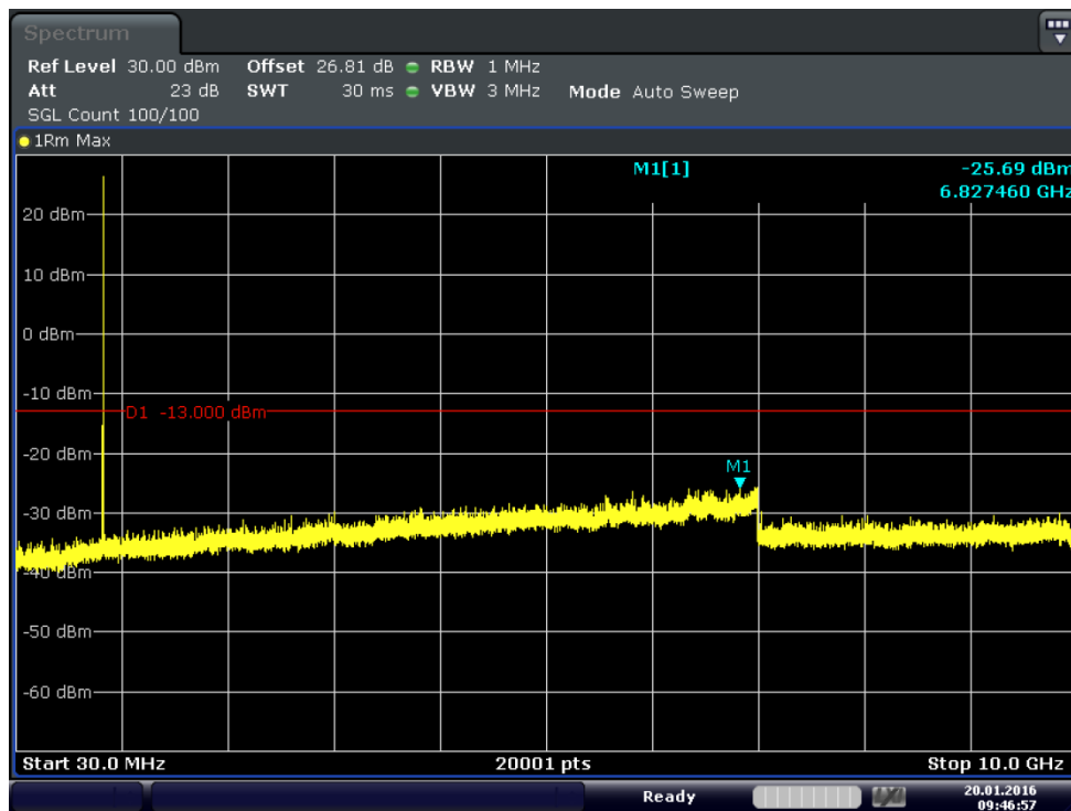
Plot 6-24. Conducted Spurious Plot (Band 5–3.0MHz–QPSK–RB Size 1–RB Offset 14– Ch.20635)
