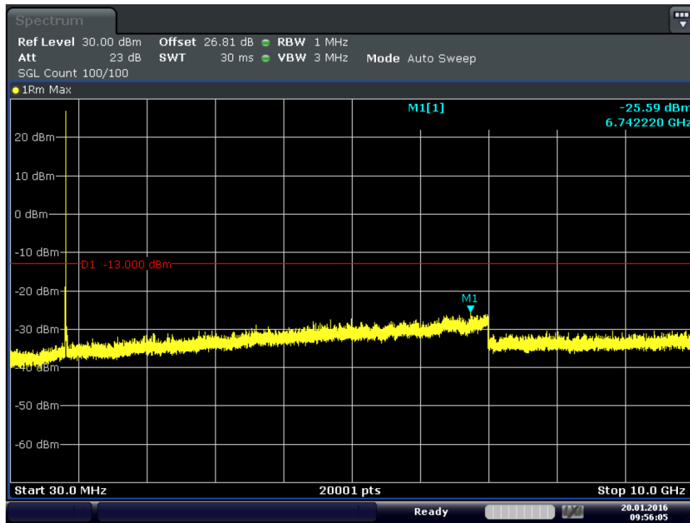
Plot 6-29. Conducted Spurious Plot (Band 5–10.0MHz–QPSK–RB Size 1–RB Offset 49– Ch.20525)
