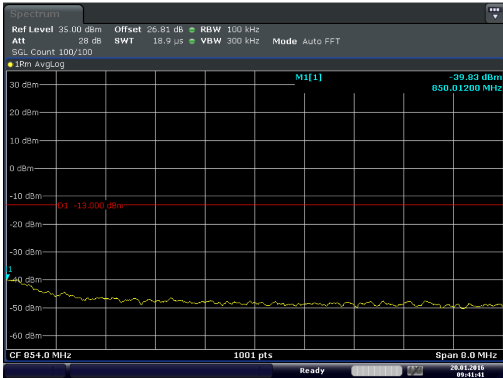
Plot 6-42. Extended Upper Band Edge Plot (Band5 – 1.4MHz – QPSK – RB Size 6)
