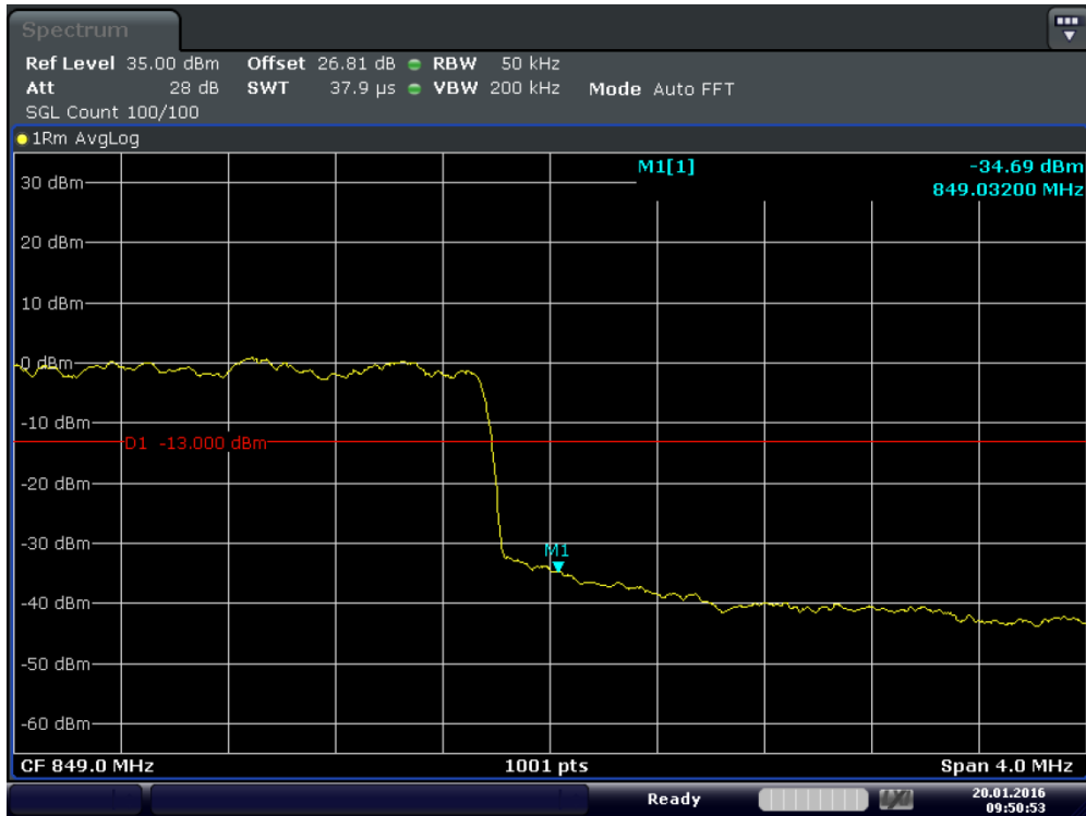
Plot 6-49. Upper Band Edge Plot (Band 5 – 5.0MHz – QPSK – RB Size 25)
