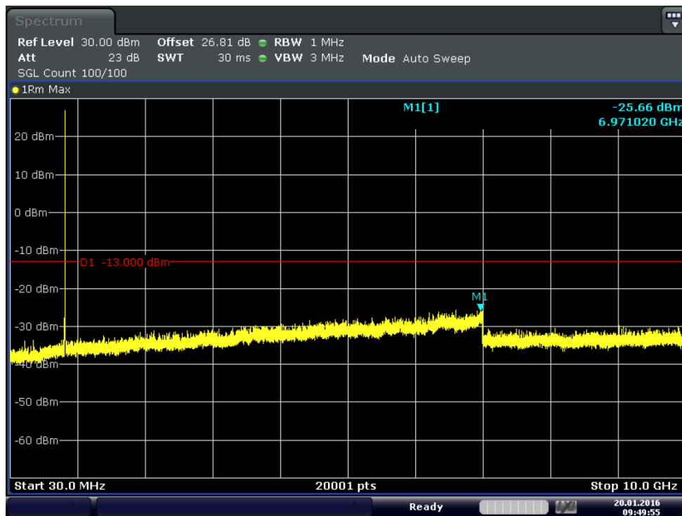
Plot 6-26. Conducted Spurious Plot (Band 5-5.0MHz-QPSK-RB Size 1-RB Offset 0- Ch.20525)
