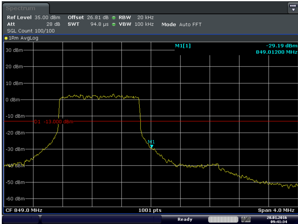
Plot 6-41. Upper Band Edge Plot (Band5 – 1.4MHz – QPSK – RB Size 6)
