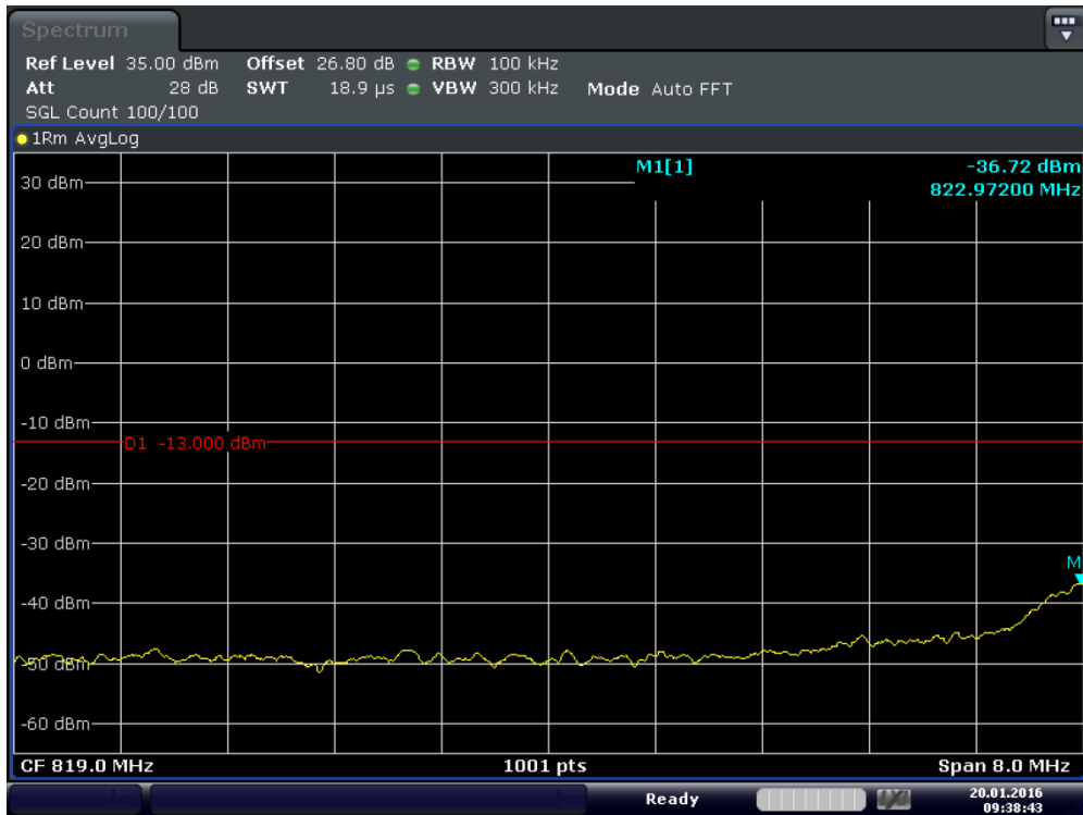
Plot 6-40. Extended Lower Band Edge Plot (Band5 – 1.4MHz – QPSK – RB Size 6)
