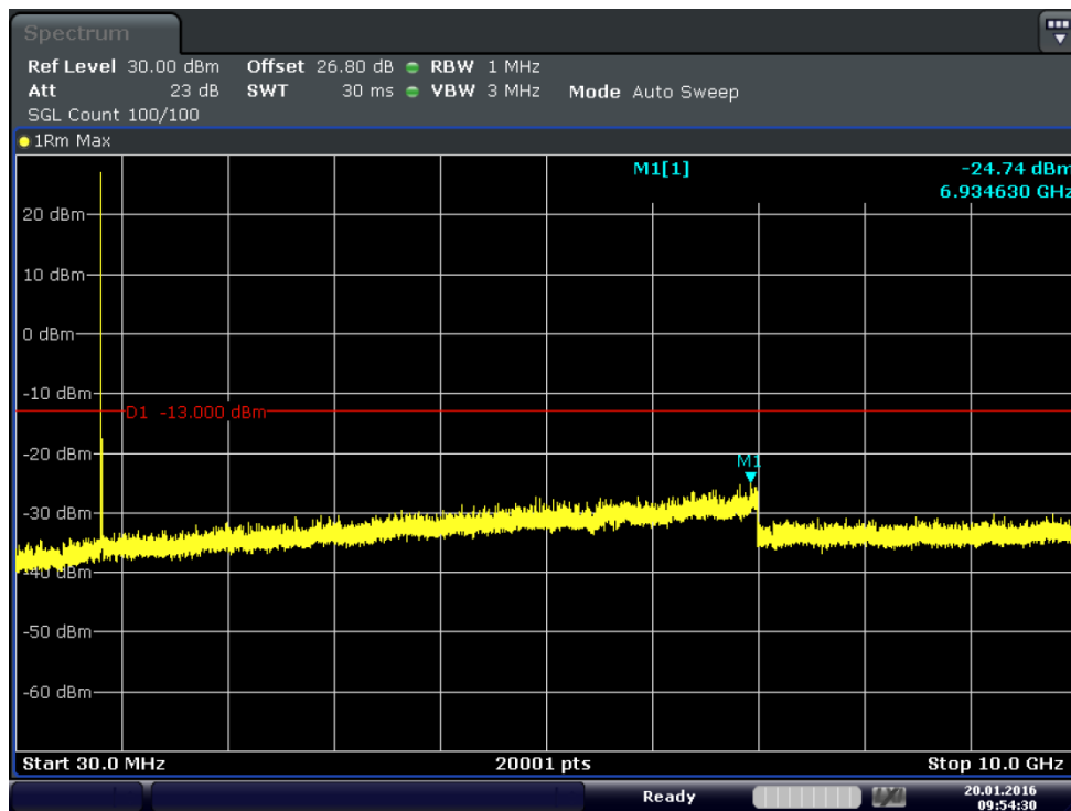
Plot 6-28. Conducted Spurious Plot (Band 5-10.0MHz-QPSK-RB Size 1-RB Offset 0- Ch.20450)
