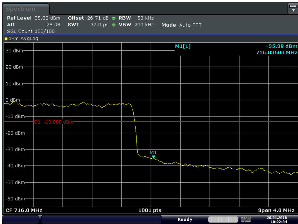
Plot 6-33. Upper Band Edge Plot (Band17 – 5MHz – QPSK – RB Size 25)
