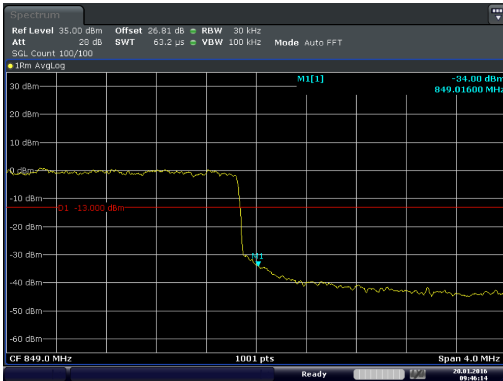
Plot 6-45. Upper Band Edge Plot (Band 5 – 3.0MHz – QPSK – RB Size 15)
