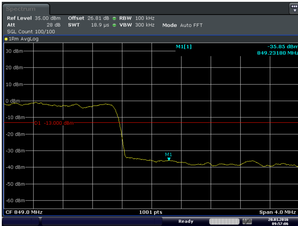
Plot 6-53. Upper Band Edge Plot (Band 5 – 10.0MHz – QPSK – RB Size 50)
